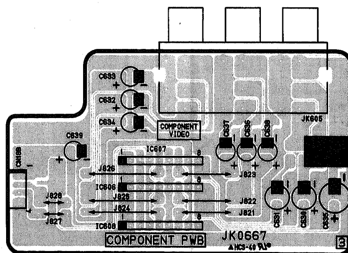
Component PWB
