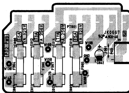
PT2 PWB
