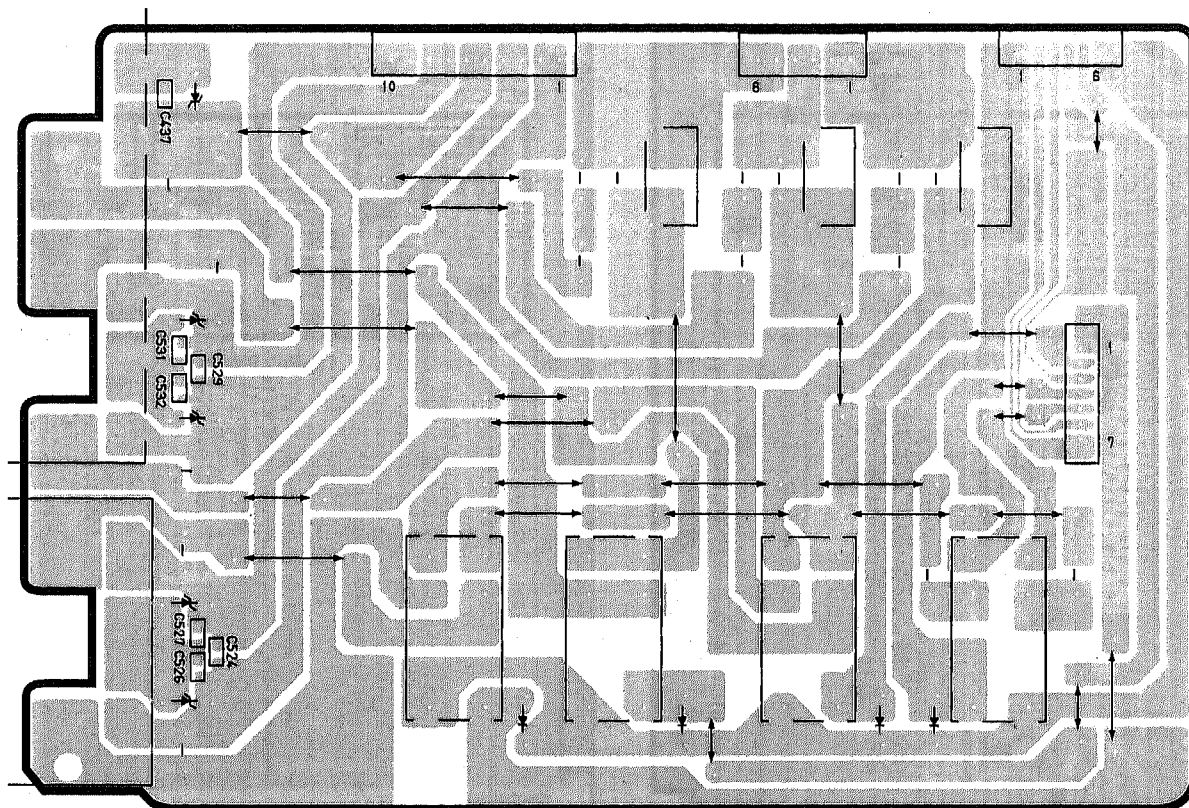
Relay PWB
