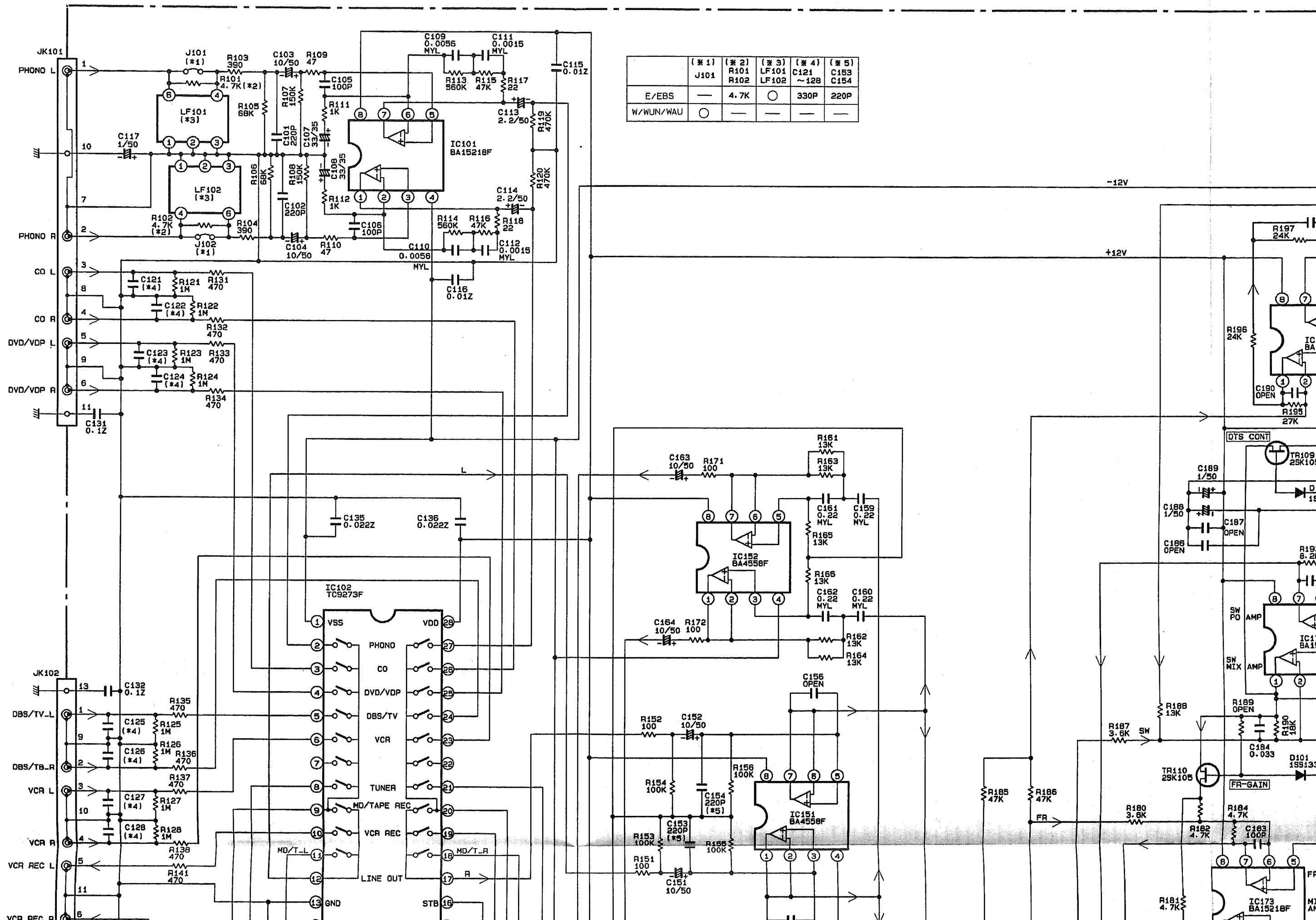
AUDIO diagram
