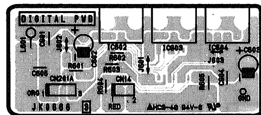
Digital PWB
