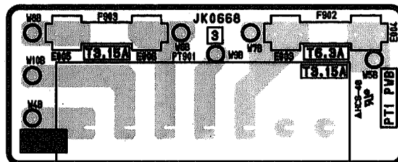
PT1 PWB
