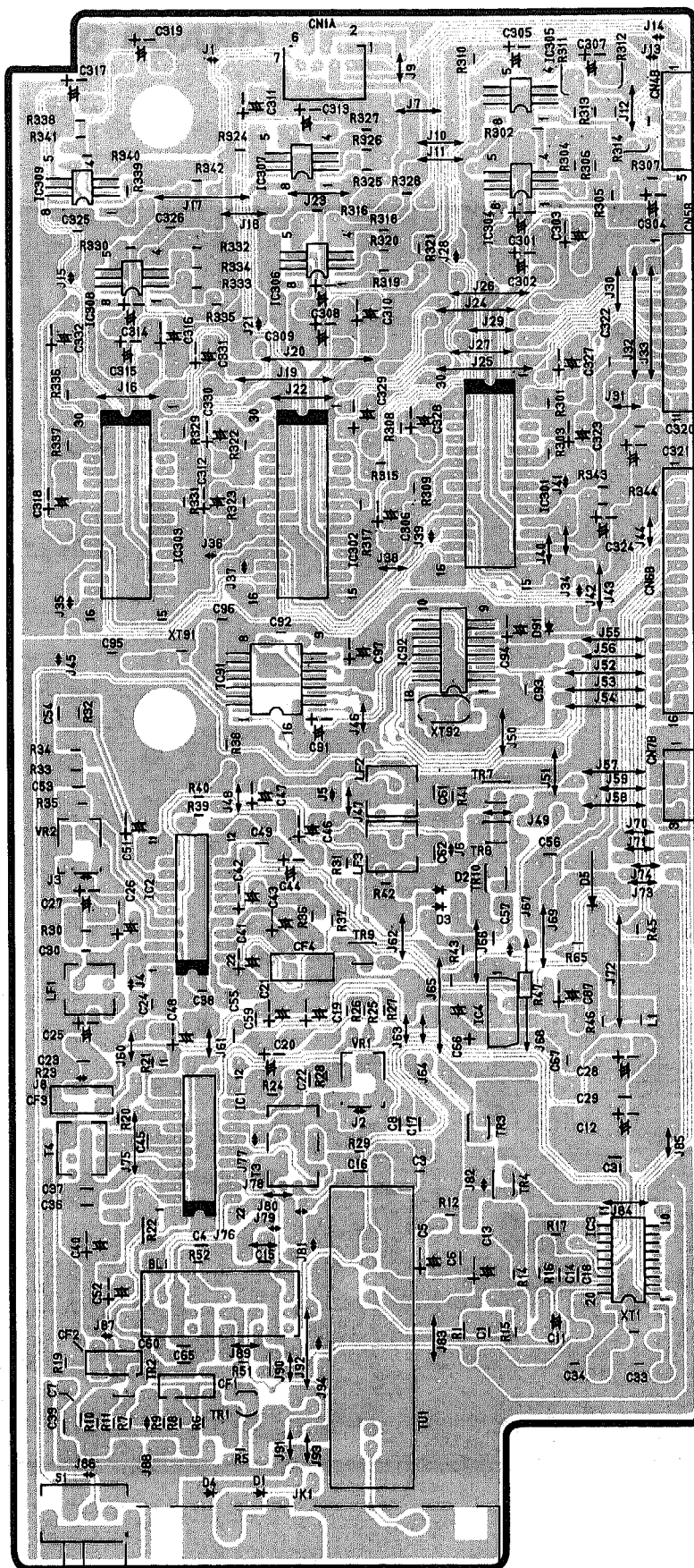
TUNER PWB
