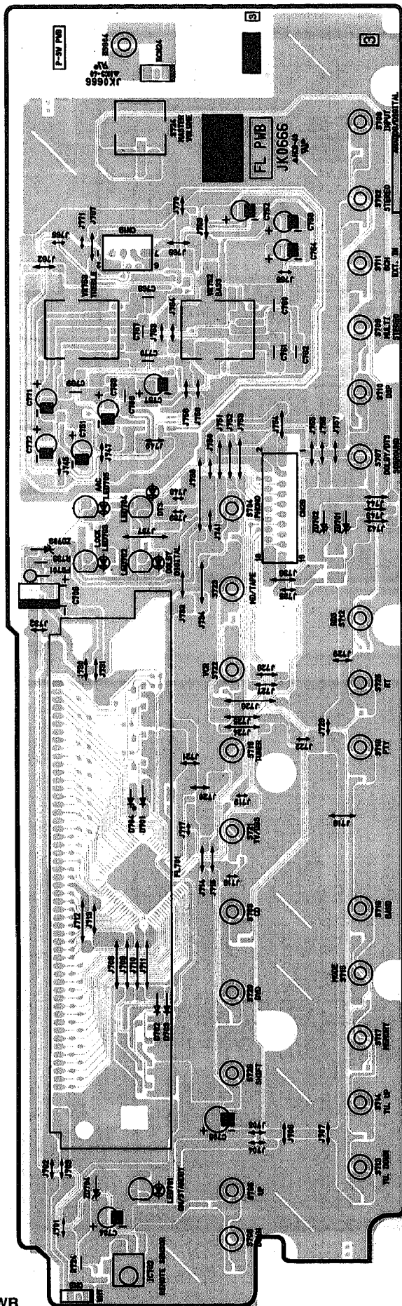
FL PWB
