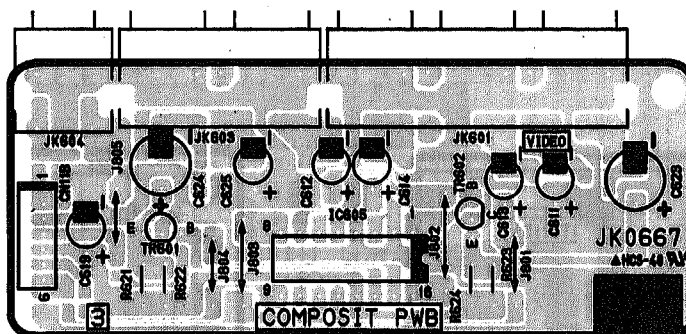
Composit PWB
