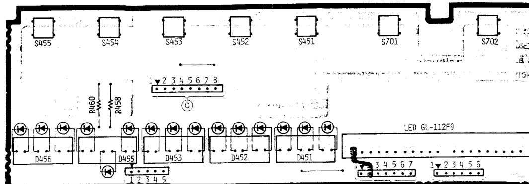
HEADPHONE P.W.B.
