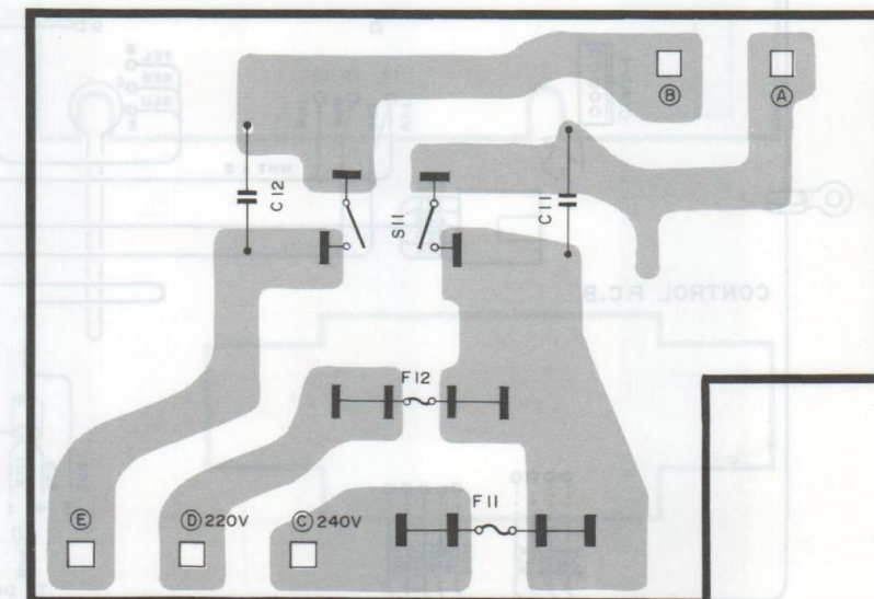
Switch P. C. Board
