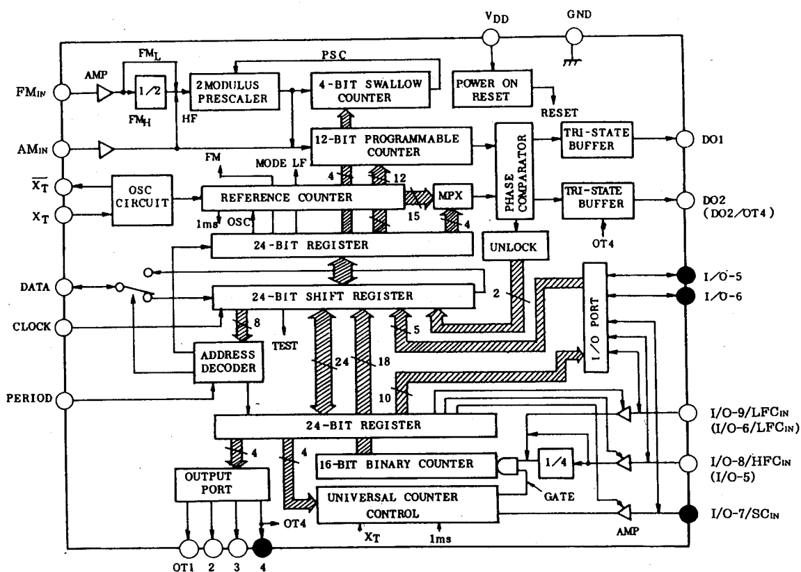
Block Diagram
