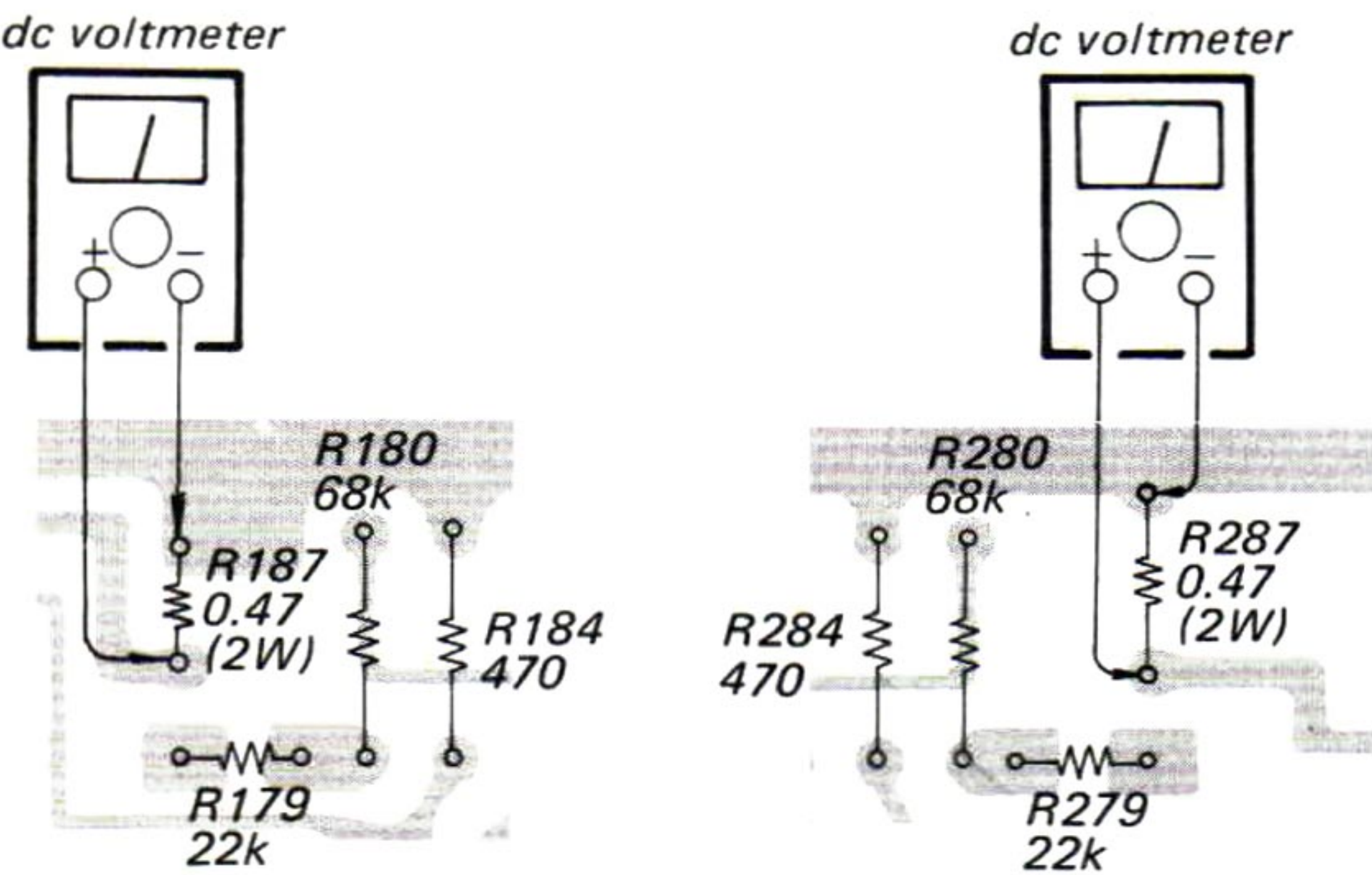
Idling current adjustment (Power amplifier circuit board)
