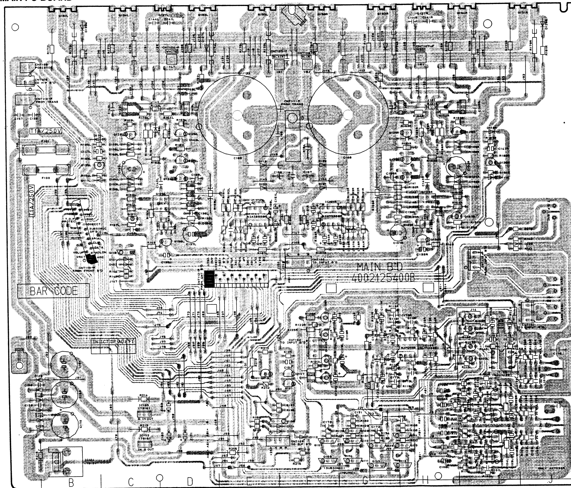
Bottom View
