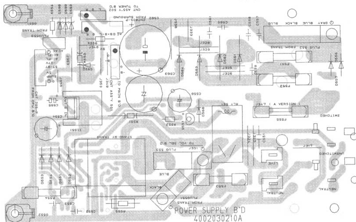
P.C.Board Power Supply
