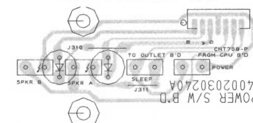
P.C.Board Power S/W
