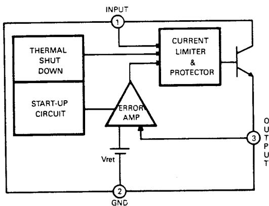
GD7815: IC201
