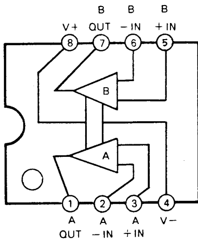
NJM4558DD: IC104 (Dual OP Amp)
