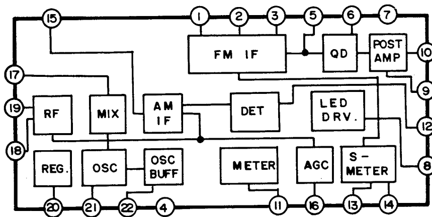
LA1265: IC101 (IF)
