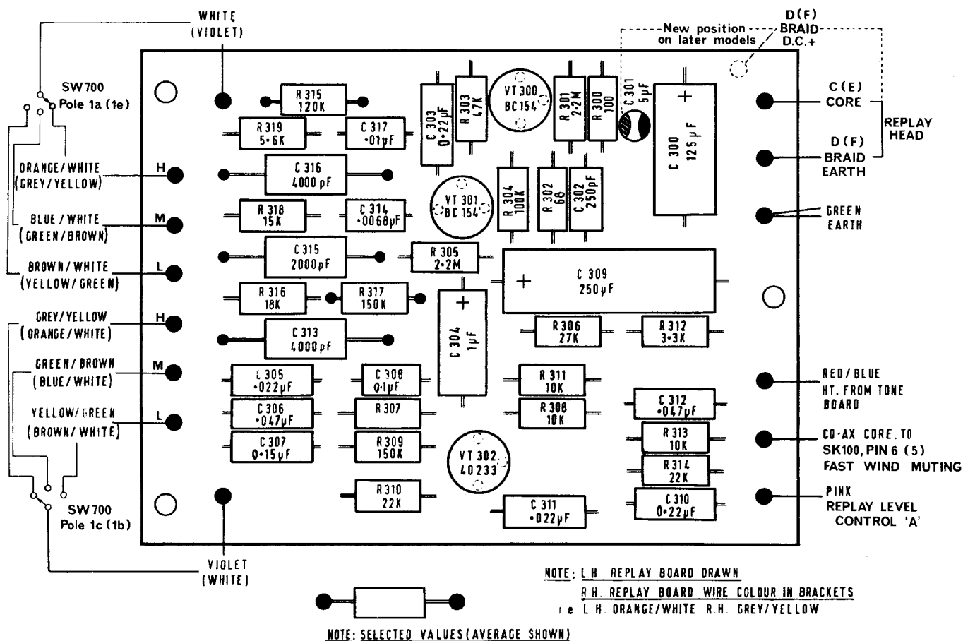
FIG. 20. REPLAY BOARD
