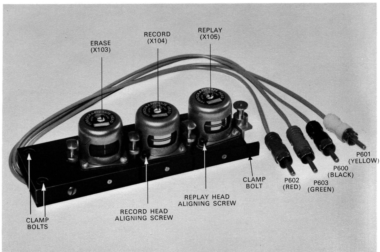
FIG. 9. HEAD ASSEMBLY
