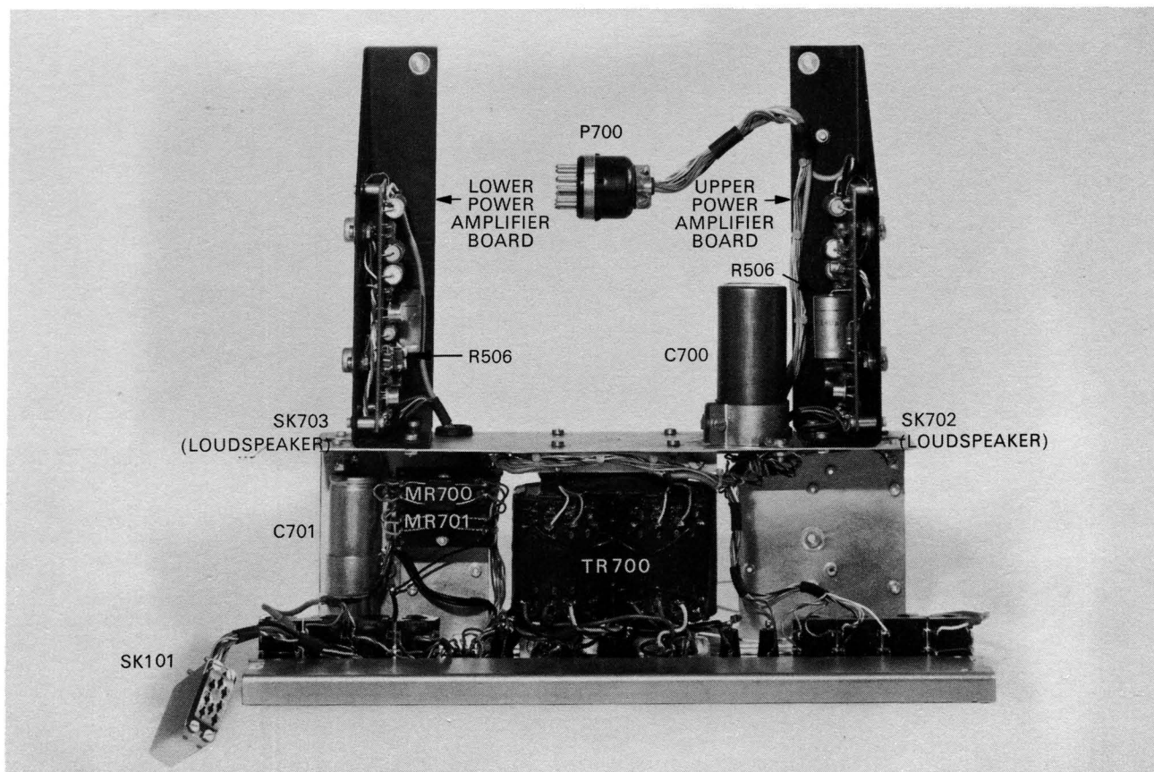
FIG. 6. POWER UNIT—STEREO
