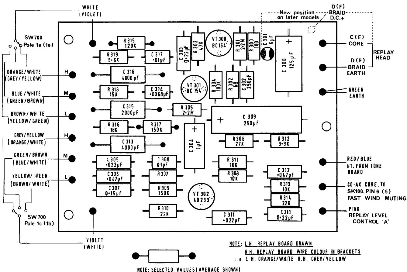
FIG. 20. REPLAY BOARD
