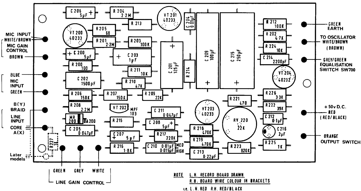
FIG. 19. RECORD BOARD
