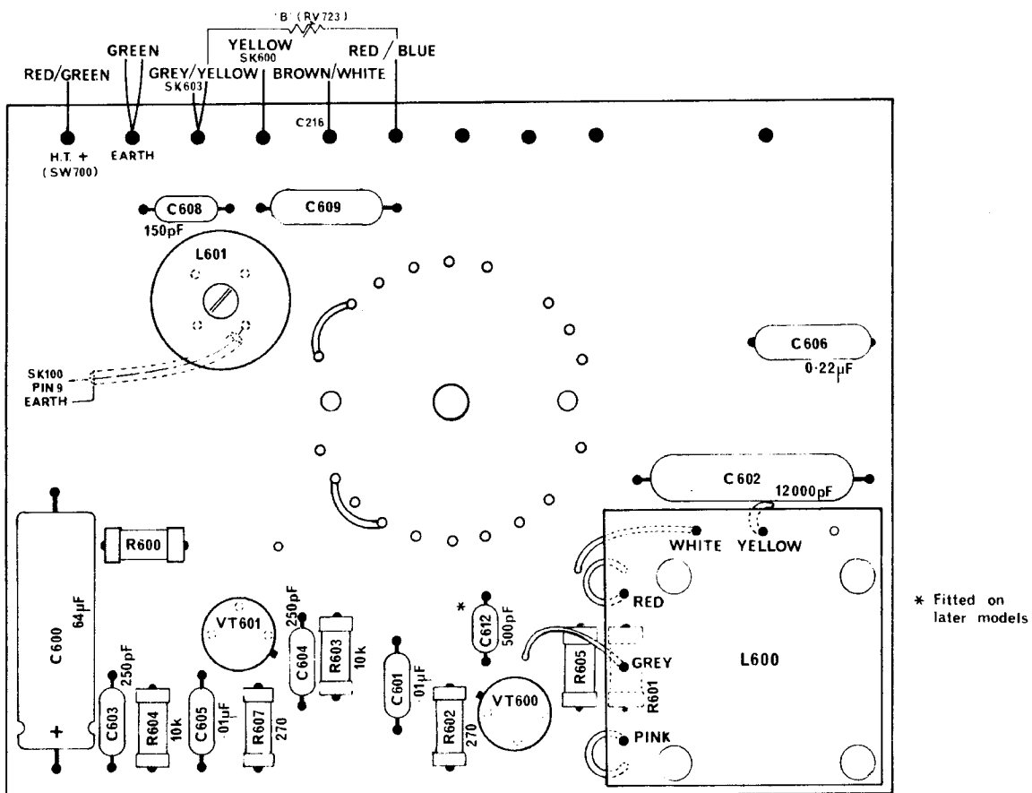
FIG. 24. OSCILLATOR BOARD—MONO
