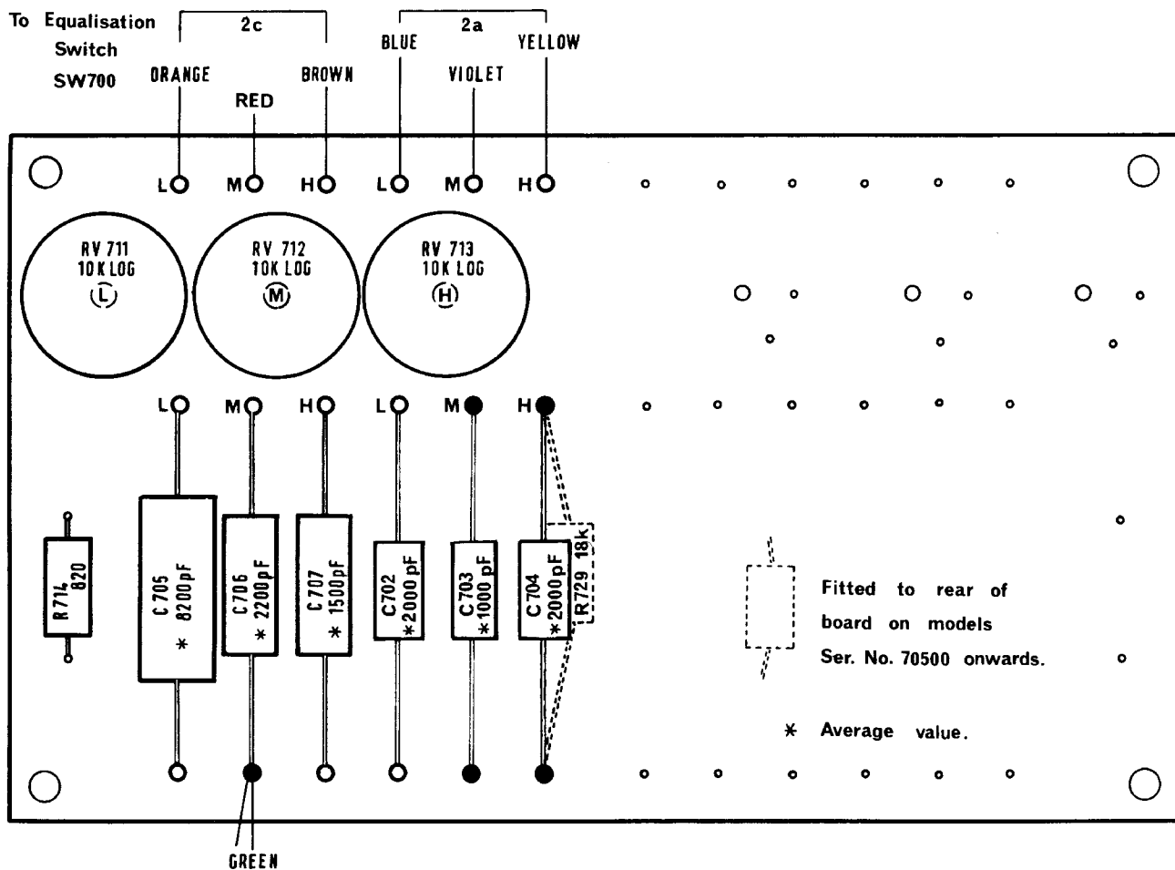
FIG. 16. EQUALISATION BOARD—MONO
