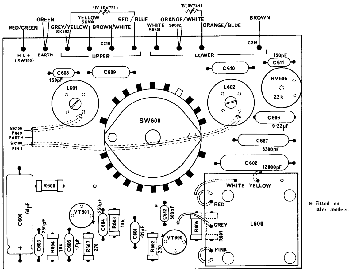
FIG. 23. OSCILLATOR BOARD—STEREO
