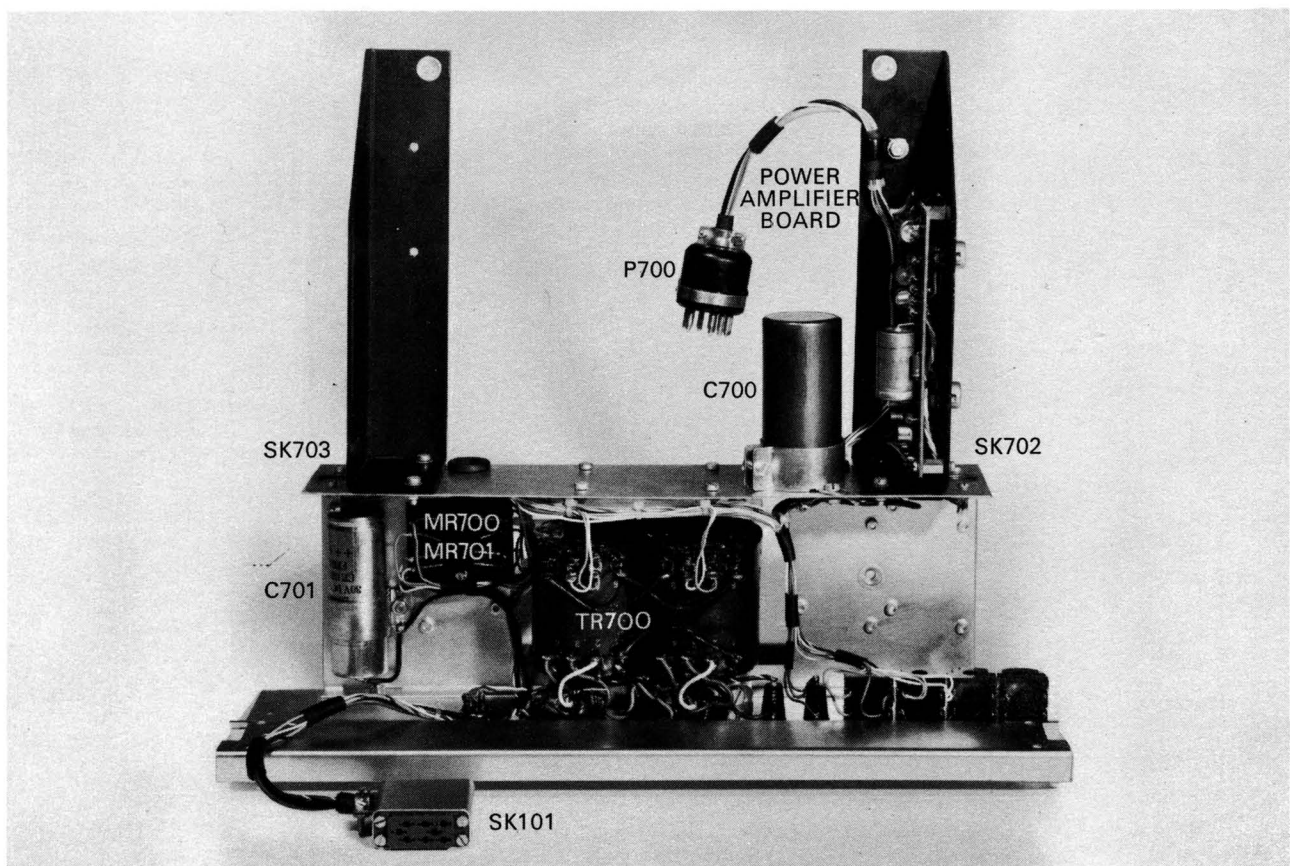
FIG. 7. POWER UNIT—MONO
