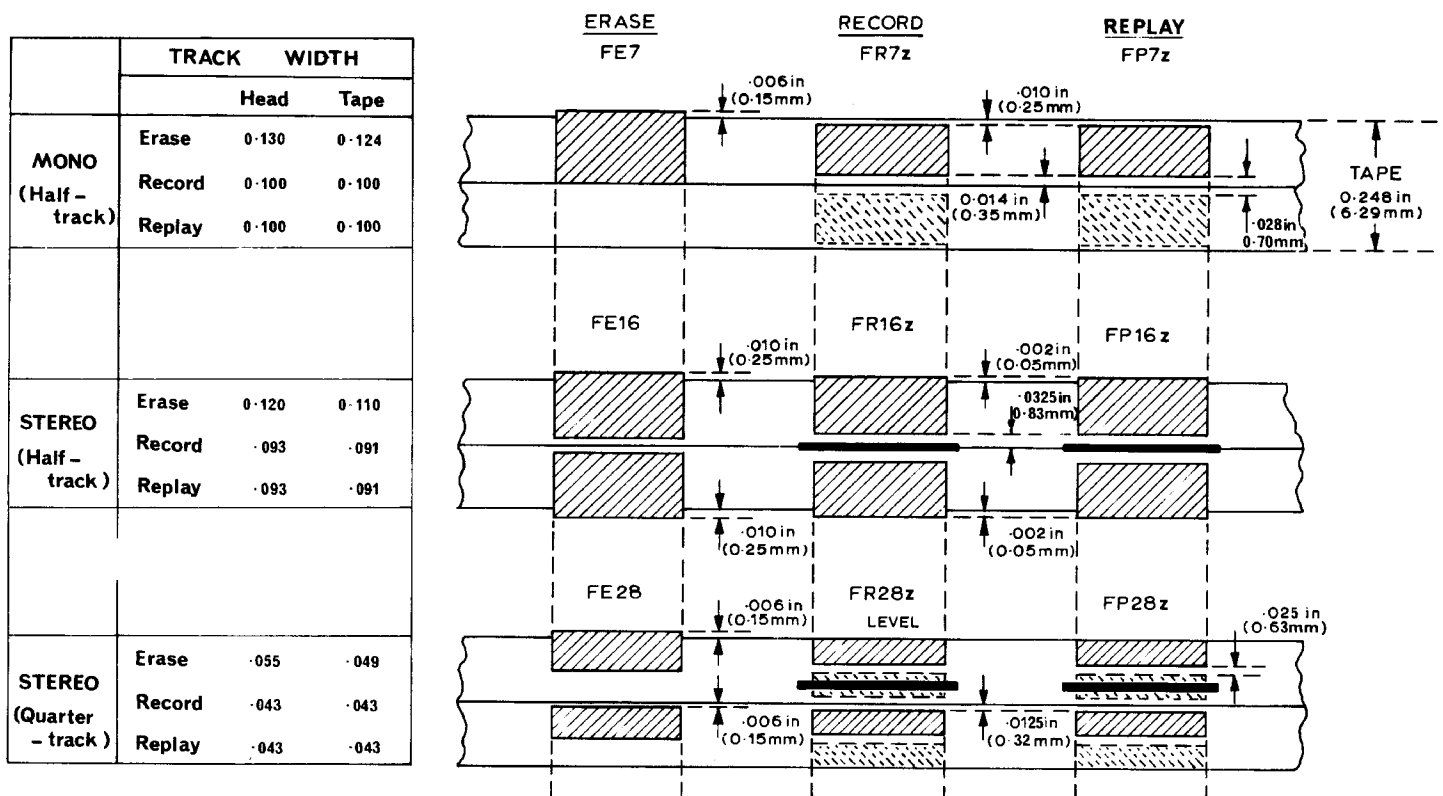
FIG. 12. HEAD ALIGNMENT
