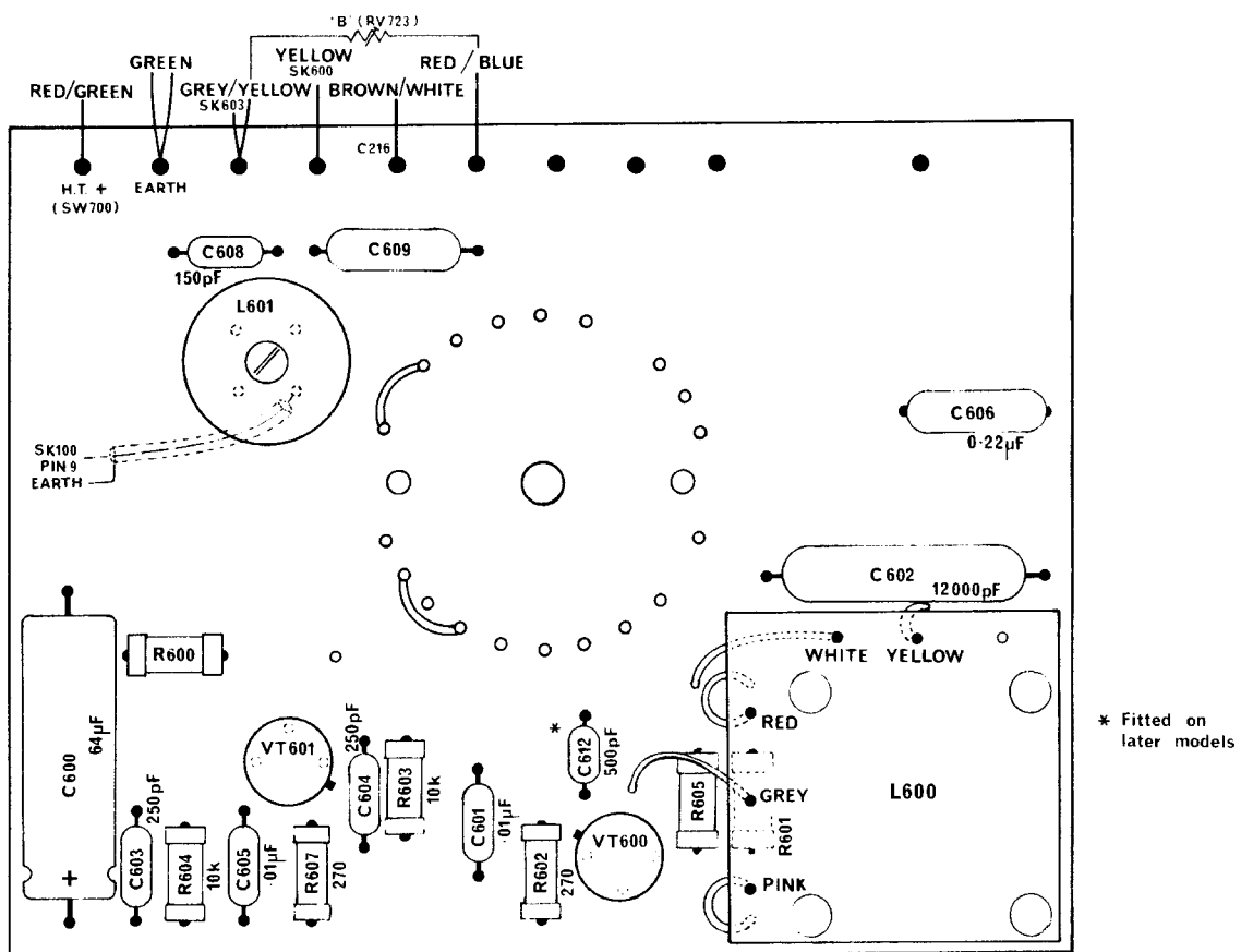
FIG. 24. OSCILLATOR BOARD—MONO
