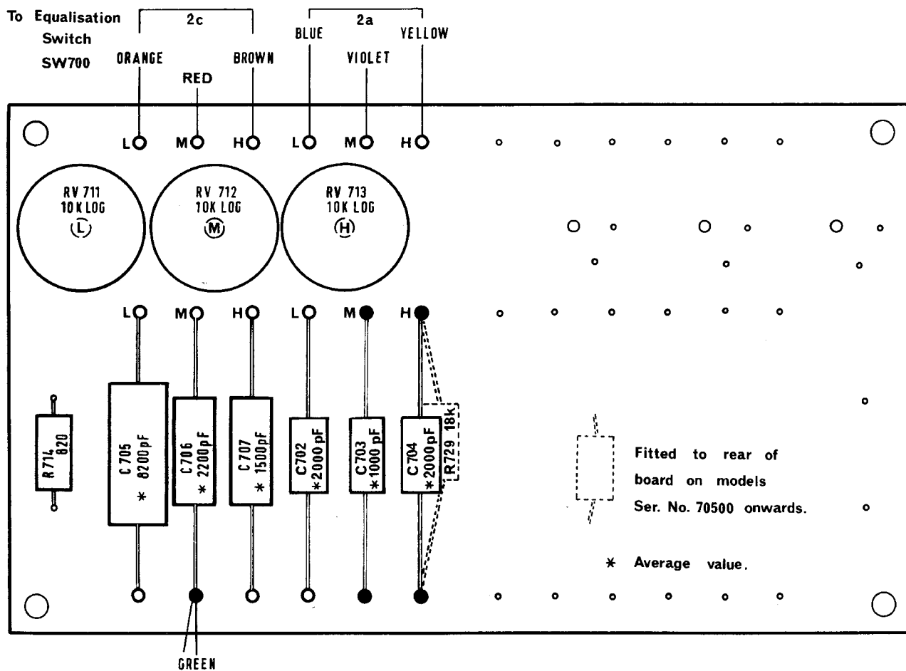
FIG. 16. EQUALISATION BOARD—MONO
