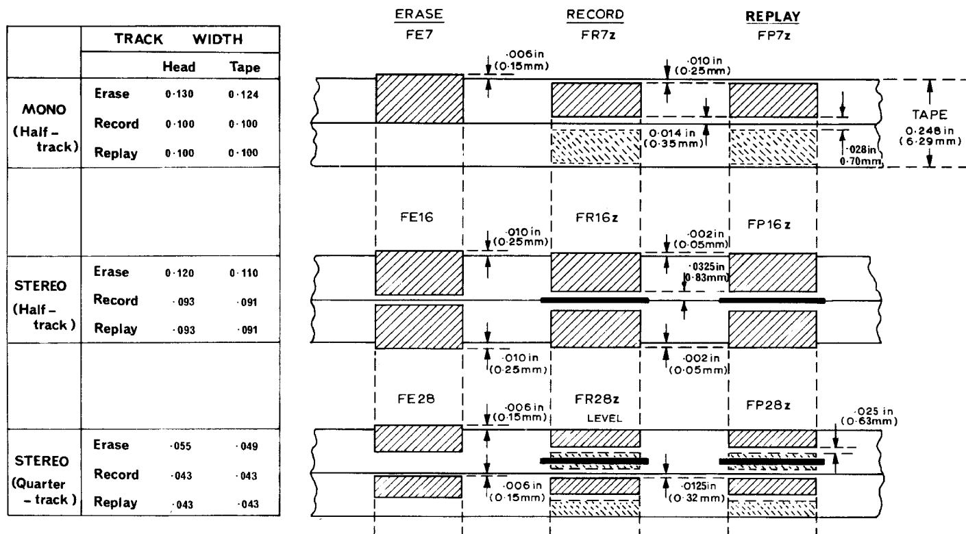
FIG. 12. HEAD ALIGNMENT
