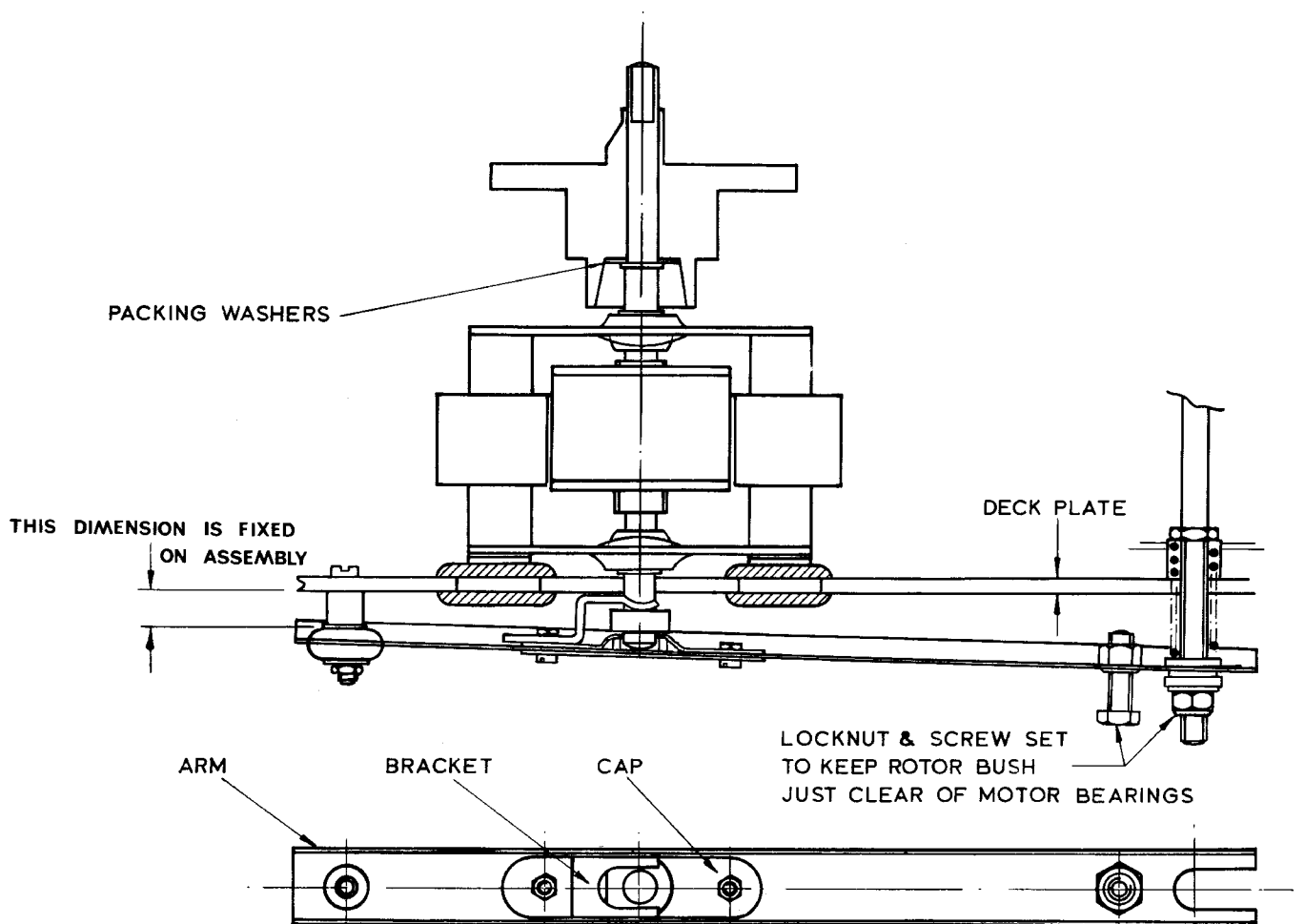
FIG. 11. REEL HEIGHT ADJUSTMENT
