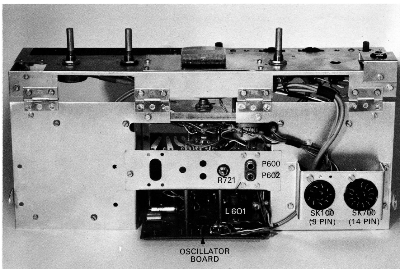
FIG. 5. AMPLIFIER—MONO, REAR VIEW
