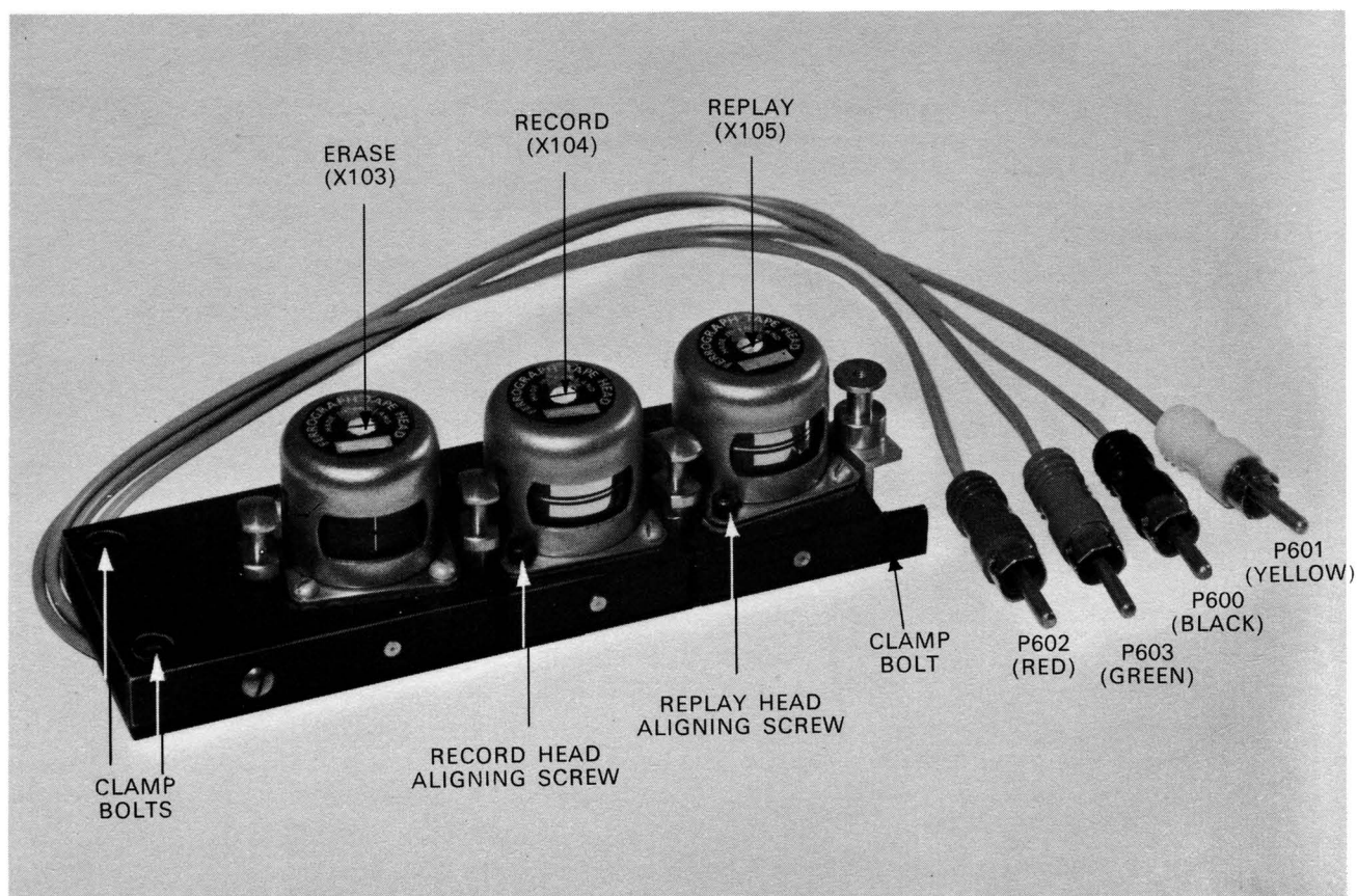
FIG. 9. HEAD ASSEMBLY
