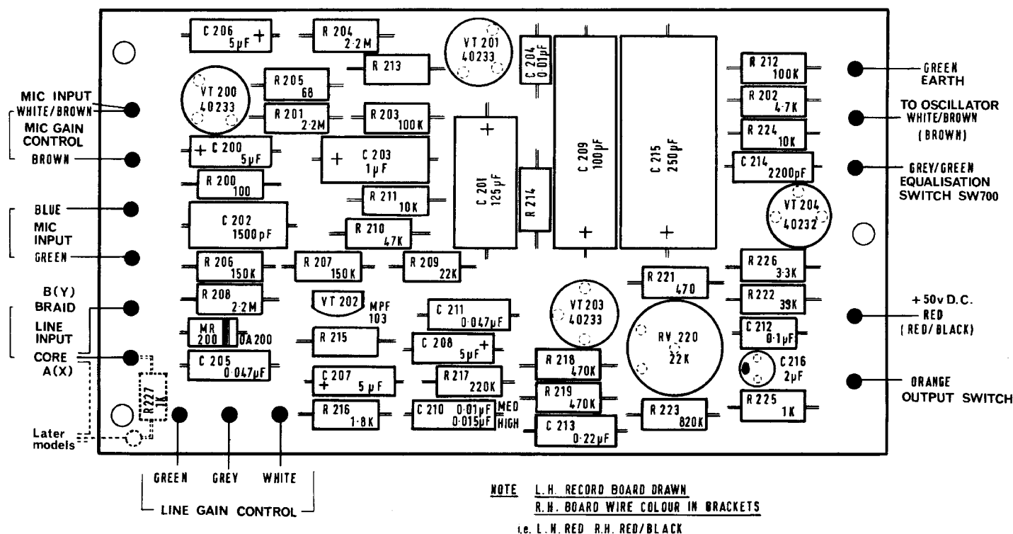
FIG. 19. RECORD BOARD
