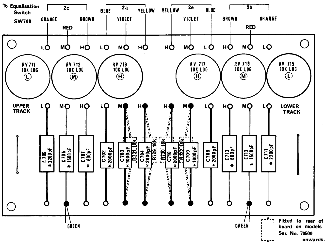
FIG. 17. EQUALISATION BOARD—STEREO, HIGH SPEED * Average value.
