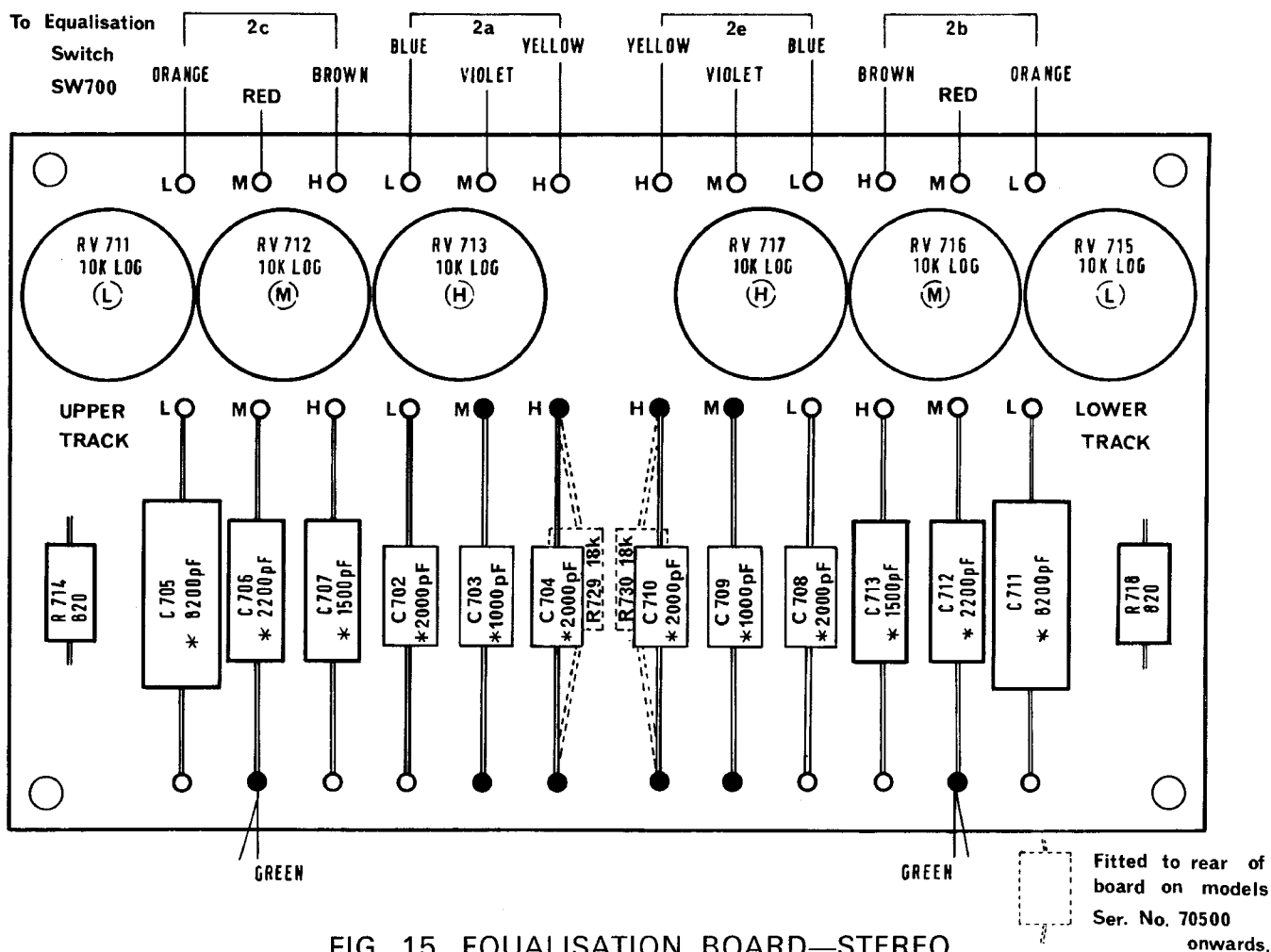
FIG. 15. EQUALISATION BOARD—STEREO
