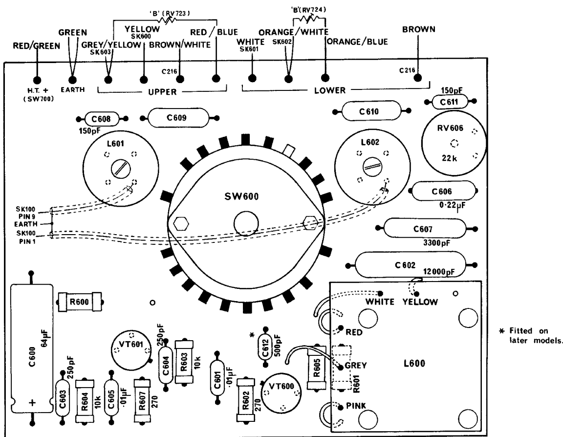
FIG. 23. OSCILLATOR BOARD—STEREO
