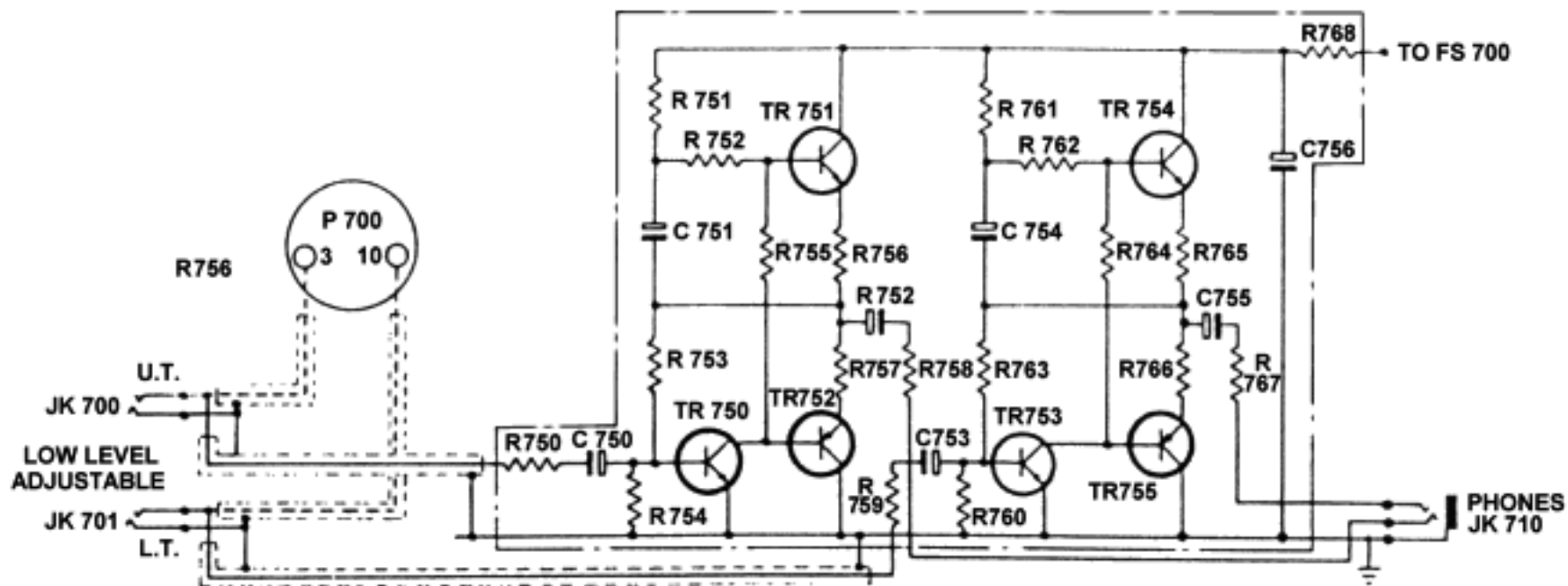
FIG. 29b PHONES AMPLIFIER—MODELS 7602 & 7604
