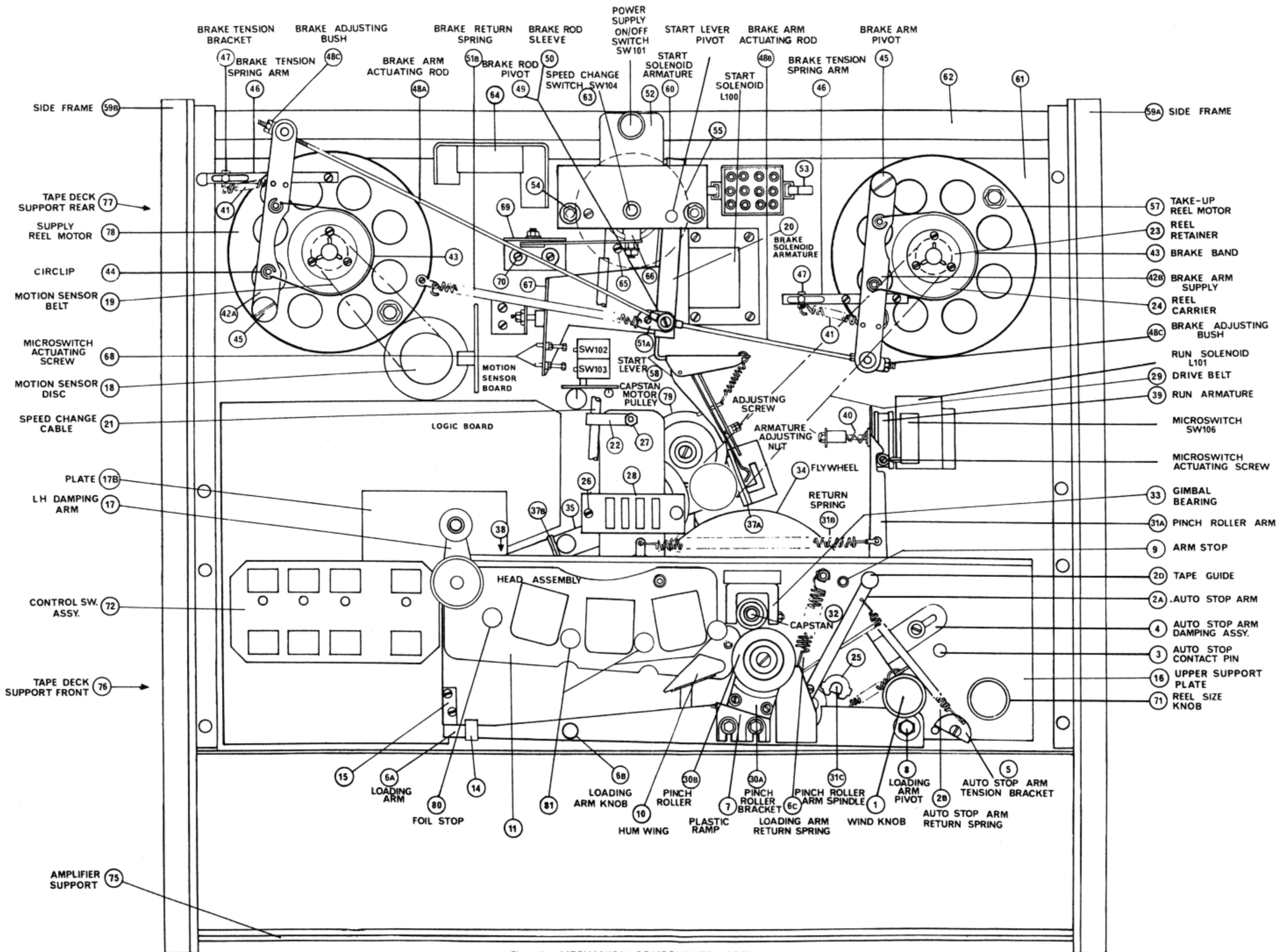
Fig. 12. MECHANICAL COMPONENTS—DECK
