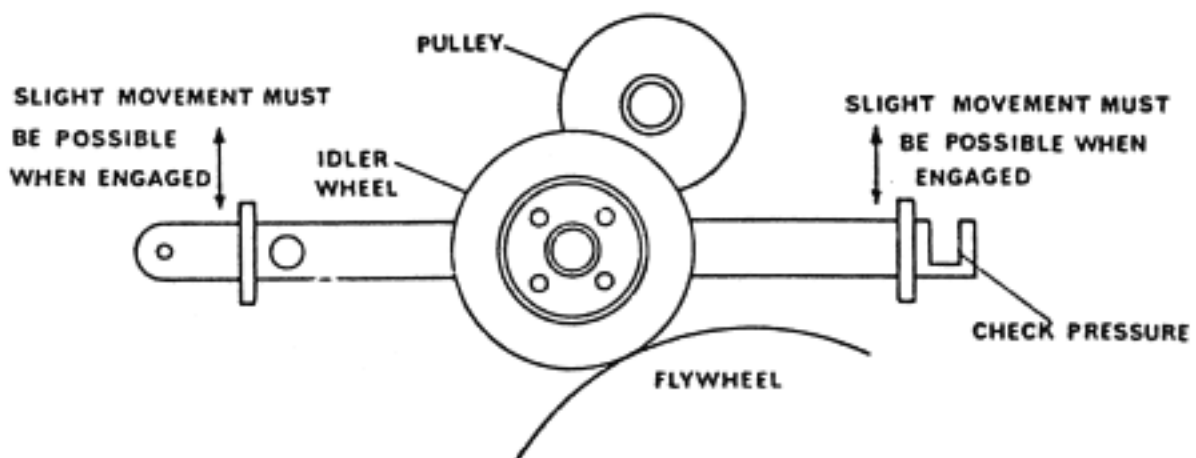
FIG. 6 IDLER AND IDLER ARM ASSEMBLY
