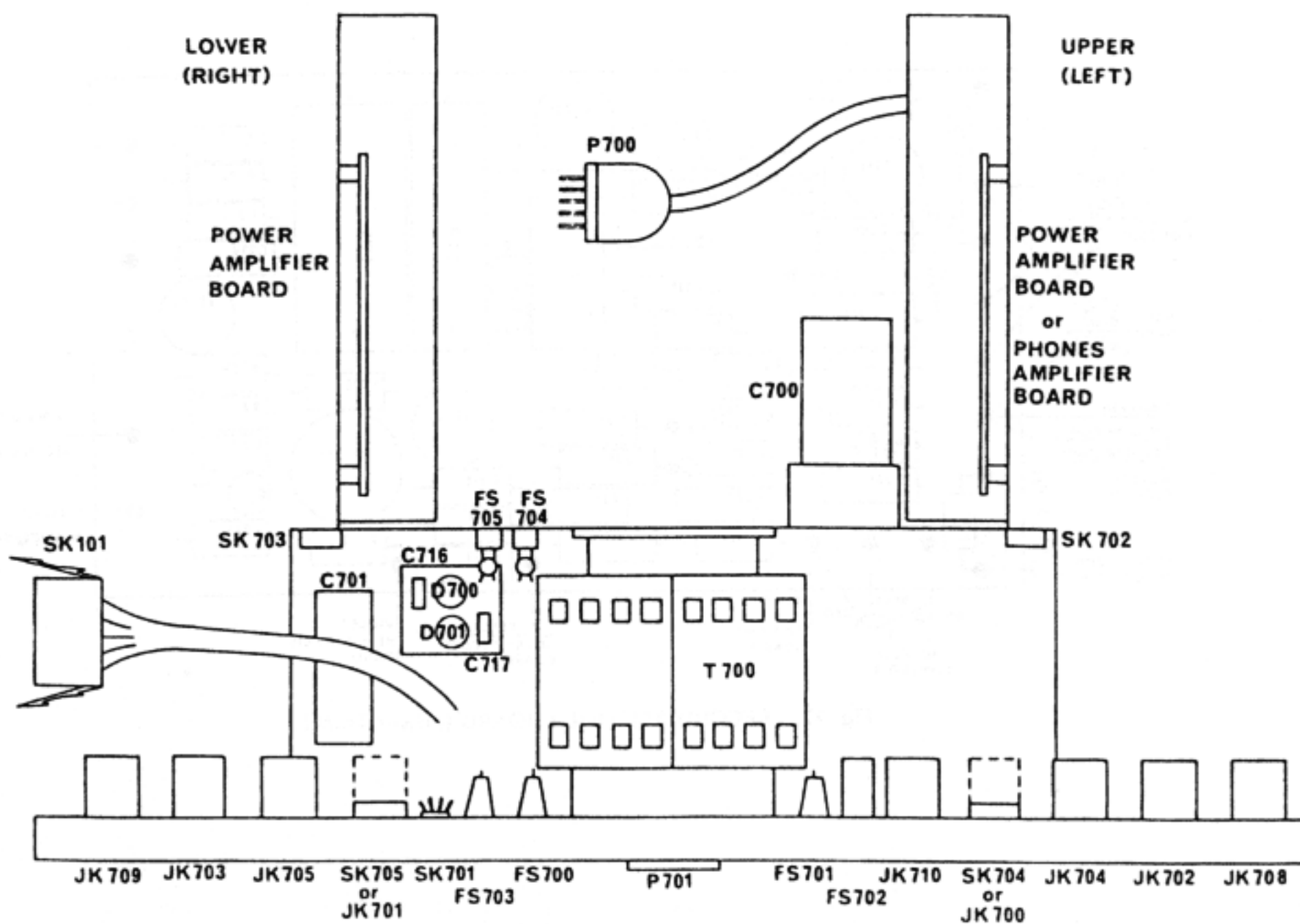
Fig. 25. POWER UNIT—REAR VIEW
