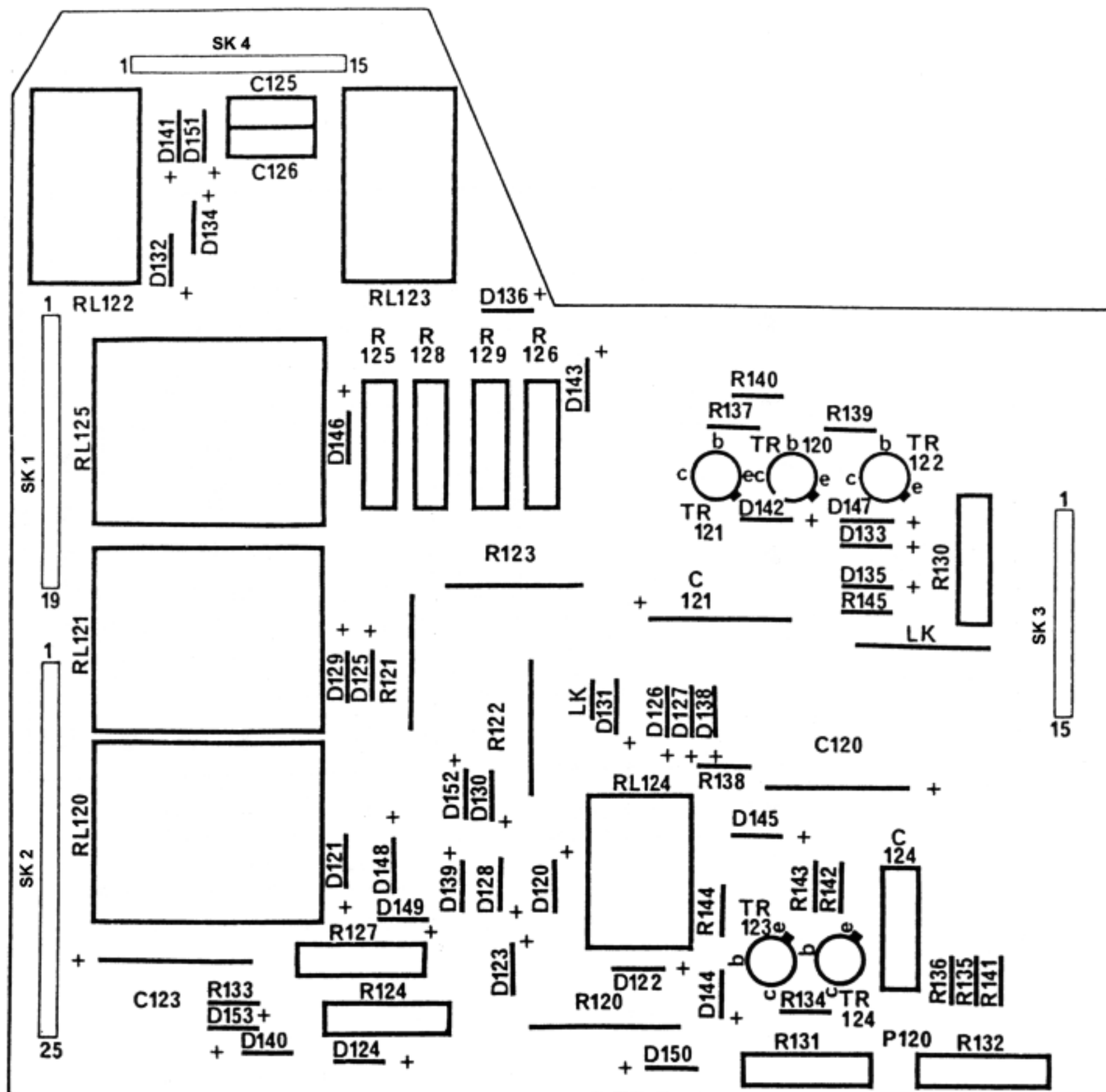
Fig. 36. LOGIC BOARD
