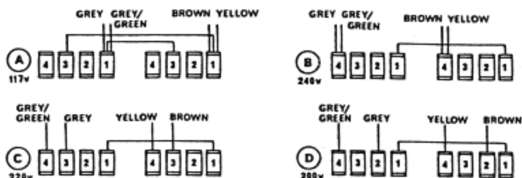
Fig. 10 Mains Supply Transformer Wiring.
