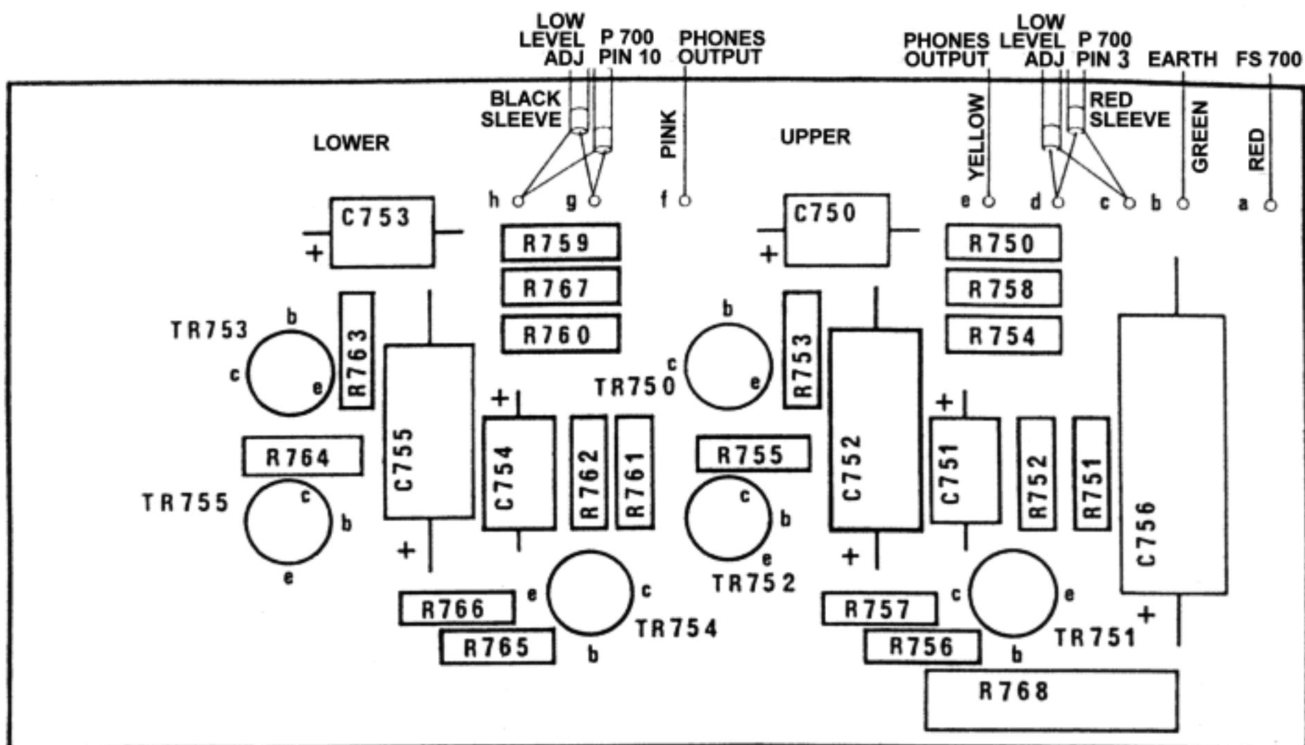
Fig. 40. PHONES BOARD
