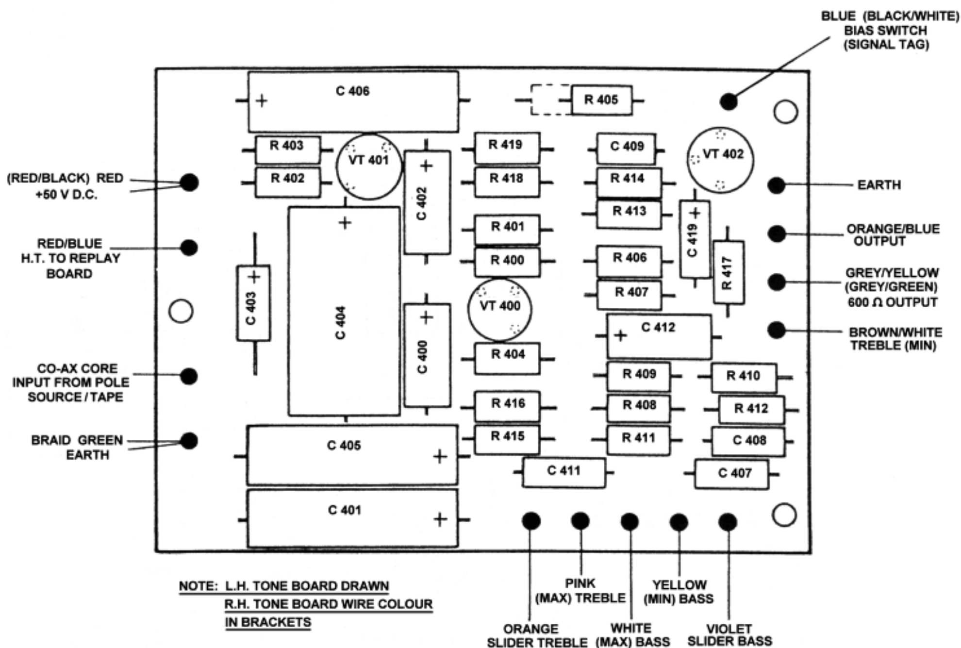
Fig. 34. TONE CONTROL BOARD
