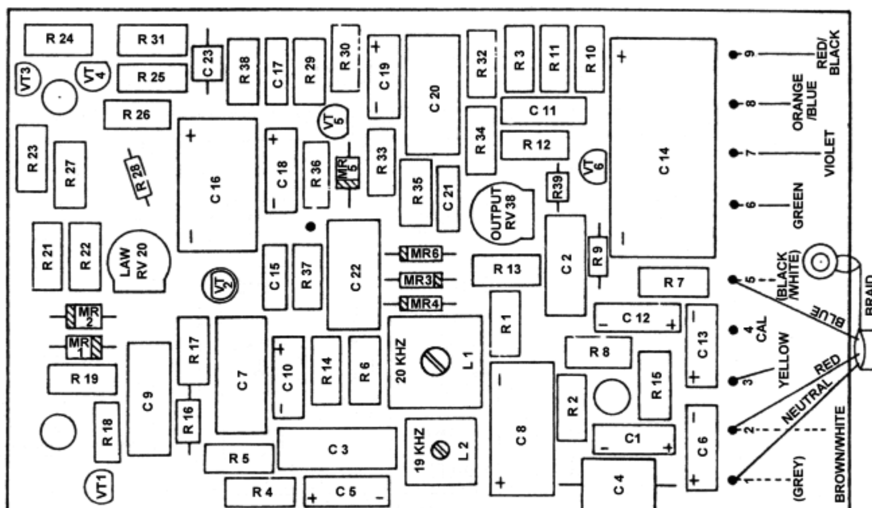
Fig. 20. DOLBY RECORD PROCESSOR BOARD
