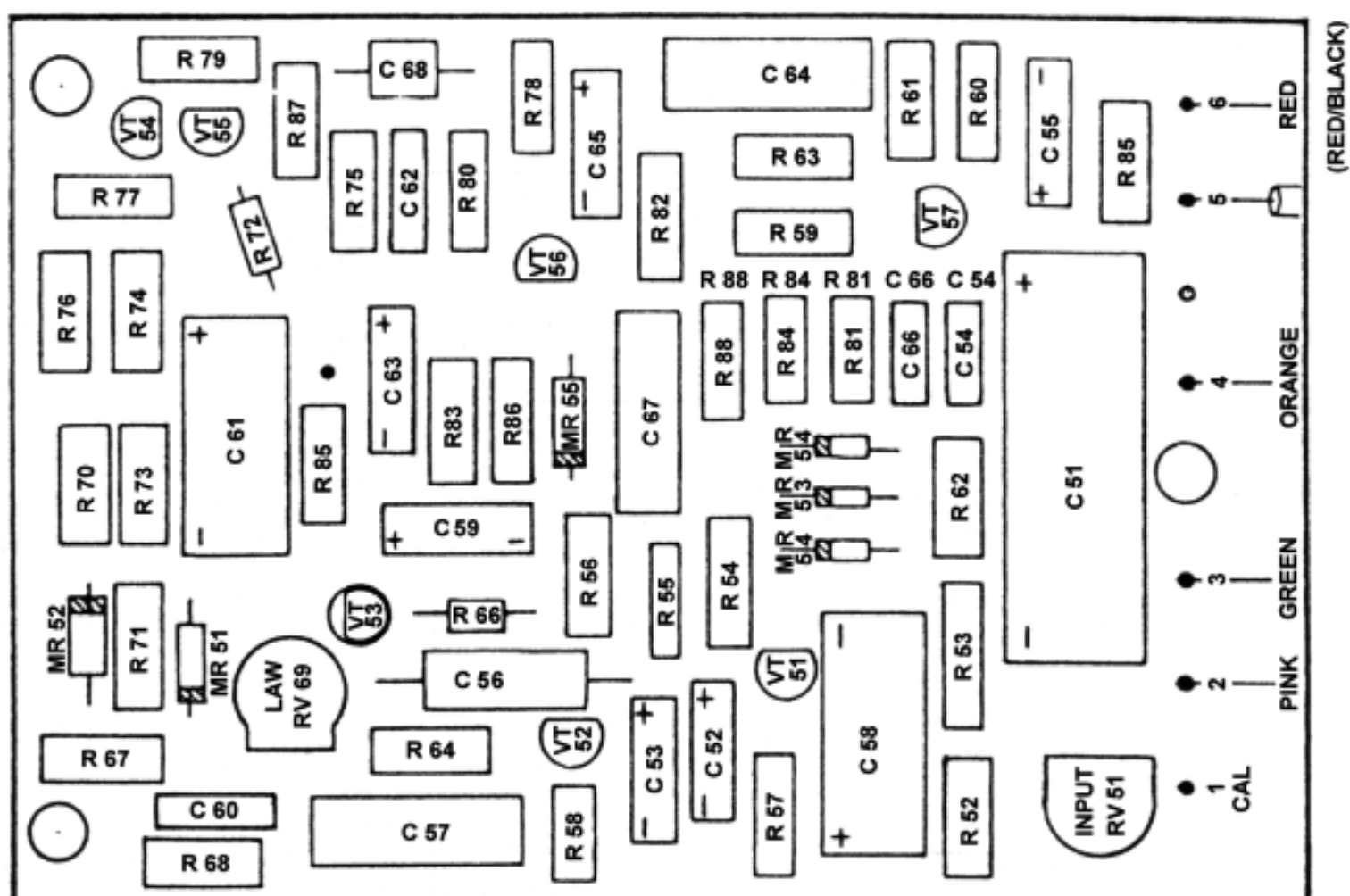
Fig. 21. DOLBY REPLAY PROCESSOR BOARD
