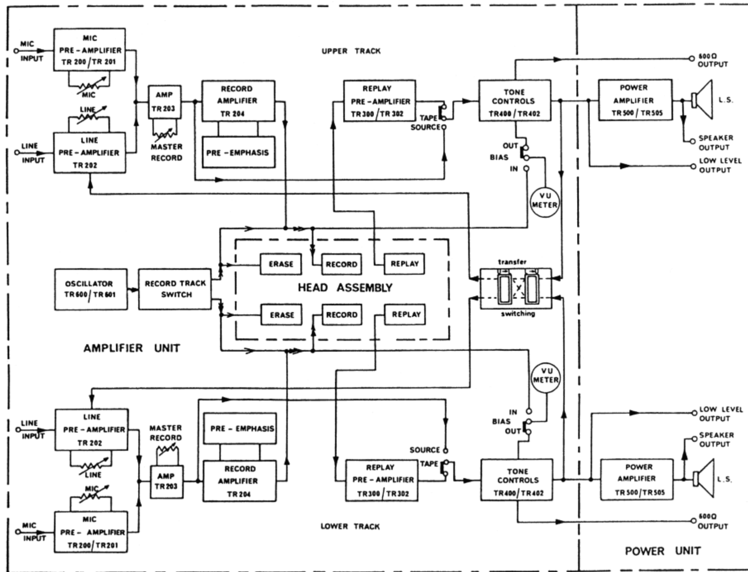
Fig. 38. BLOCK DIAGRAM—STANDARD MODELS
