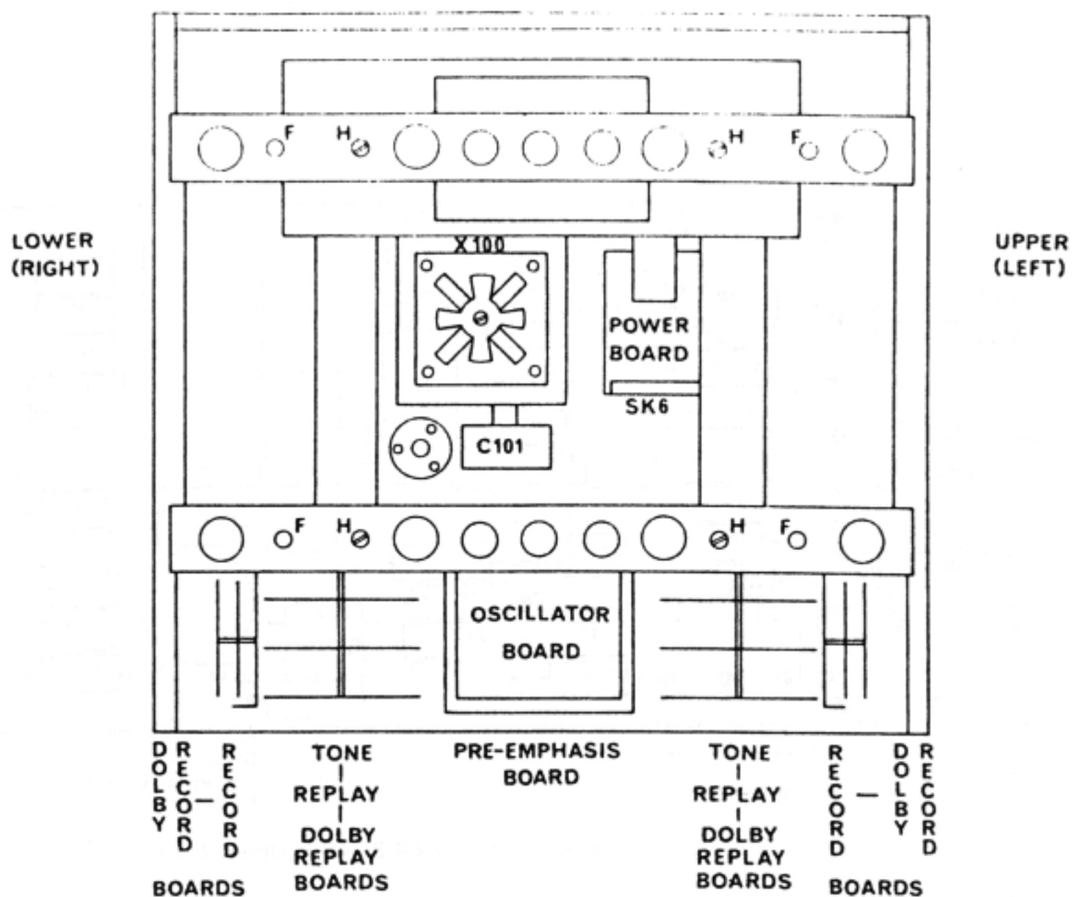
Fig. 24. RECORDER—REAR VIEW
