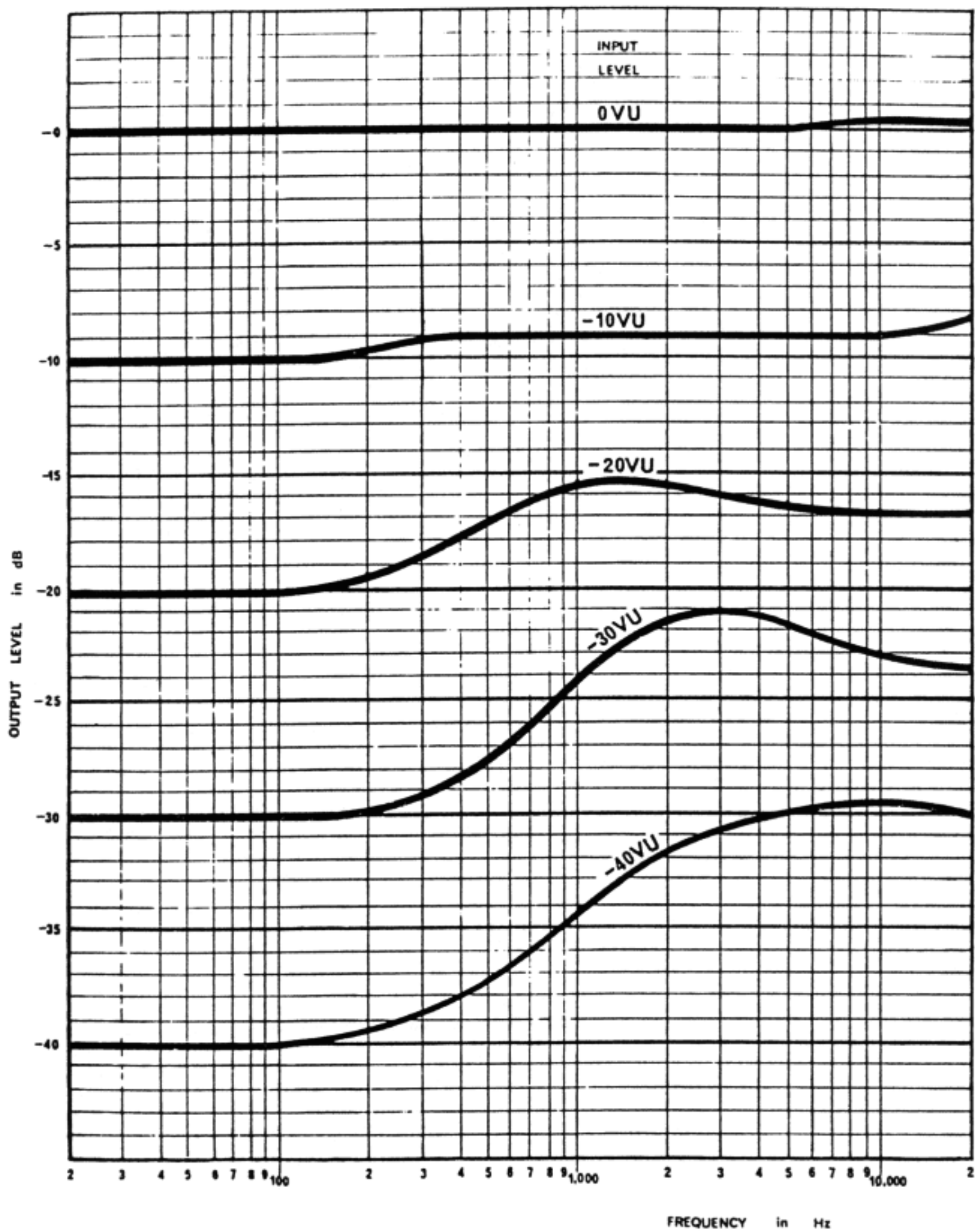
Fig. 16. RECORD PROCESSOR CHARACTERISTICS
