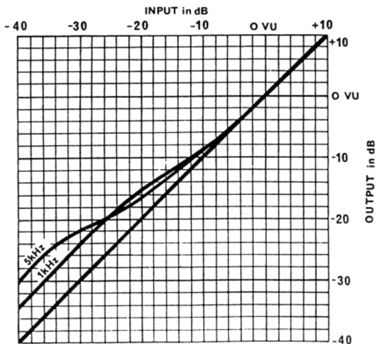
Fig. 18. RECORD TRANSFER CHARACTERISTICS—1kHz AND 5kHz
