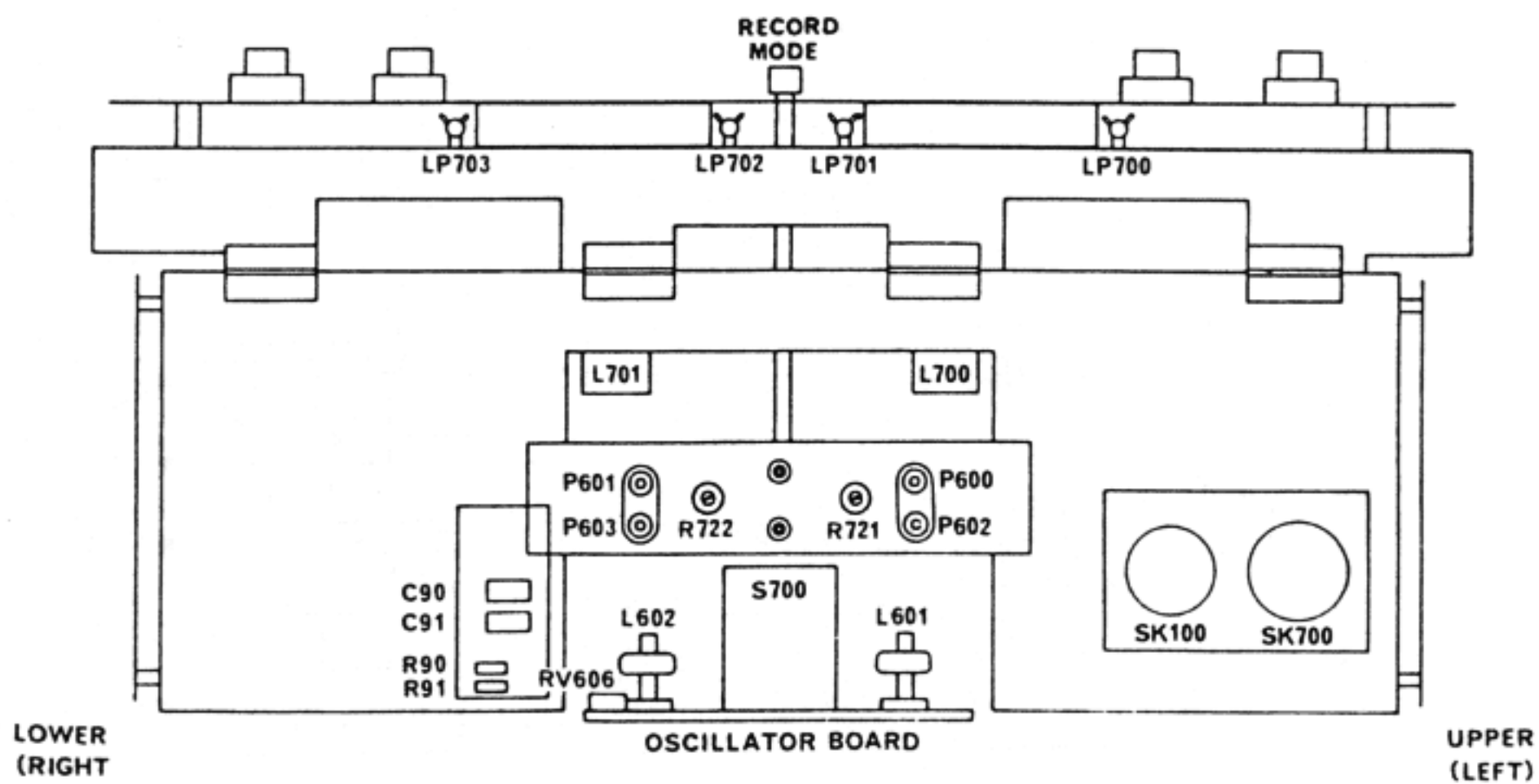
Fig. 23. AMPLIFIER—REAR VIEW
