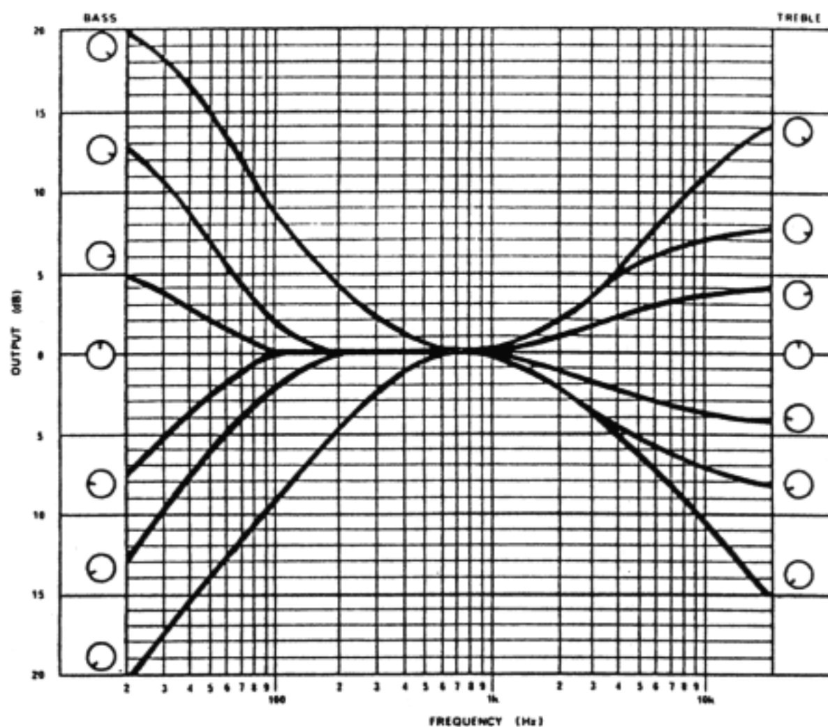
Fig. 14. EFFECT OF BASS AND TREBLE CONTROLS
