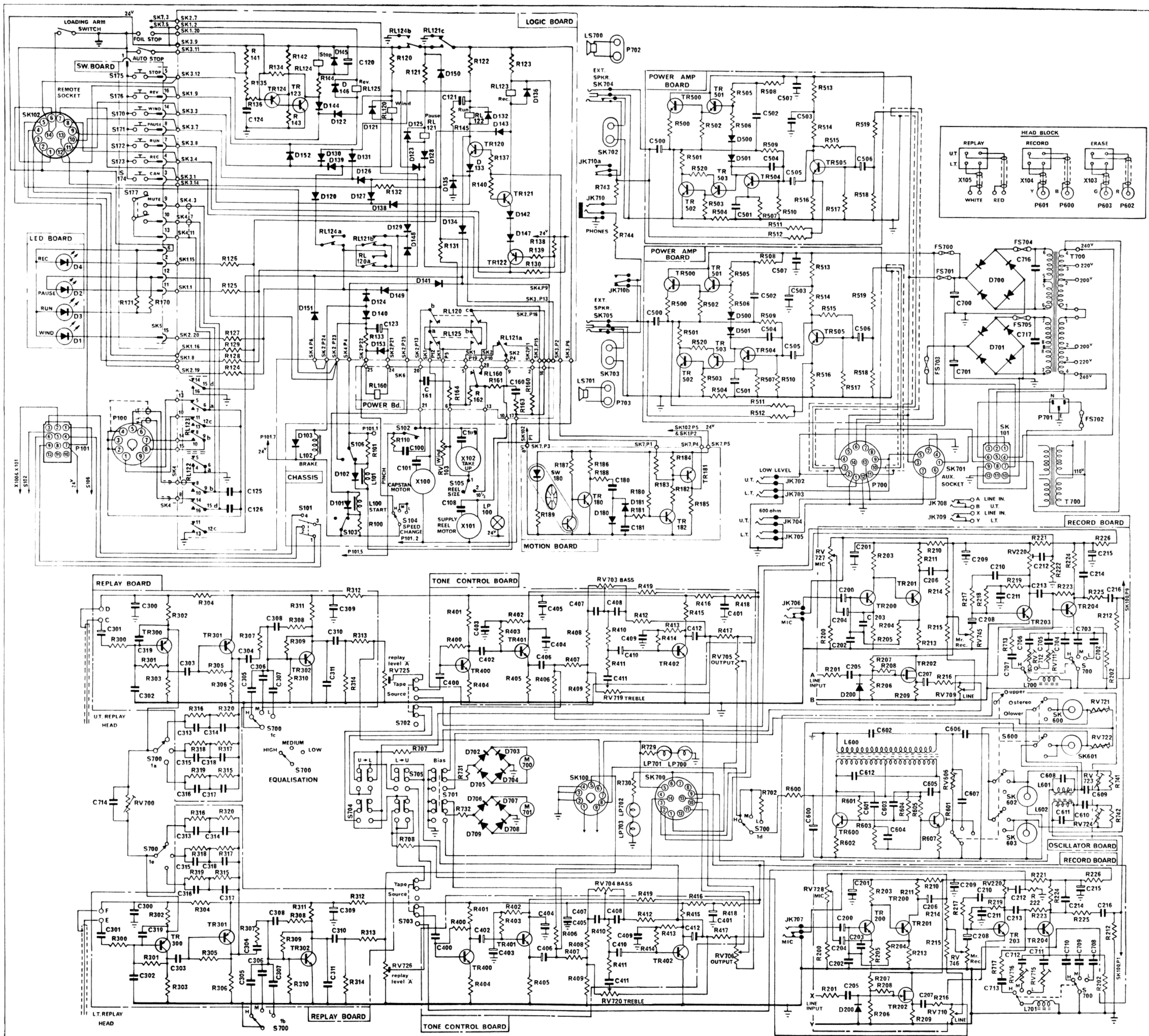
FIG. 30. CIRCUIT DIAGRAM OF RECORDER
