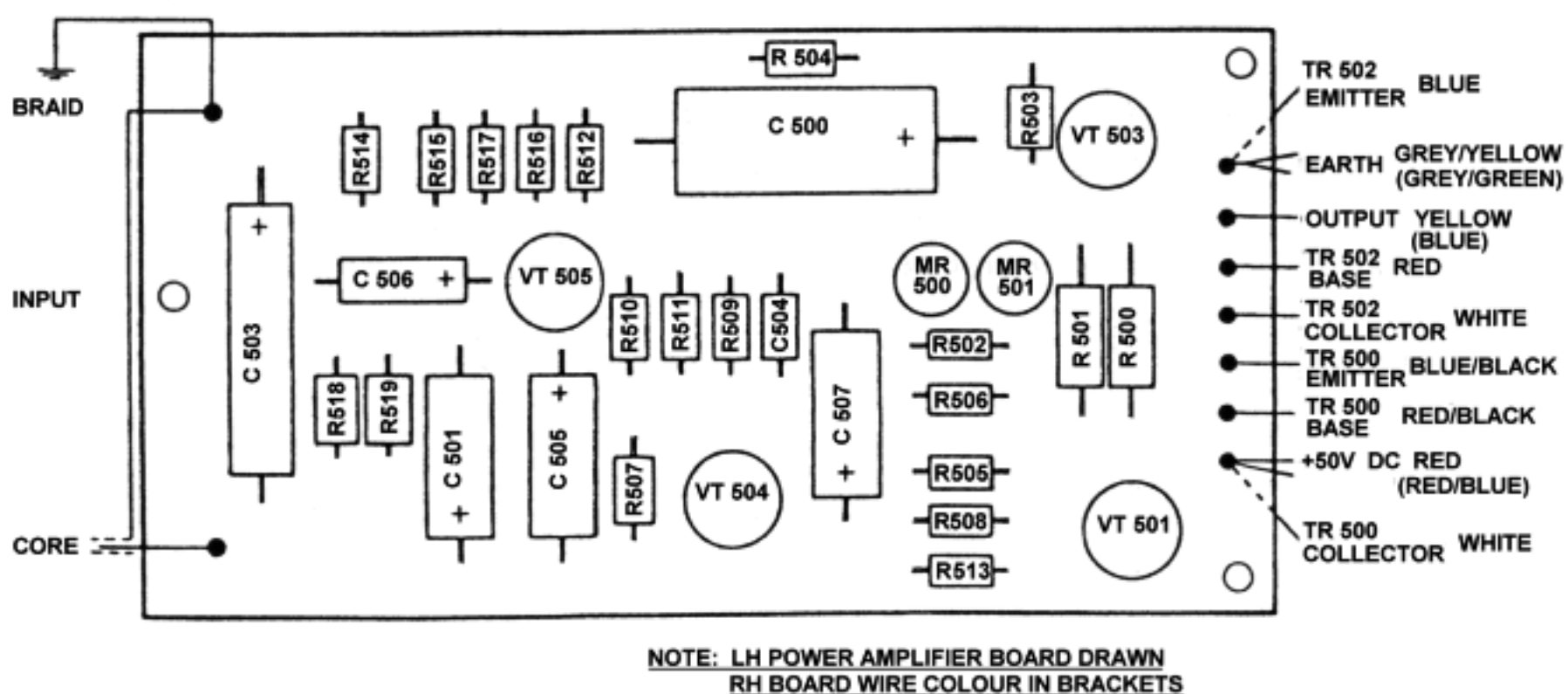
Fig. 33. POWER AMPLIFIER BOARD
