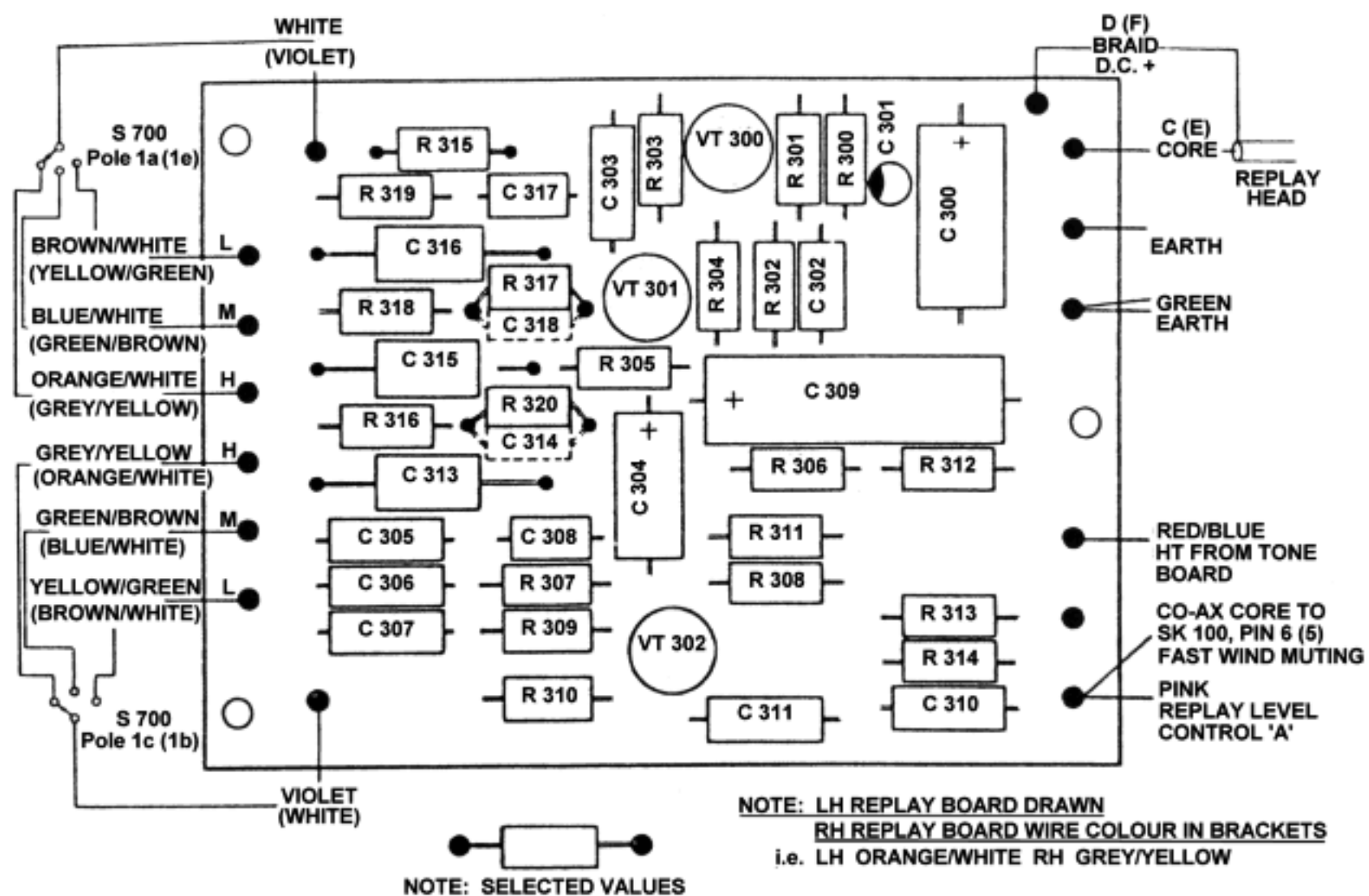
Fig. 32. REPLAY BOARD
