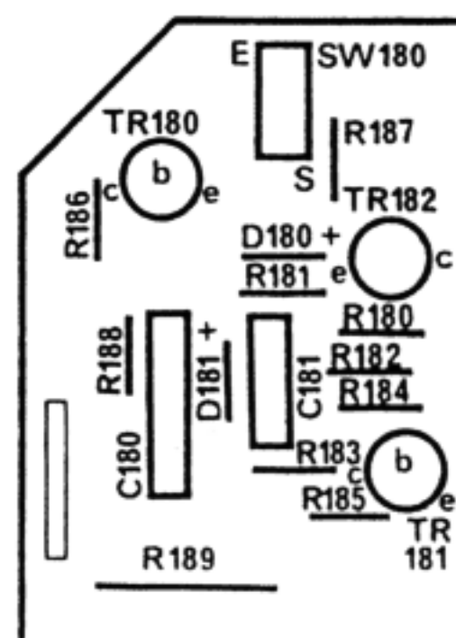
Fig. 37. MOTION SENSOR BOARD
