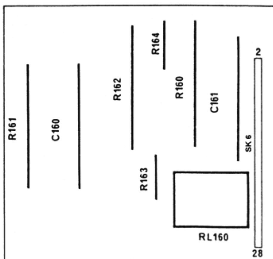
Fig. 35. POWER BOARD
