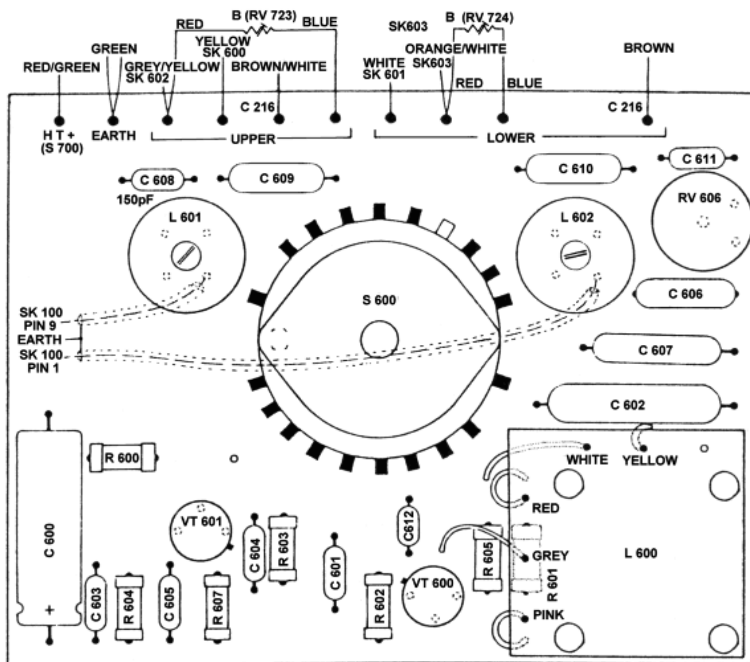
Fig. 28. OSCILLATOR BOARD
