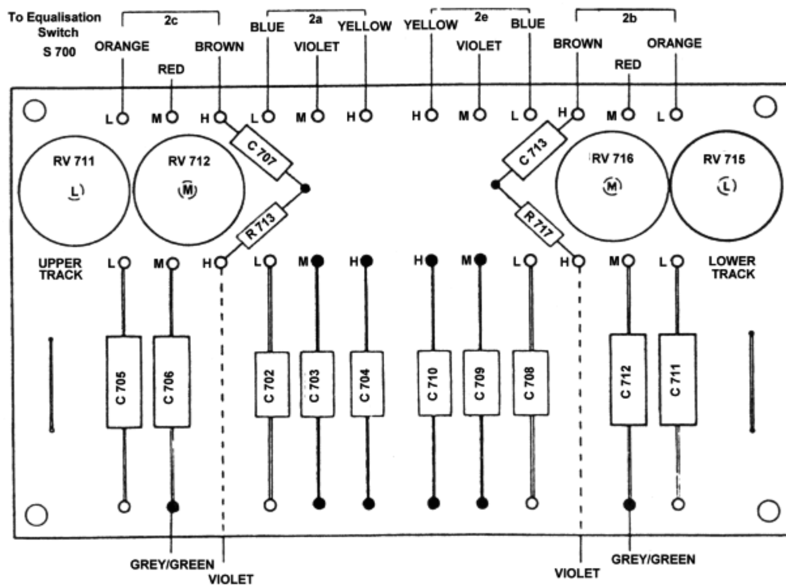
Fig. 31. PRE-EMPHASIS BOARD
