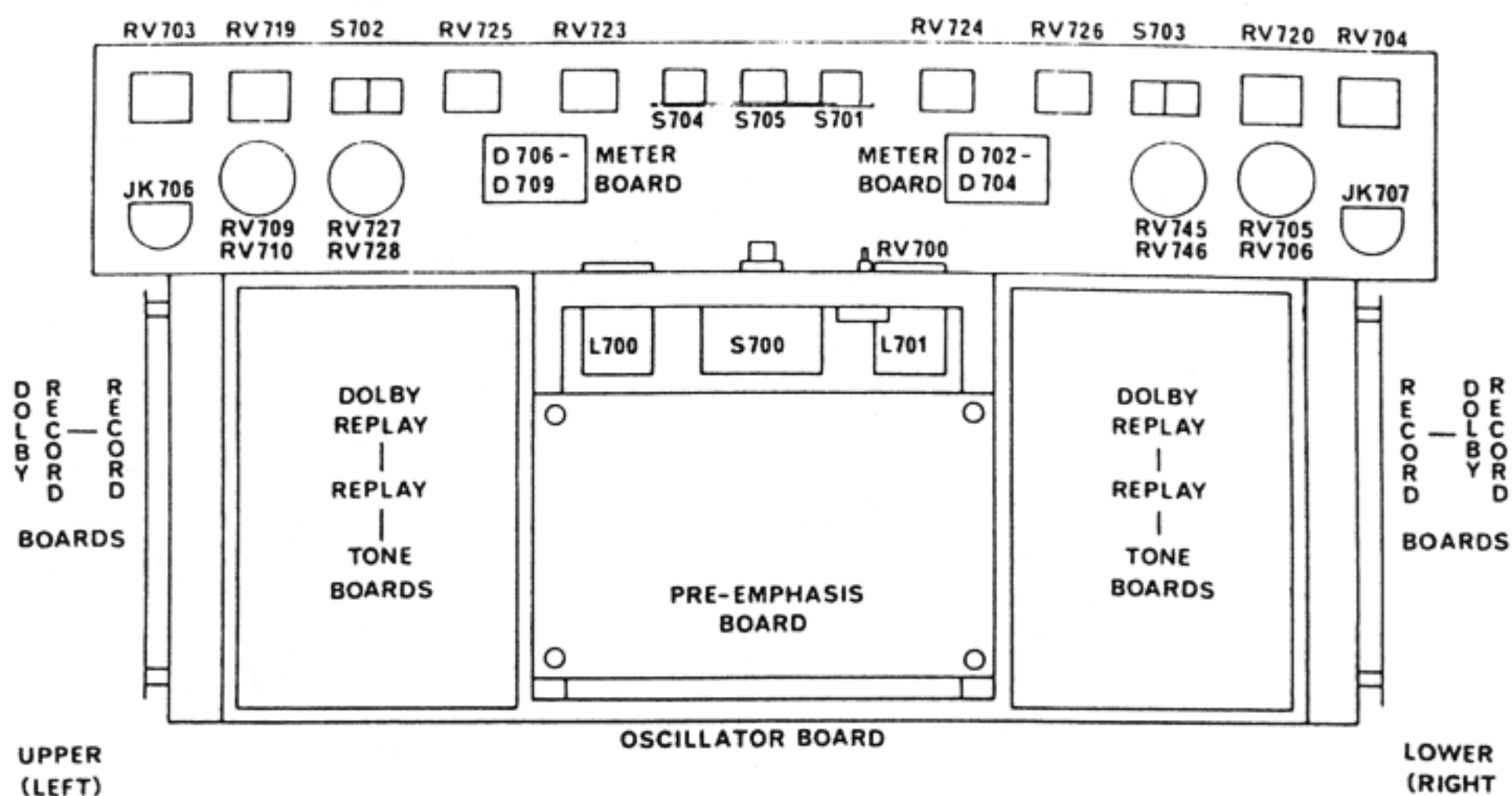
Fig. 22. AMPLIFIER—FRONT VIEW
