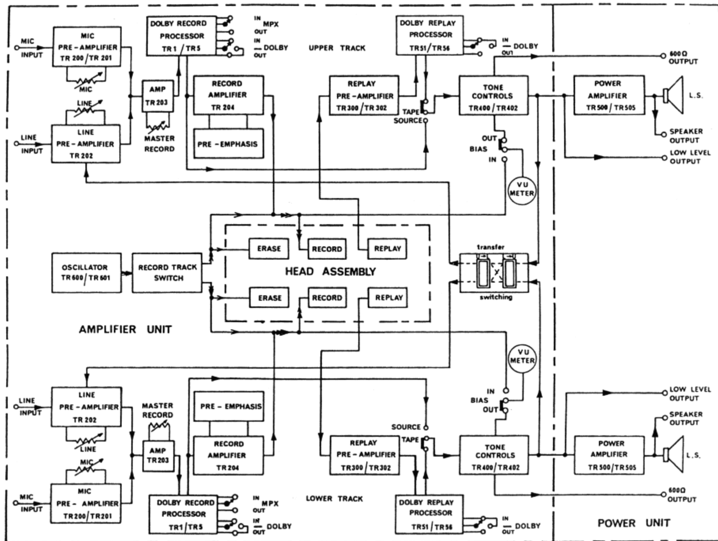
Fig. 39. BLOCK DIAGRAM—DOLBY MODELS (Suffix D)
