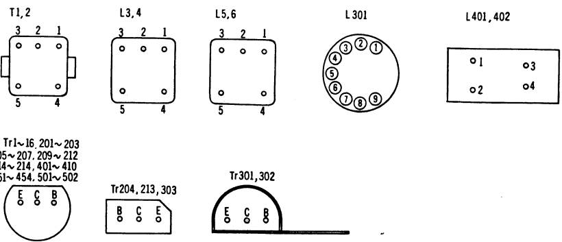
TRANSISTOR TRANSFORMER & COIL TERMINATION (BOTTOM VIEW)
