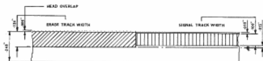
FIG. 21. MONO TRACK DIMENSIONS MODEL 713
