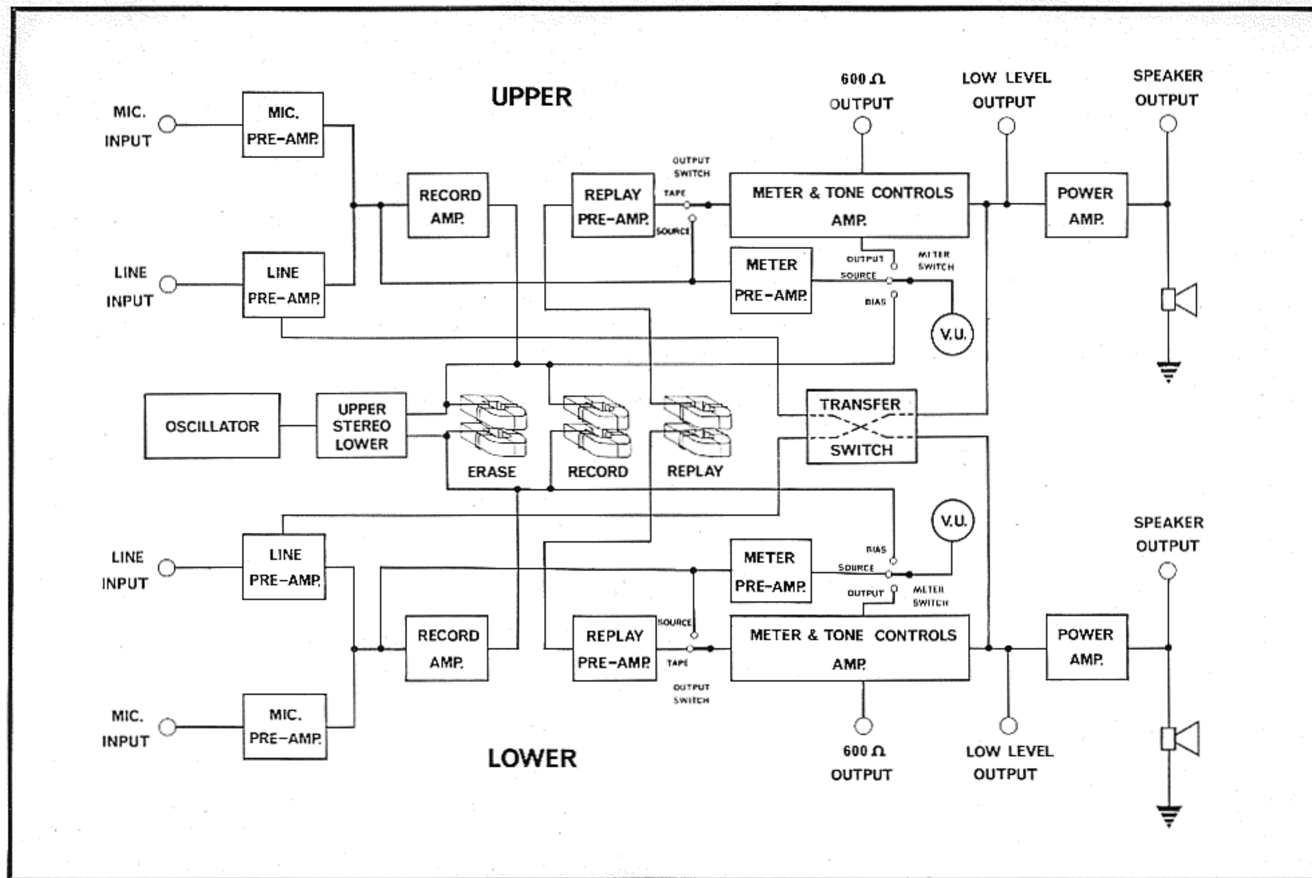
FIG. 16. BLOCK DIAGRAM—STEREO MODELS
