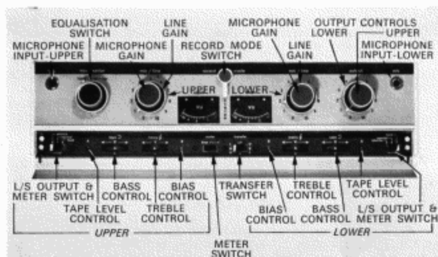
FIG. 8. AMPLIFIER CONTROLS—STEREO
