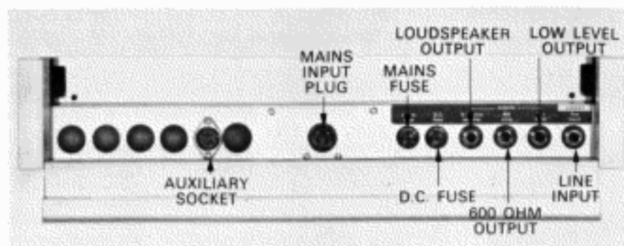
FIG. 3. REAR PANEL—MONO
