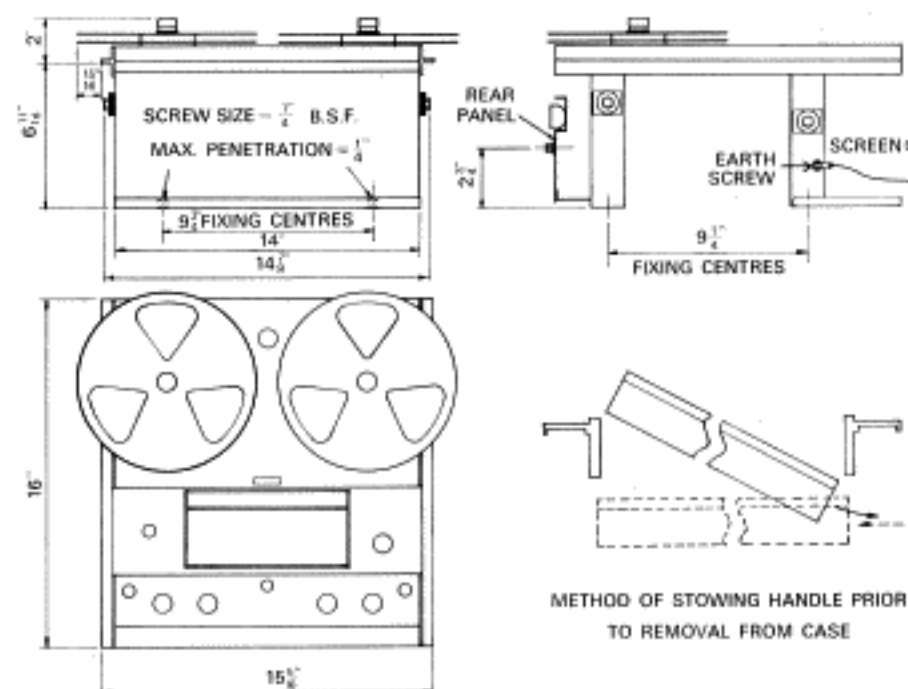
FIG. 15. CHASSIS MODEL DIMENSIONS
