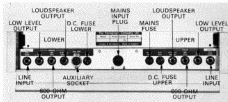
FIG. 4. REAR PANEL—STEREO
