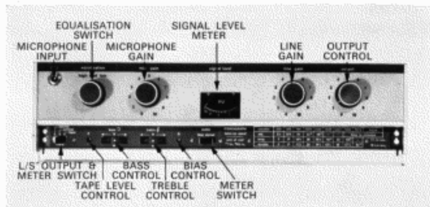
FIG. 7. AMPLIFIER CONTROLS—MONO
