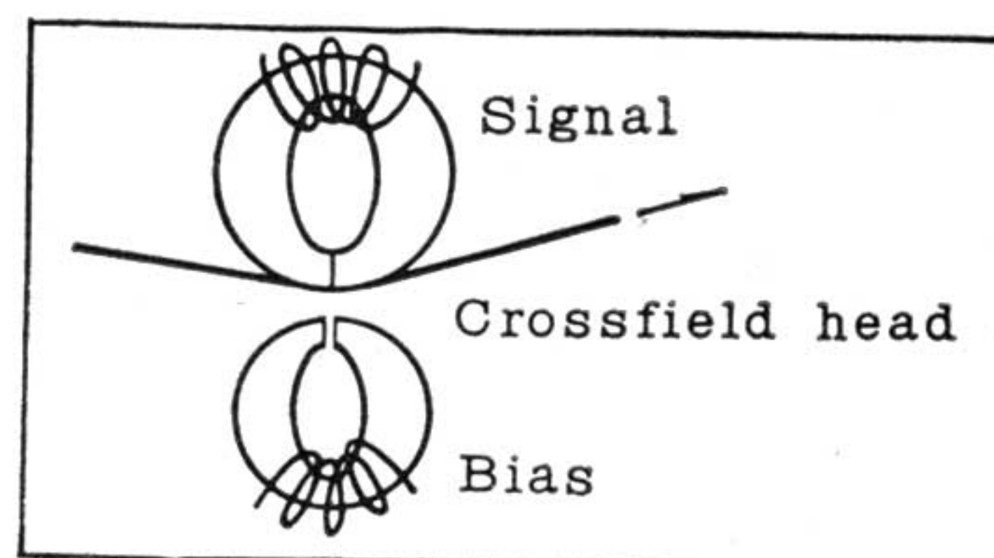
Diagram 2. Cross-field recording system
