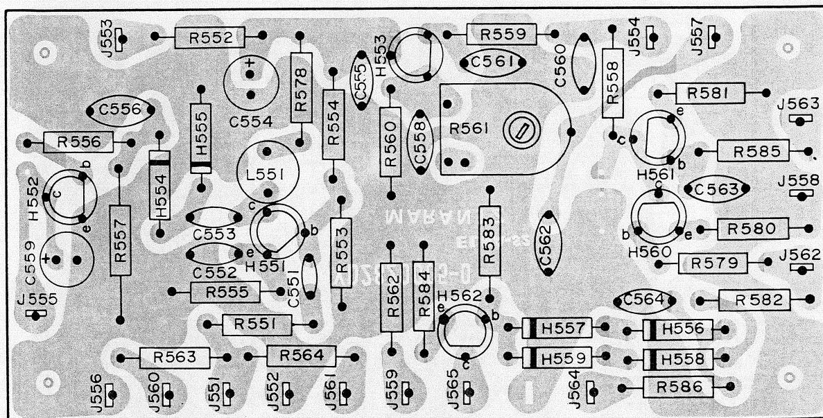
Figure 12. Muting Control Amplifier Assembly P550 Component Locations
