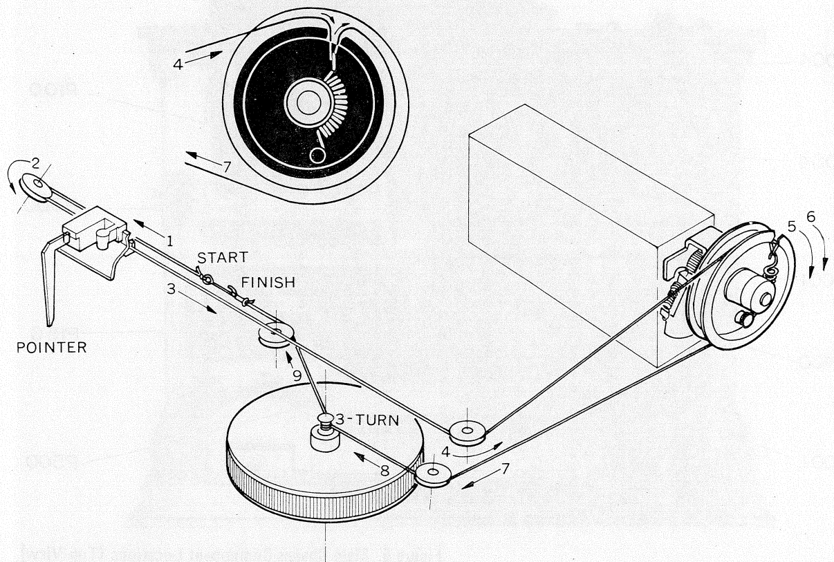
Figure 3. Dial Stringing
