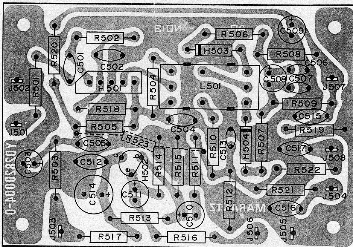
Figure 10. FM Detector P500 Component Locations
