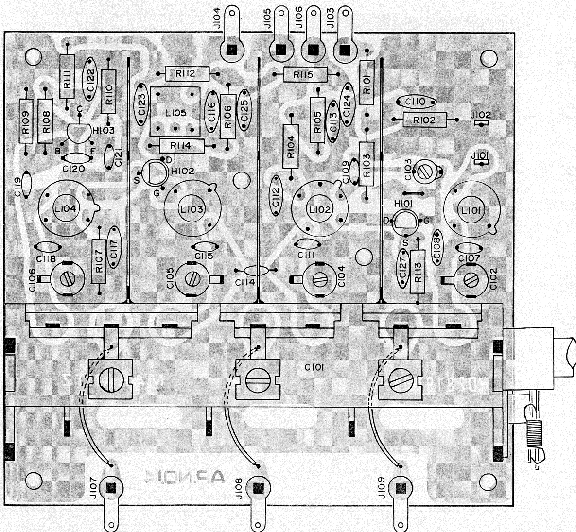
Figure 8. FM Front End Assembly P100 Component Locations
