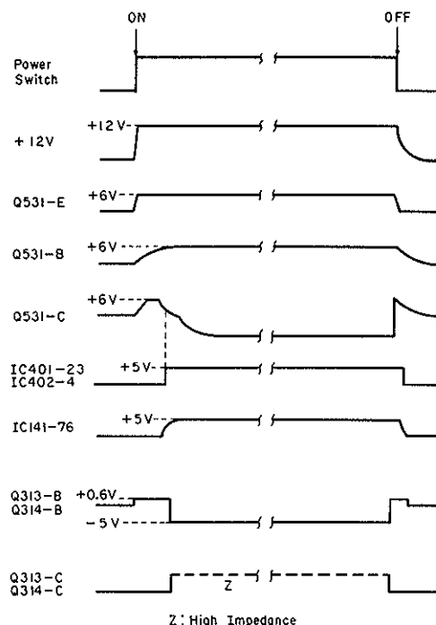
Fig. 10 Reset Timing Chart
