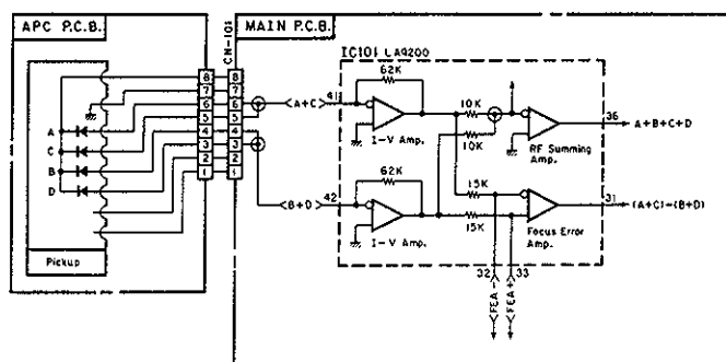
Fig. 21 RF Amp. Circuit
