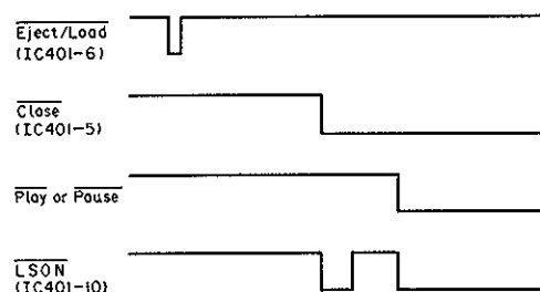
Fig. 16 Laser ON/OFF Timing Chart
