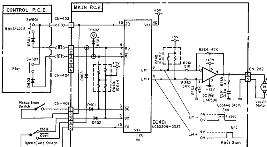
Fig. 11 Eject/Load Circuit
