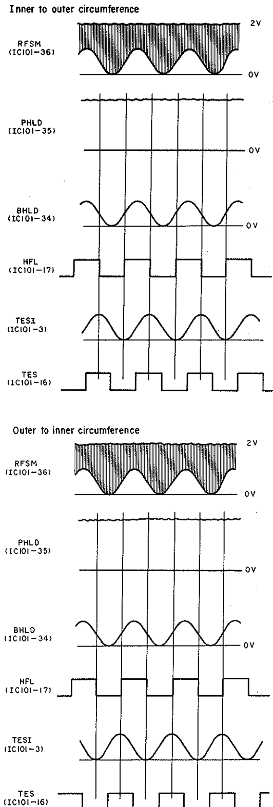
Fig. 32 HFL and TES Signals
