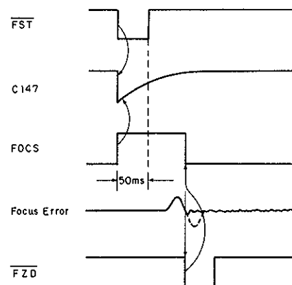
Fig. 24 Timing Chart
