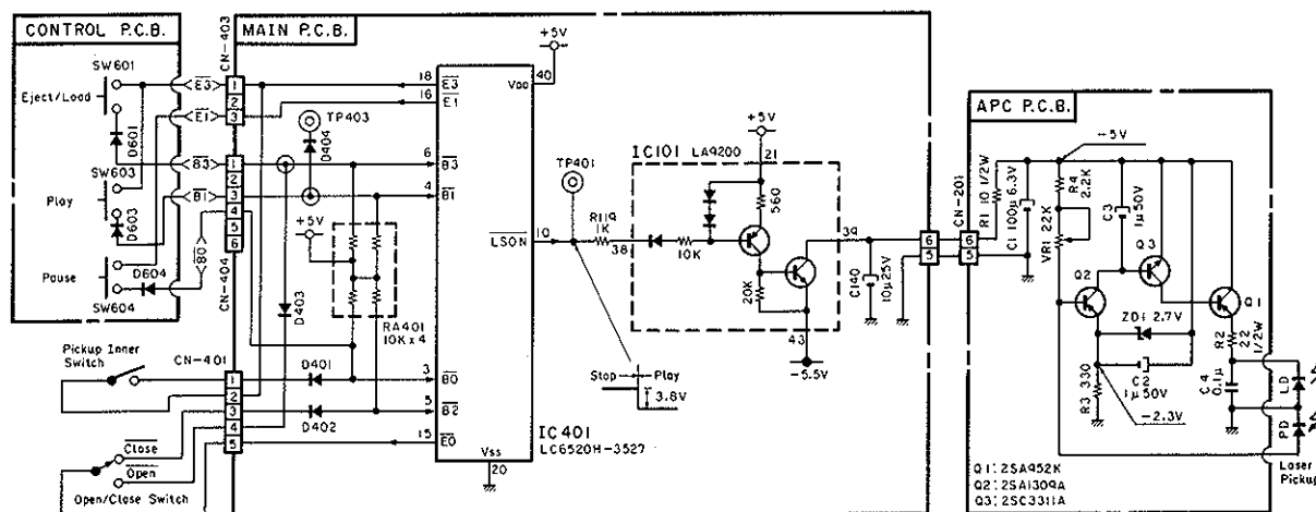
Fig. 15 Auto Power Control Circuit
