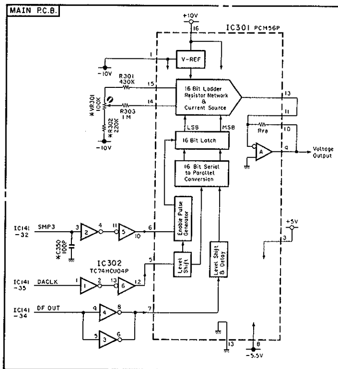
Fig. 57 D/A Converter Circuit
