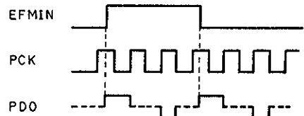
Fig. 41 Timing Charts at PDO Pin
