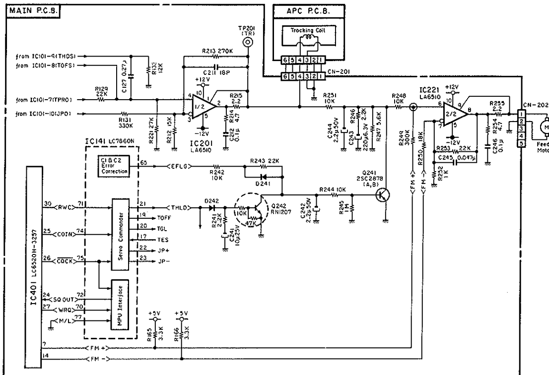
Fig. 30 Feed Servo Circuit
