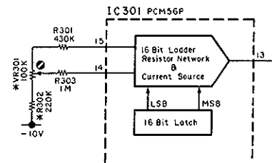
Fig. 59 MSB Correction Circuit
