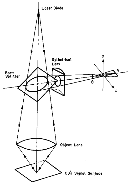
Fig. 18 Astigmatism Method
