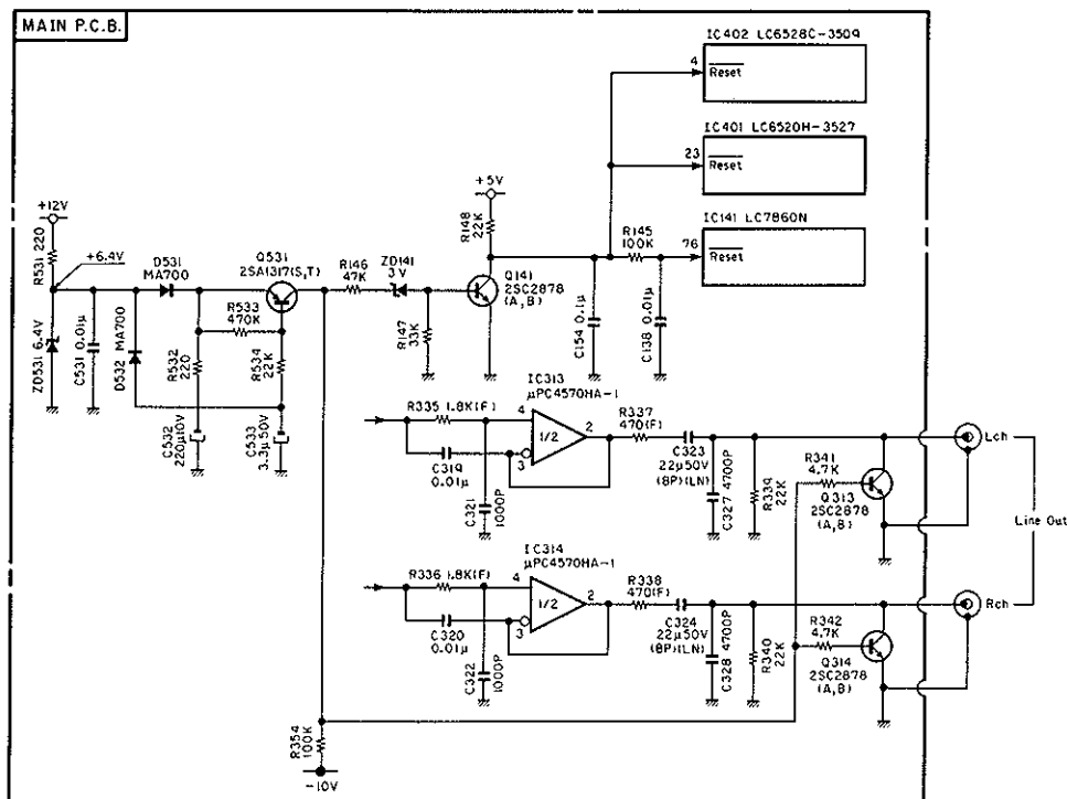
Fig. 9 Reset Circuit
