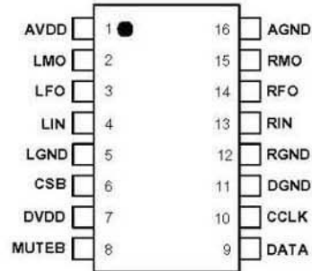
WM8816
