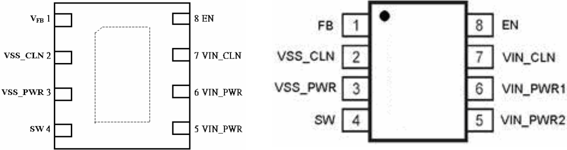
Pin Function FBP-8, Adjustable
