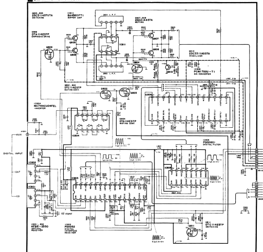
1. D/A CONVERTER CIRCUIT
