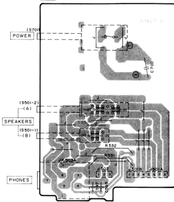
I POWER SWITCH/HEADPHONES P.C.B.
