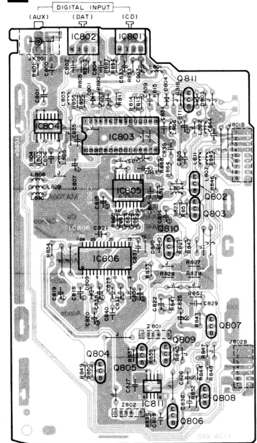
A D/A CONVERTER P.C.B.
