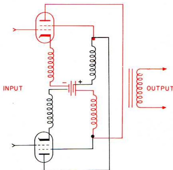
Figure 2. Representation of McIntosh output circuit
