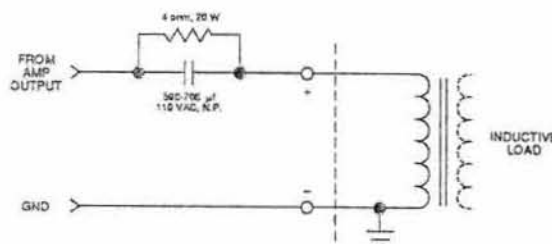
Fig. A.5 Connection to an Inductive Load
