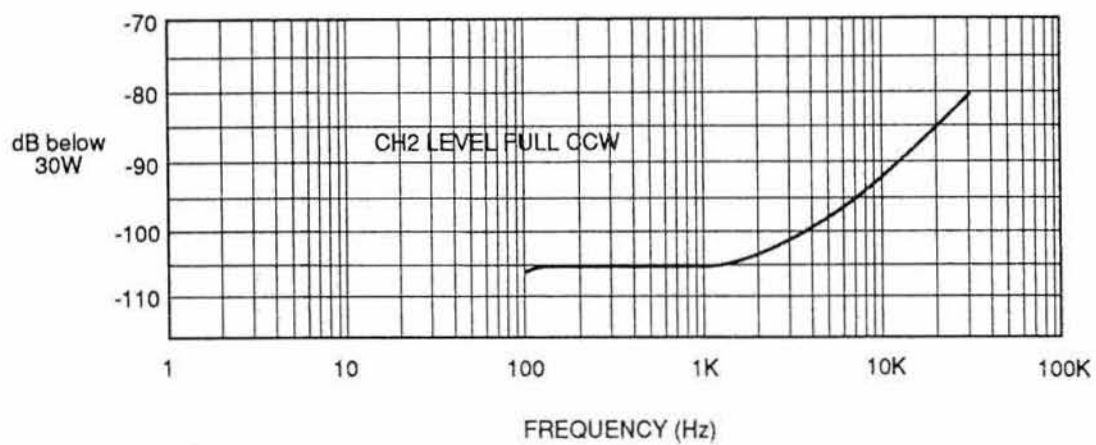
Fig. 7.8 Nominal Crosstalk
