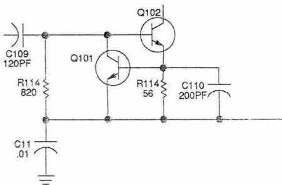
Fig. 6.5 Final Voltage Amplifier
