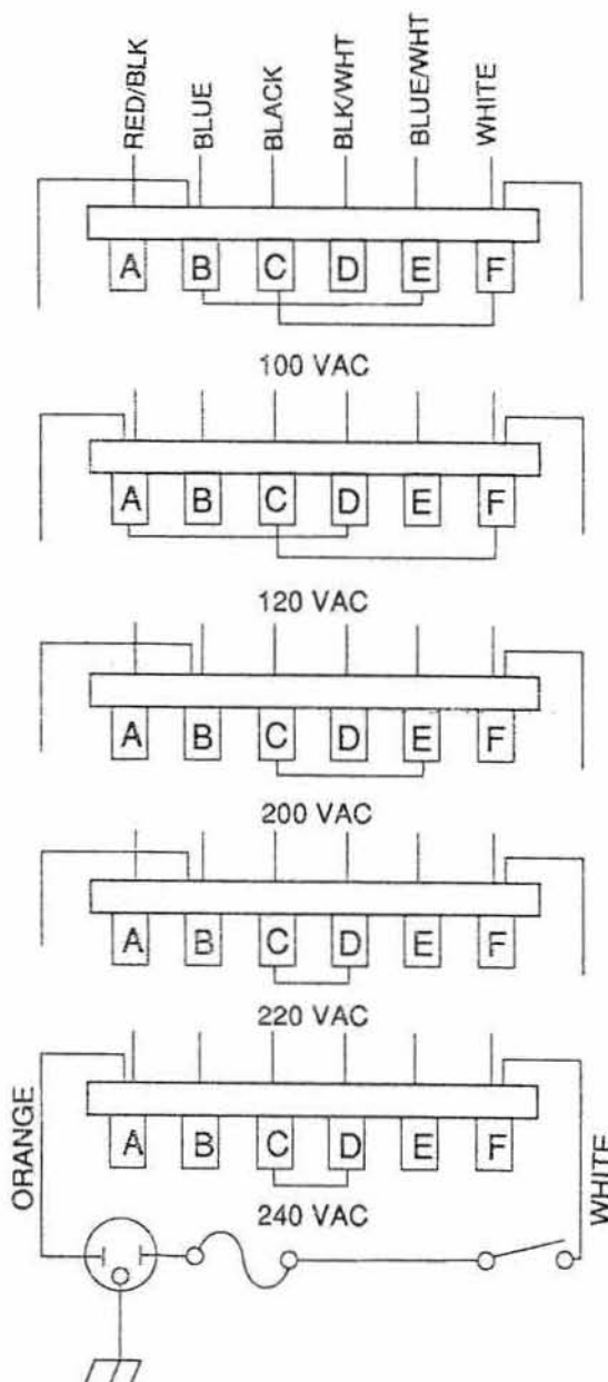
Fig. 5.1 AC Mains Voltage Conversion
