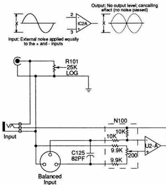
Fig. 6.2 Balanced Input Stage
