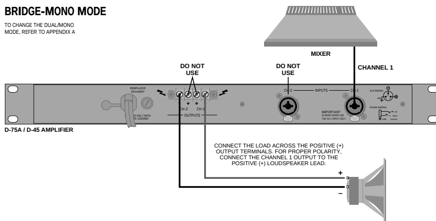
Fig. 2.2 System Connection
