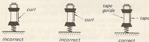
Fig. 3-12. Curl elimination
