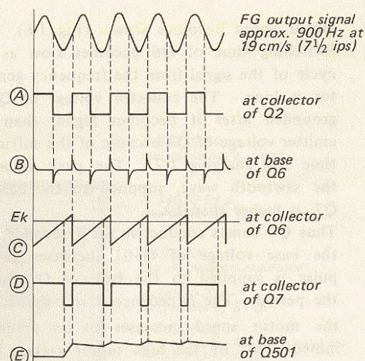
Fig. 1-4. Waveform at each point
