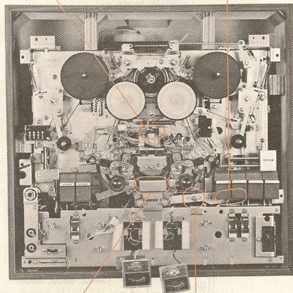
11. Pinch Roller Lever Adjustment 9. Pinch Roller Timing Adjustment
