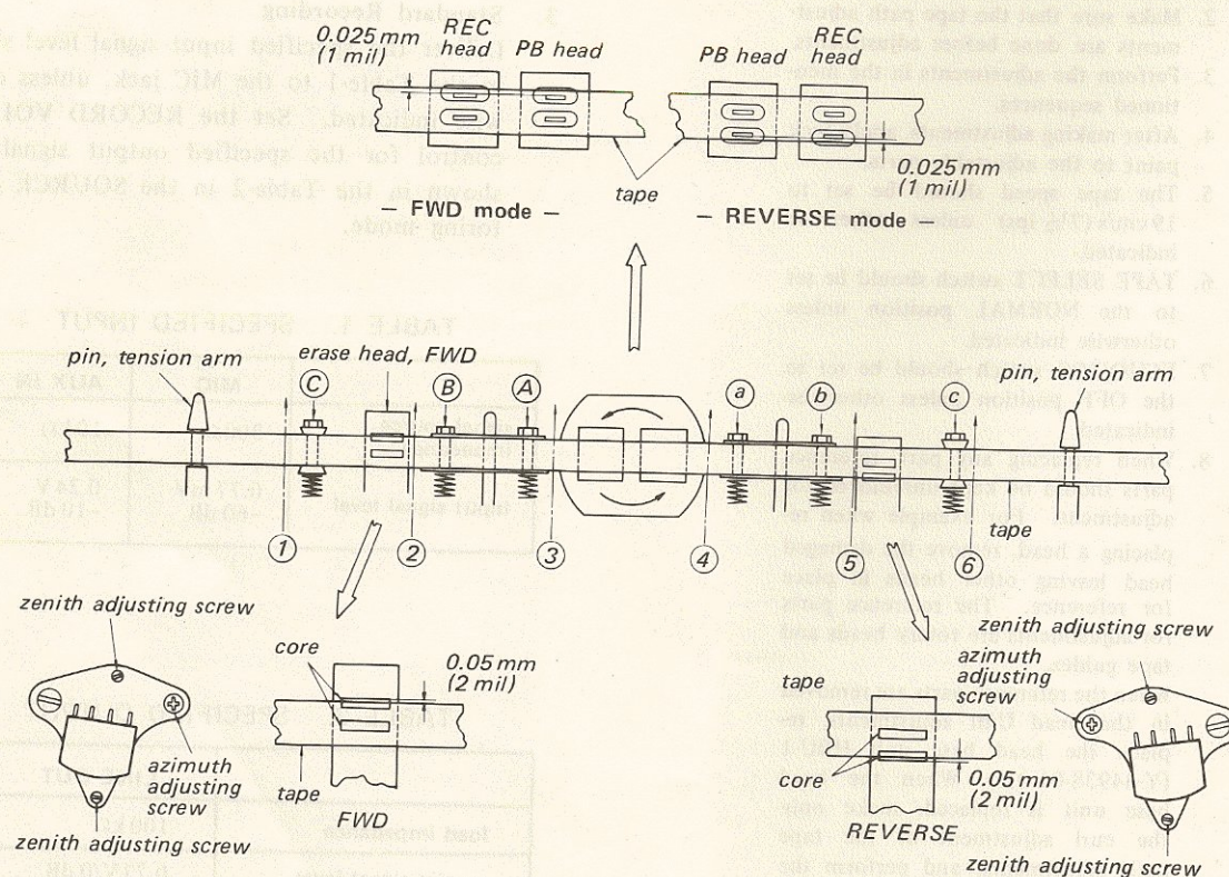
Fig. 3-11. Tape path adjustments
