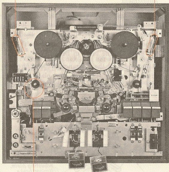
26. Tension Arm Pin Height Adjustment
