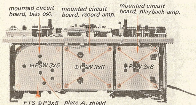
Fig. 2-2. Circuit board removal
