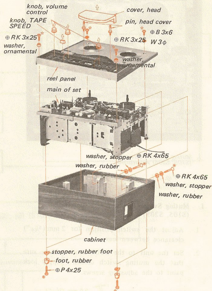
Fig. 2-1. Reel panel and cabinet removal
