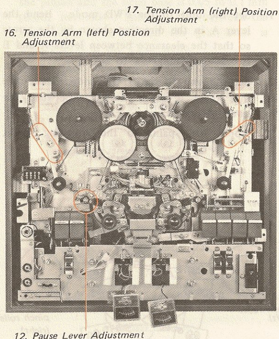
Fig. 3-6. Adjusting parts location
