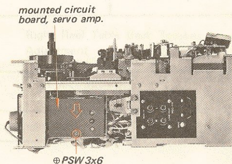
Fig. 2-4. Servo amp. circuit board removal
