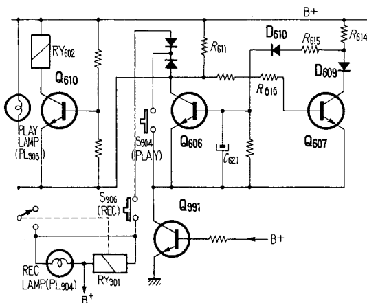
Fig. 1-3-1. Flip-flop circuit
