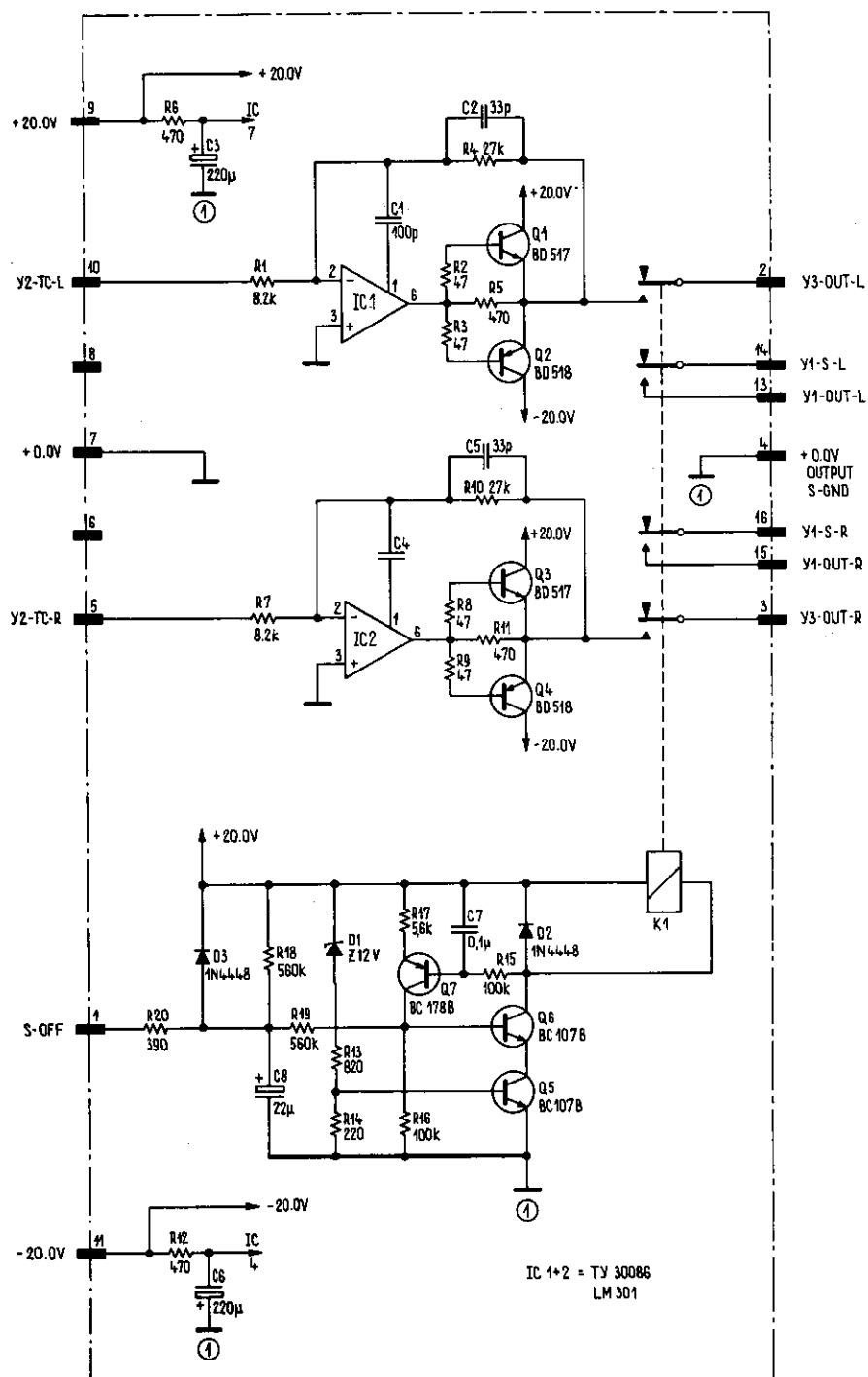
HEADPHONE AMPLIFIER 1.067.421
