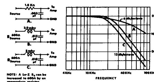
Fig. 3.9 RFI Filters
