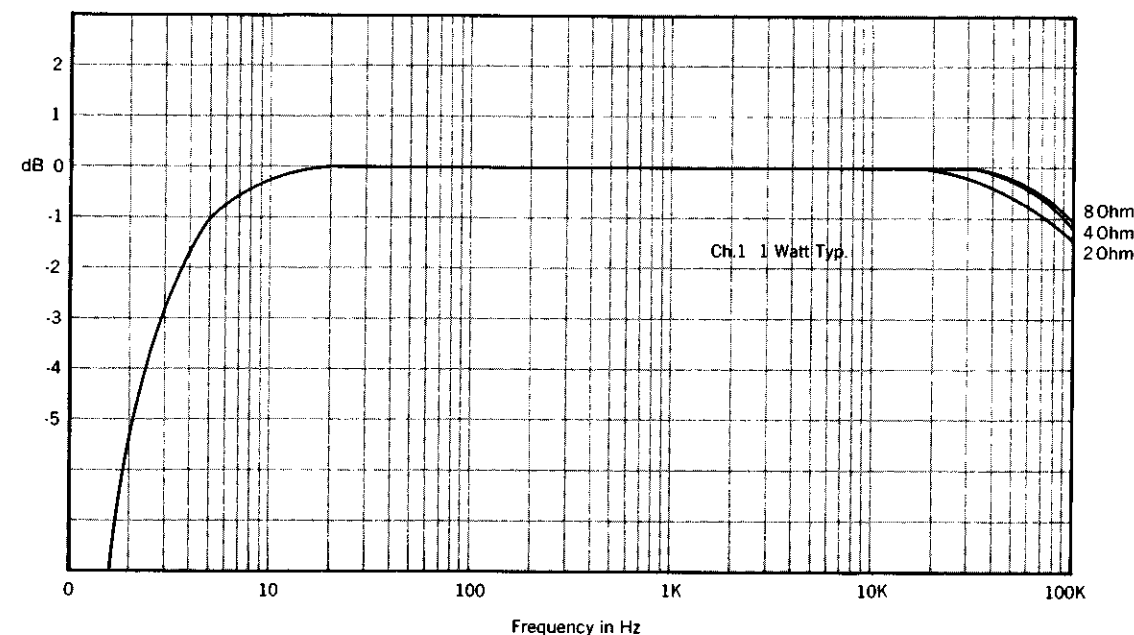
Fig. 2.1 Typical Frequency Response
