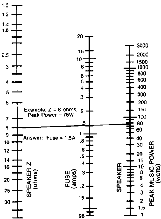
Fig. 3.10 Fuse Selector Nomograph for Loudspeaker Protection
