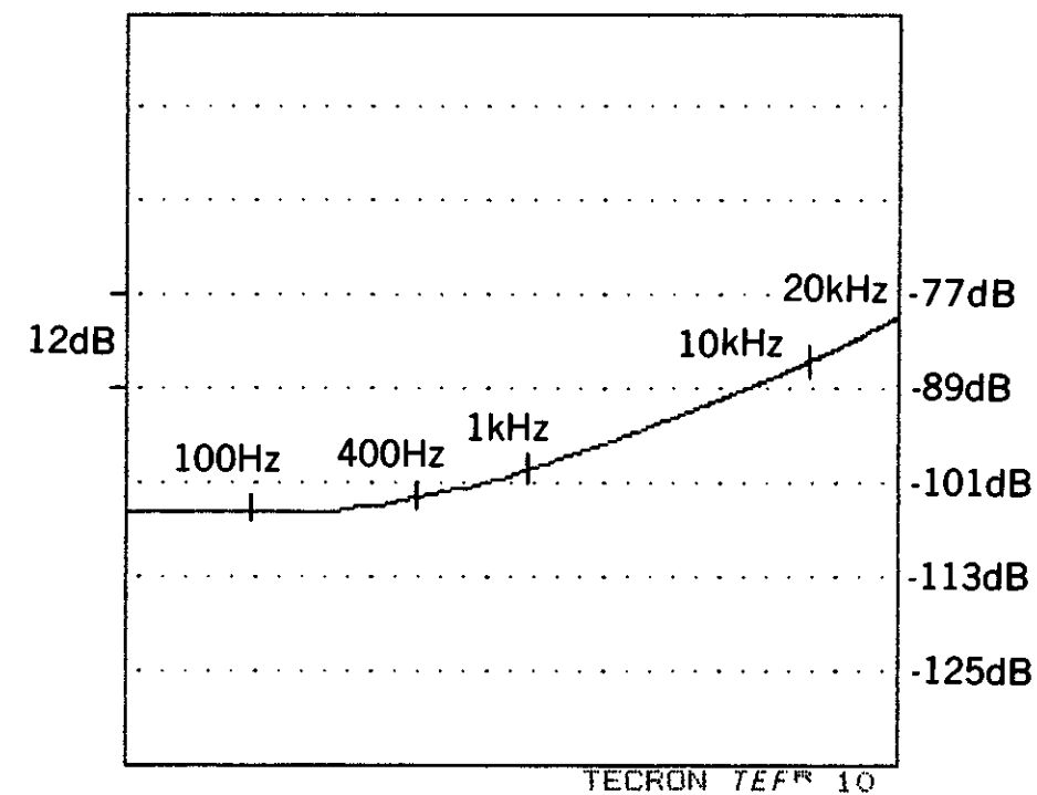
Fig. 2.8 Typical Crosstalk
