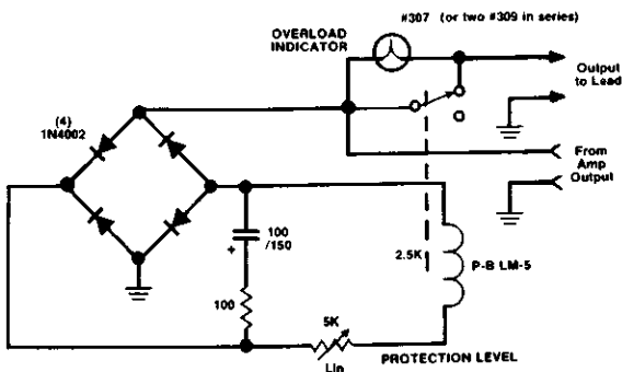
Fig. 3.11 Relay-Controlled Protector with Overload Indicator
