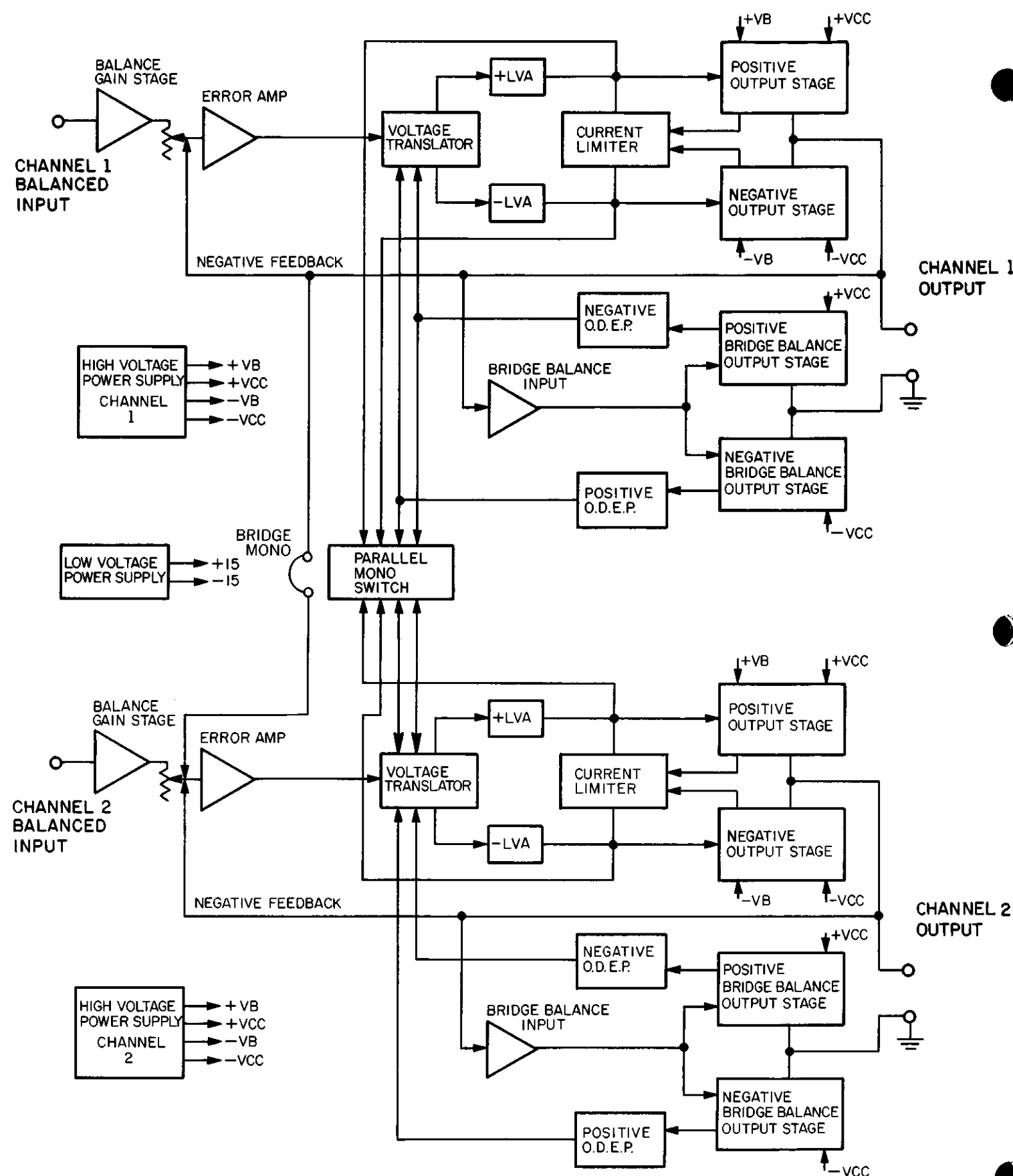
Fig. 4.1 Block Diagram
