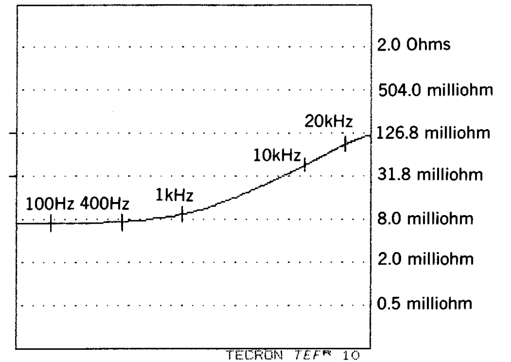
Fig. 2.9 Typical Output Impedance
