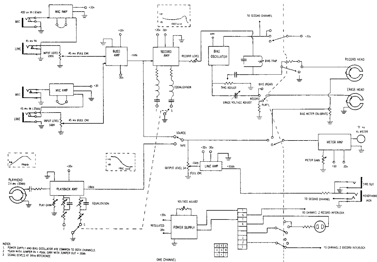
FIG. 7-5 BLOCK DIAGRAM
