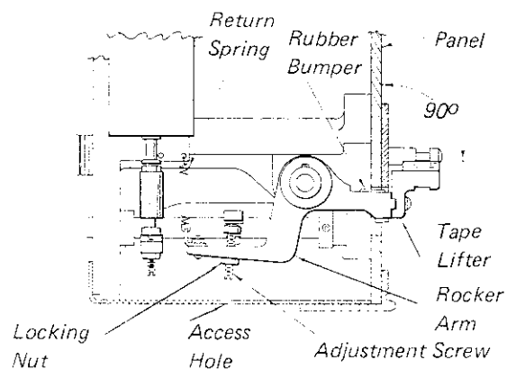
FIG. 5-6 TAPE LIFTER
