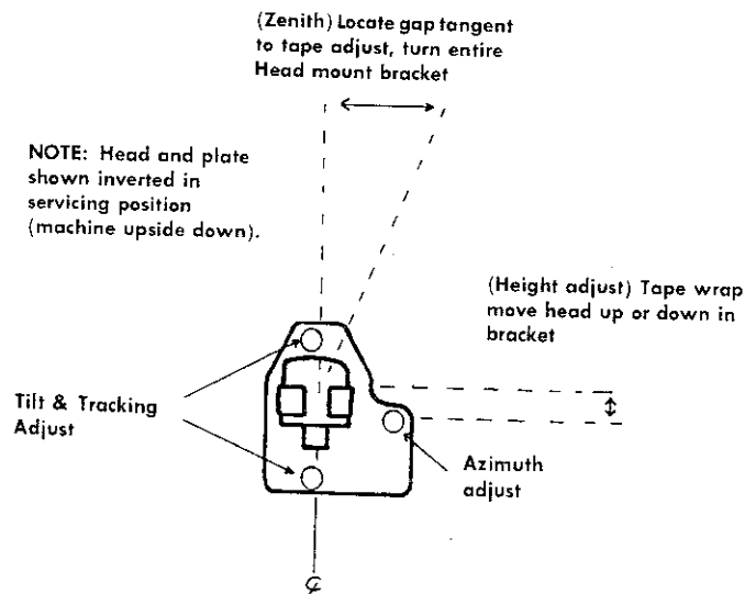
FIG. 10-8 HEAD ALIGNMENT
