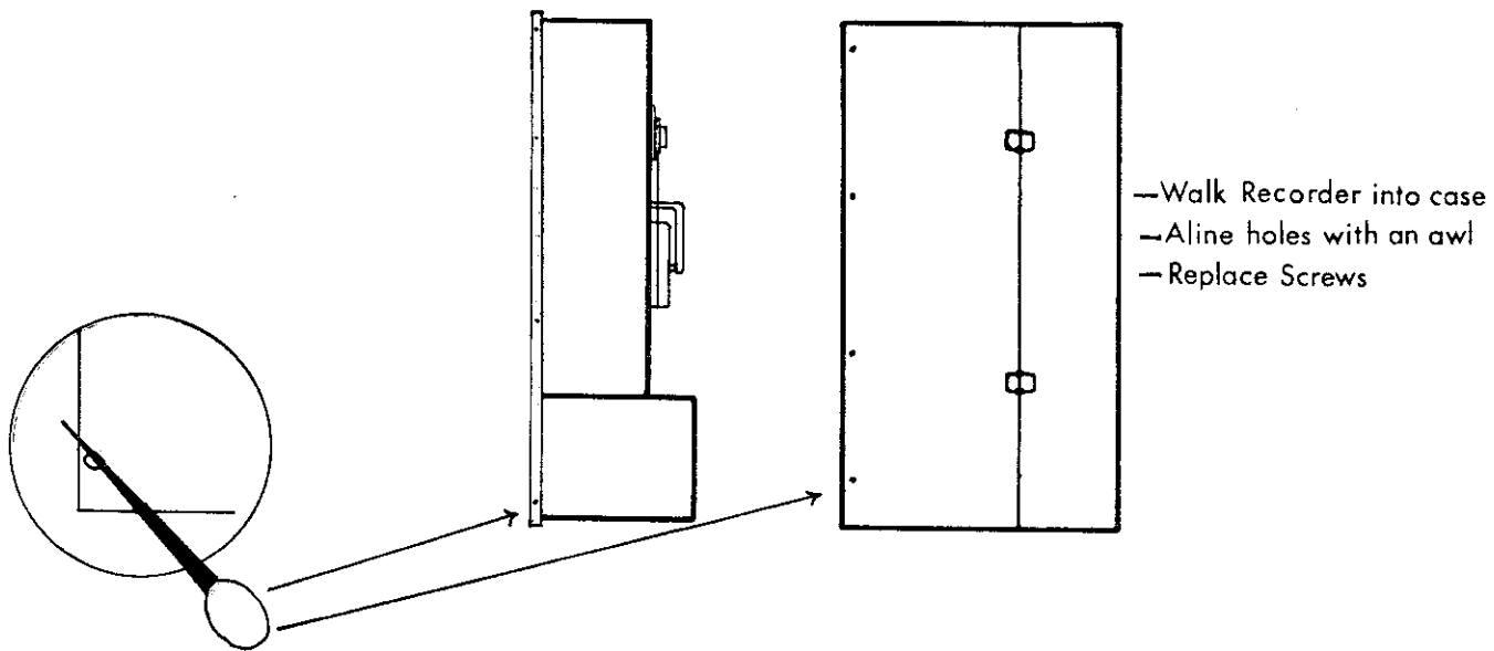
FIG. 8-2 CASING
