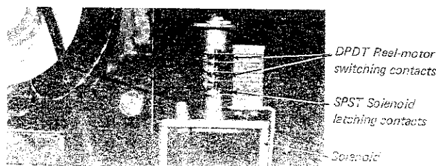
FIG. 5 - 8 STACK-SWITCH ASSEMBLY
