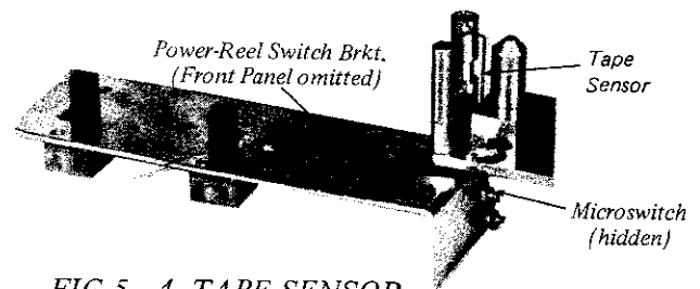
FIG 5 - 4 TAPE SENSOR
