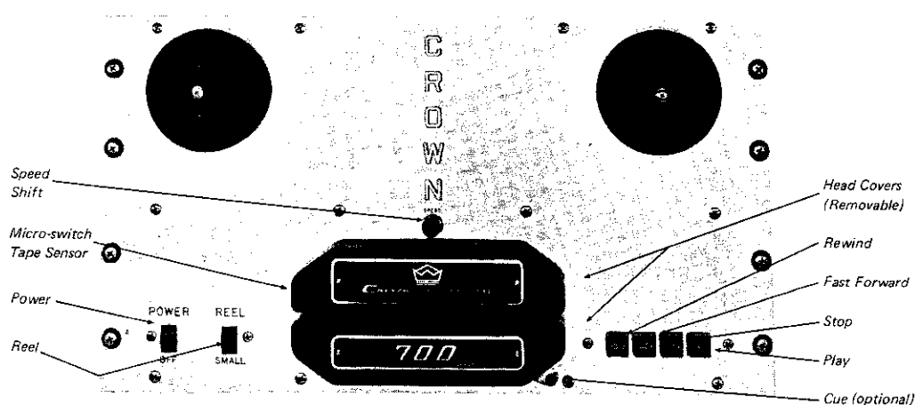
FIG. 3 - 1 PRO-700 TRANSPORT CONTROLS
