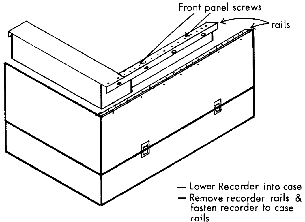
FIG. 8-1 CASING
