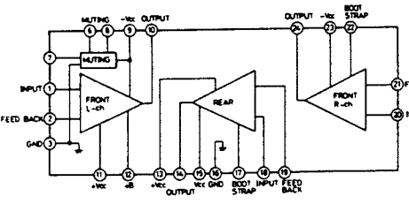
IC403 STK4152MK2(3 - Channel AF Power Amplifier)
