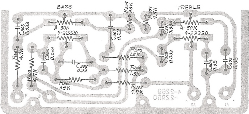
TONE P.C.B. ASSEMBLY
