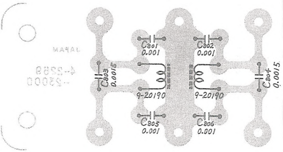
MPX., 38KHz FILTER P.C.B. ASSEMBLY
