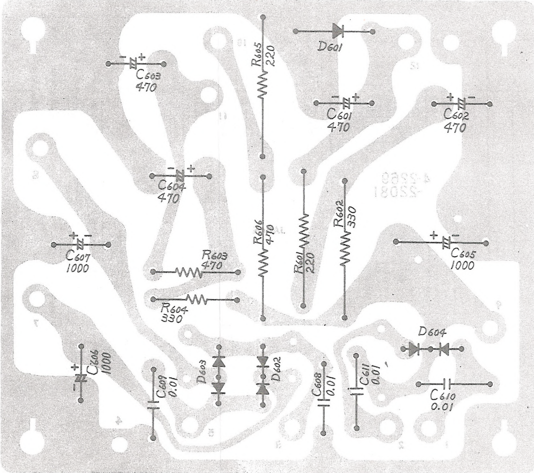
POWER SUPPLY P.C.B. ASSEMBLY
