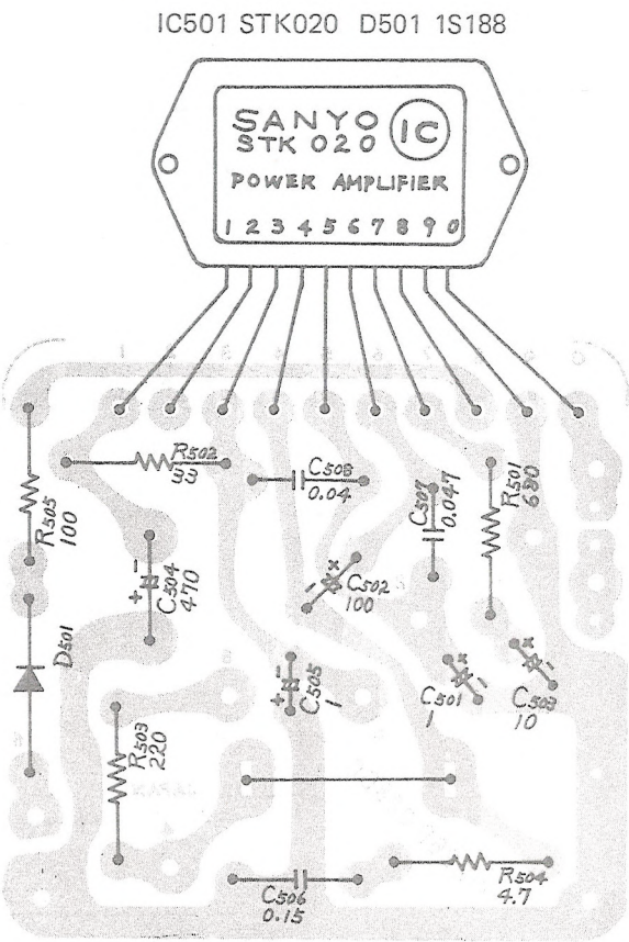
MAIN AMP P.C.B. ASSEMBLY
