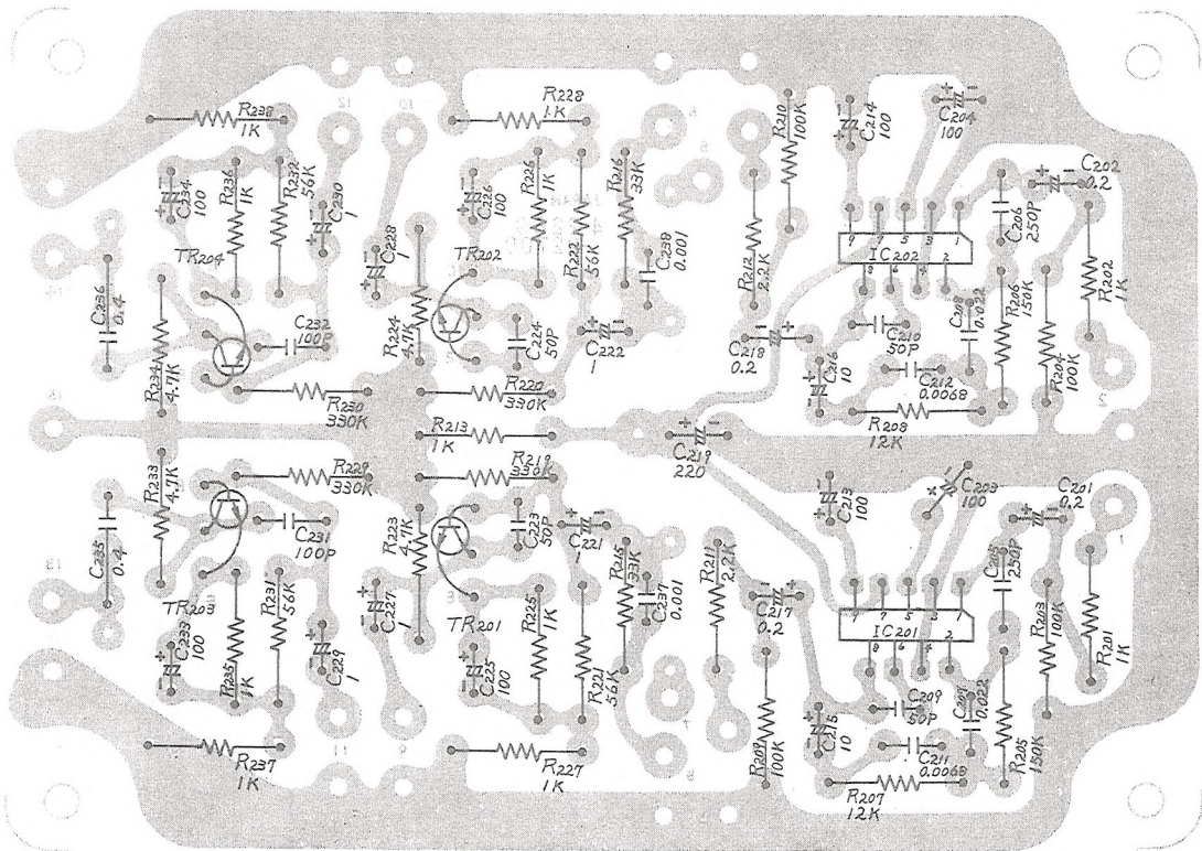
PRE AMP P.C.B. ASSEMBLY
