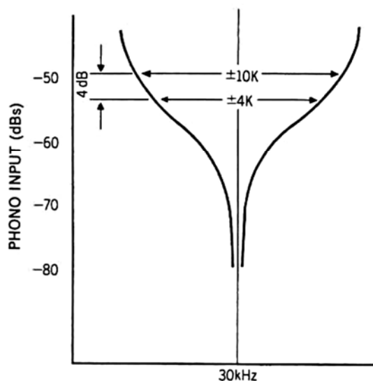
Figure 11. Phono Input Level vs. Lock Range
