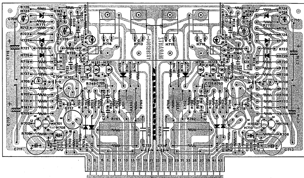
Figure 15. Power Amplifier Assembly P700 Component Locations and Schematic Diagram
