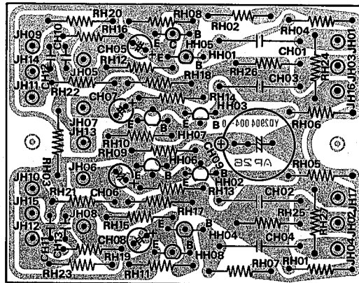
Figure 23. Filter Amplifier Assembly PH01 Component Locations
