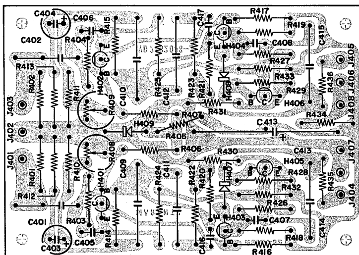
Figure 12. Phono Amplifier Assembly P400 Component Locations
