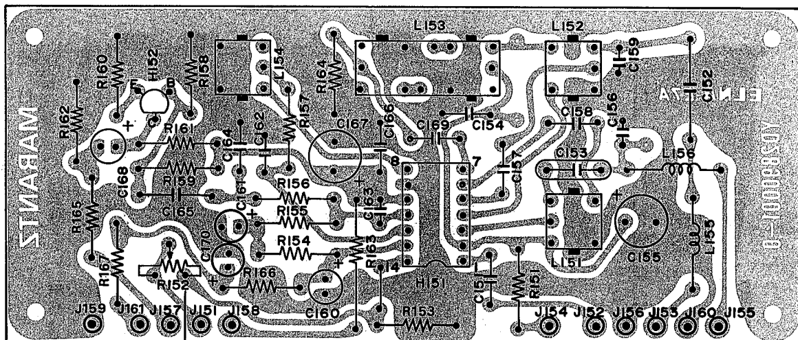
Figure 9. AM Tuner Assembly P150 Component Locations
