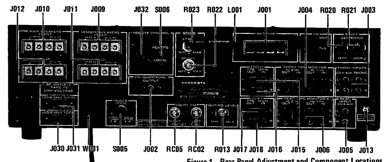
Figure 1. Rear Panel Adjustment and Component Locations
