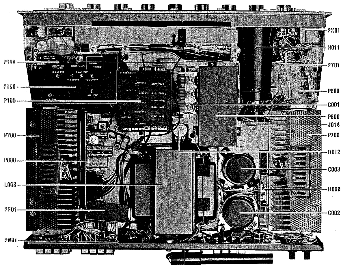
Figure 7. Main Chassis Component Locations (Top View)
