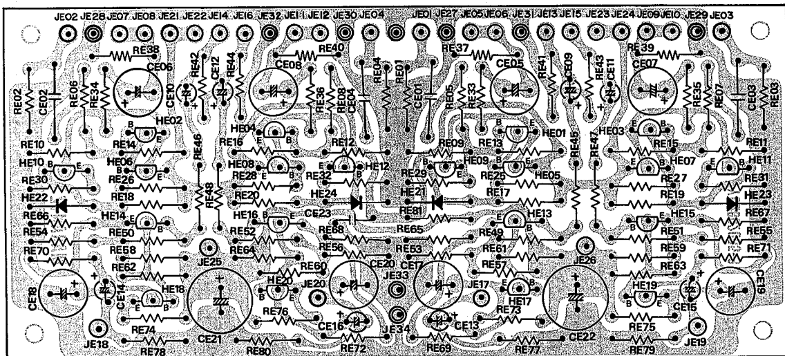
Figure 20. Buffer and Pre-Amplifier Assembly PE01 Component Locations
