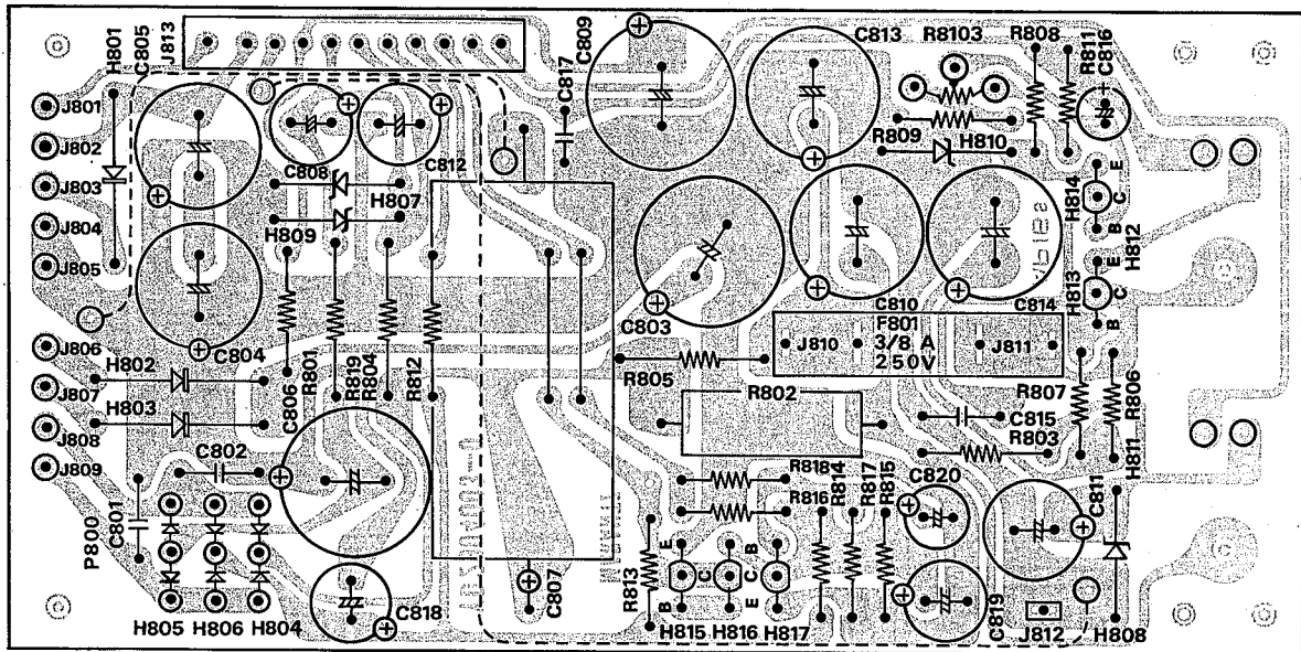
Figure 16. Power Supply Assembly P800 Component Locations
