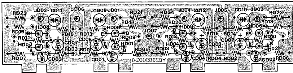
Figure 19. Tone Amplifier Assembly PD01 Component Locations
