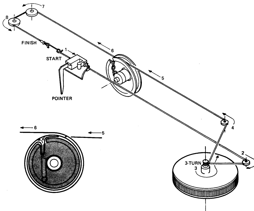
Figure 2. Dial Stringing
