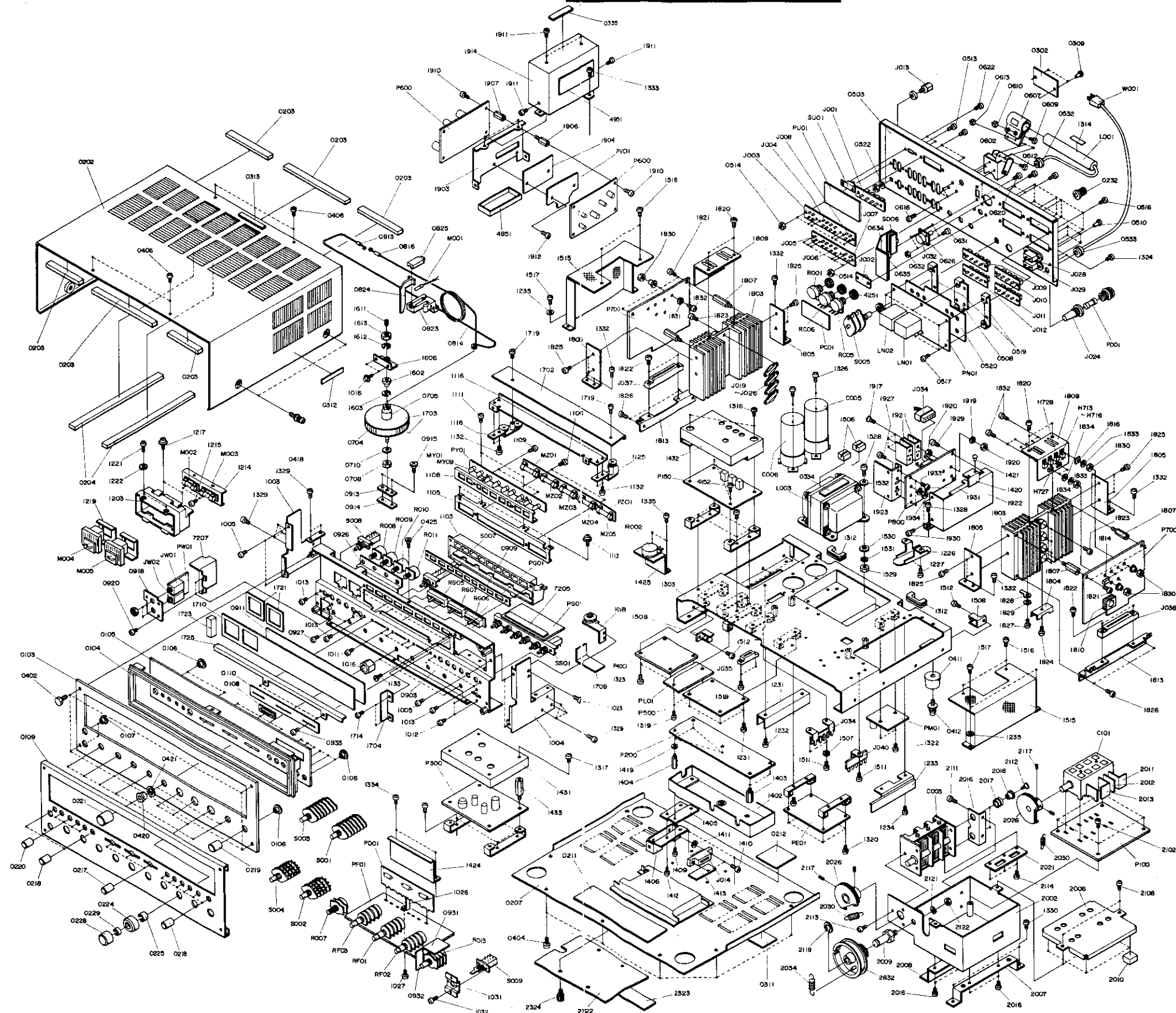
Figure 31. Exploded Mechanical Diagram
