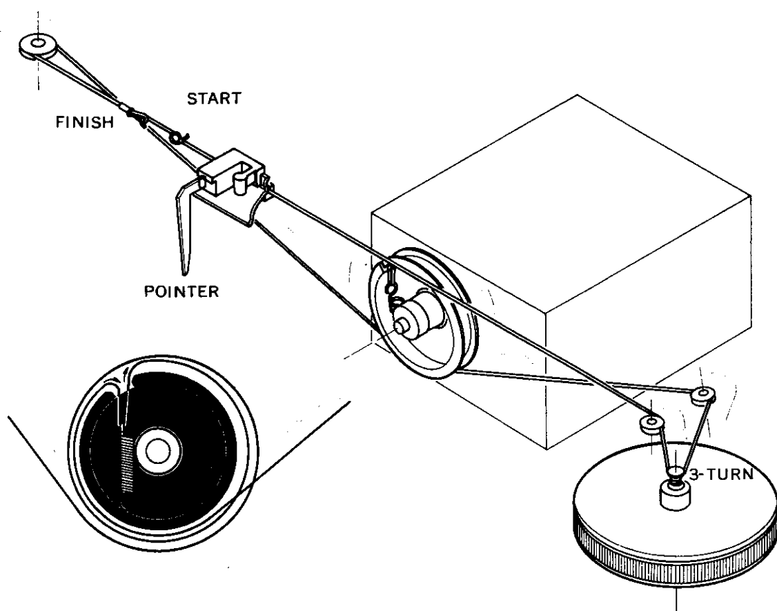
Figure 6. Dial Stringing
