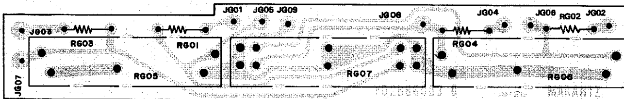
Figure 19. Balance Control Unit Assembly PG01 Component Locations
