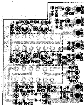
Figure 20. Hi-Filter, Loudness Assembly PH01 Component Locations
