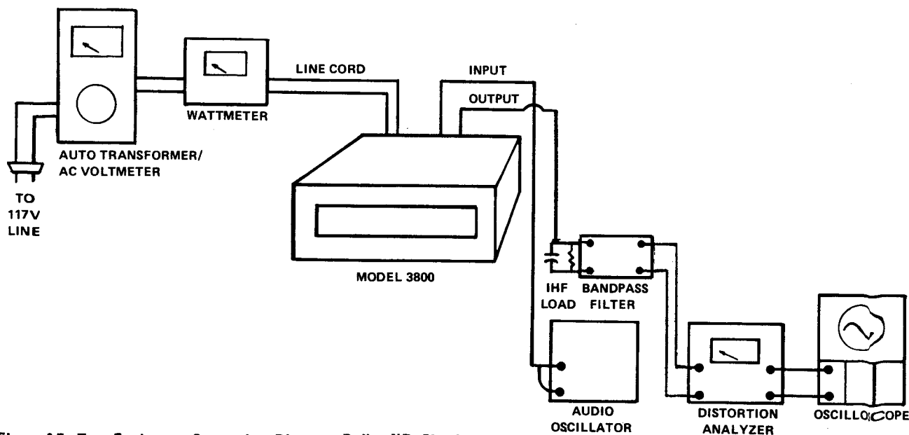
Figure 2-7 Test Equipment Connection Diagram, Dolby NR Circuits
