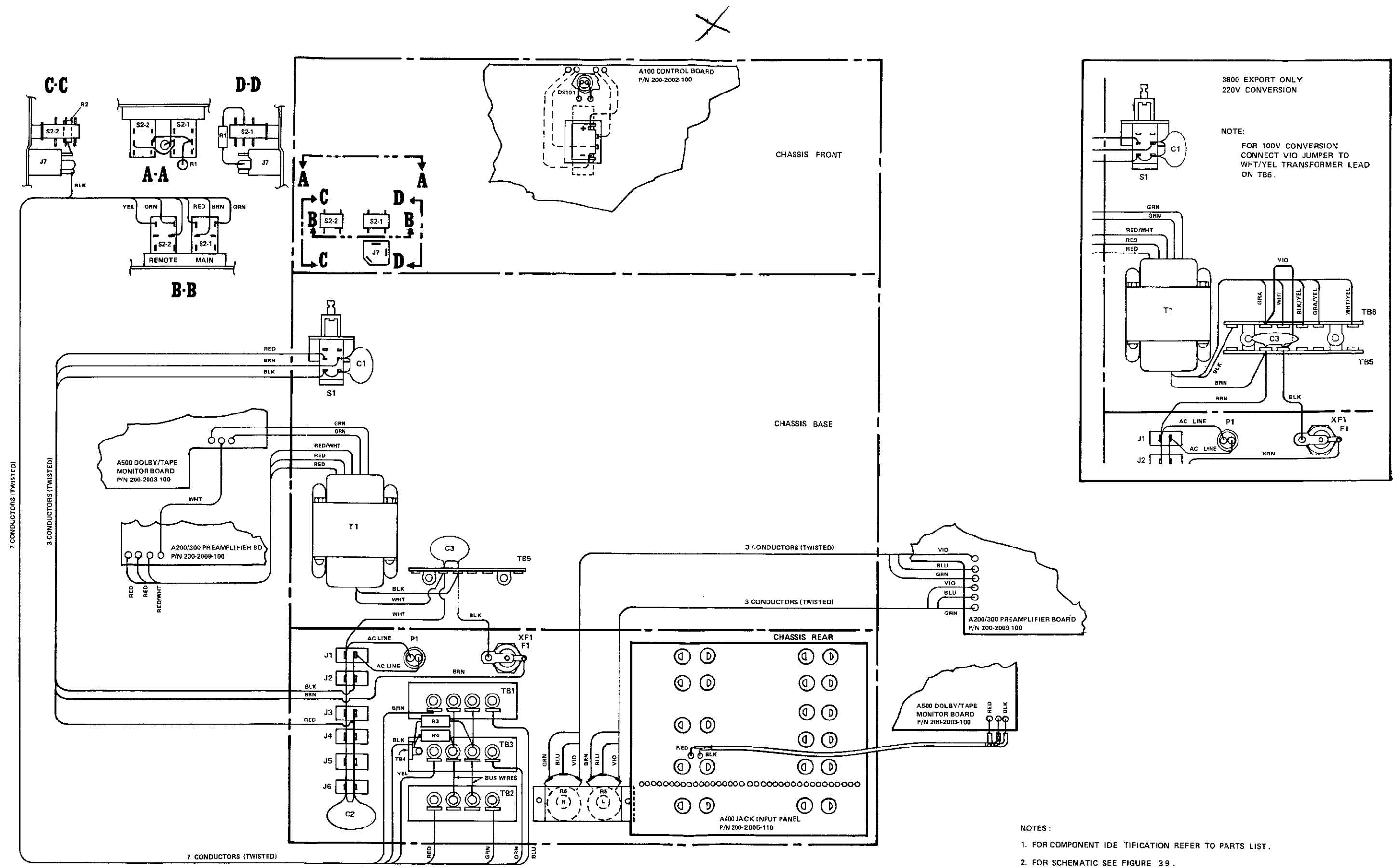
Figure 1-2 Wiring Diagram
