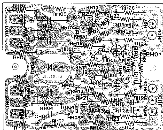
Figure 17. Buffer Amplifier Assembly PH01 Component Locations
