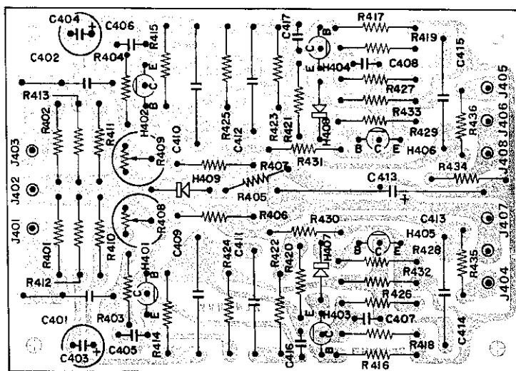
Figure 11. Phono Amplifier Assembly P400 Component Locations
