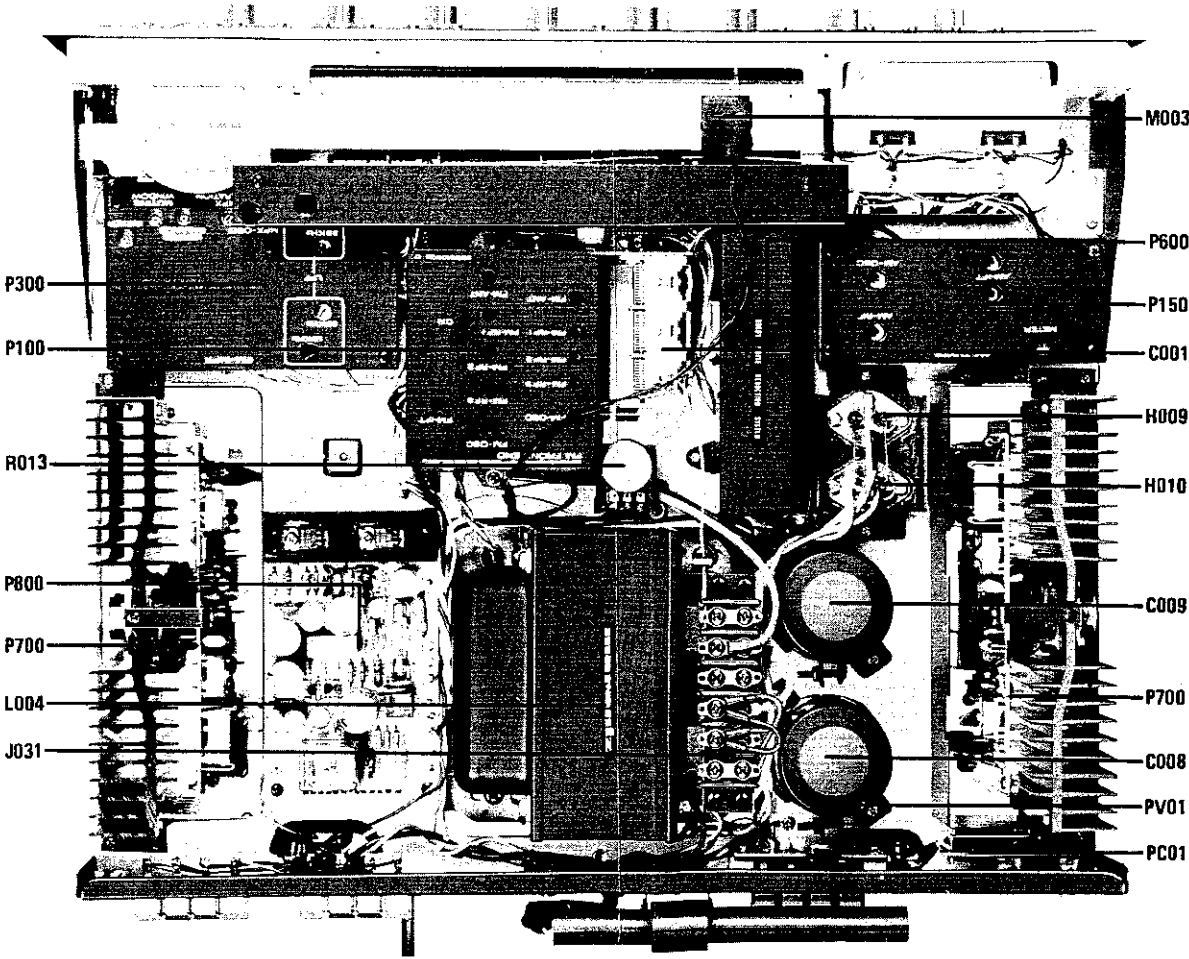
Figure 27. Main Chassis Component Locations (Top View)
