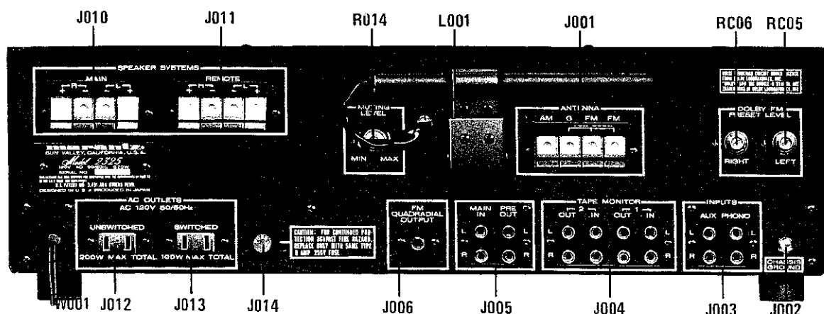
Figure 5. Rear Panel Adjustments and Component Locations
