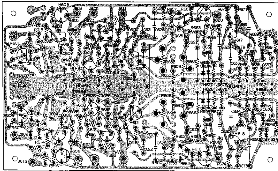
Figure 12. Dolby Unit Assembly P600 Component Locations
