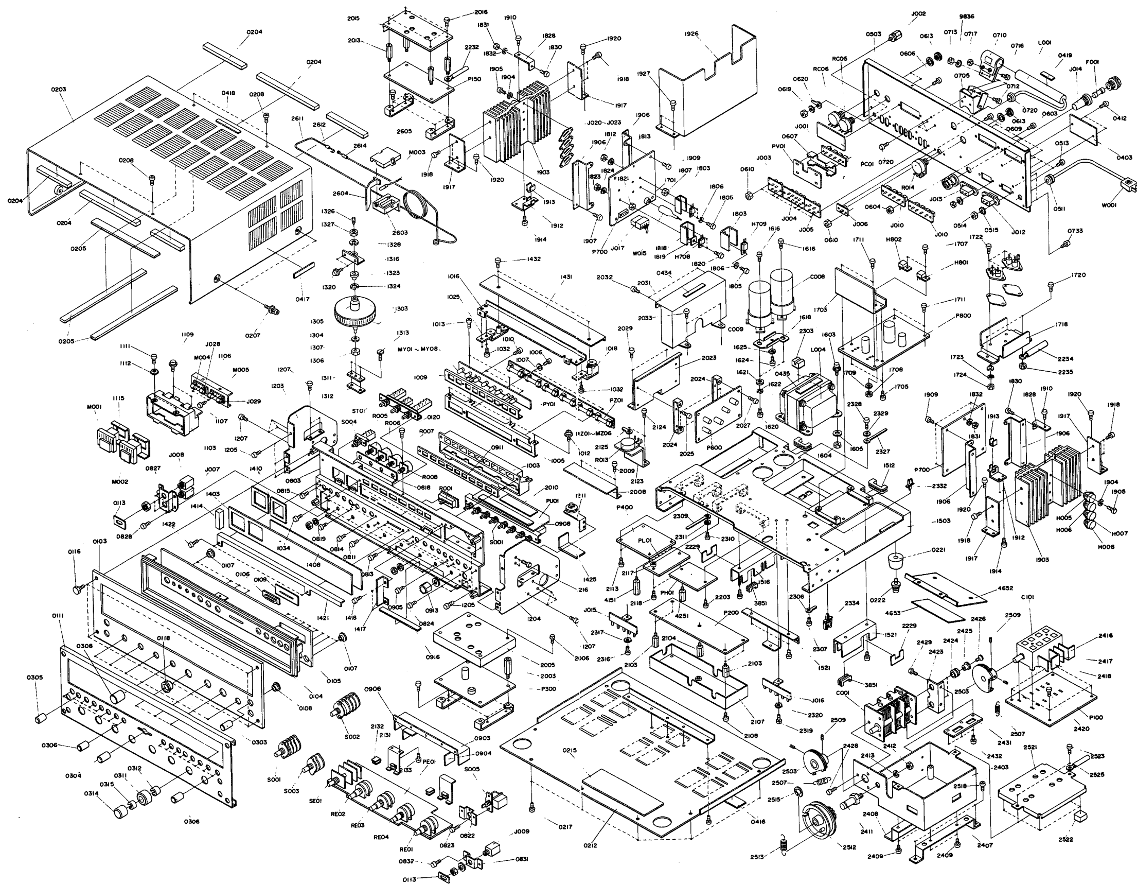
Figure 25. Exploded Mechanical Diagram
