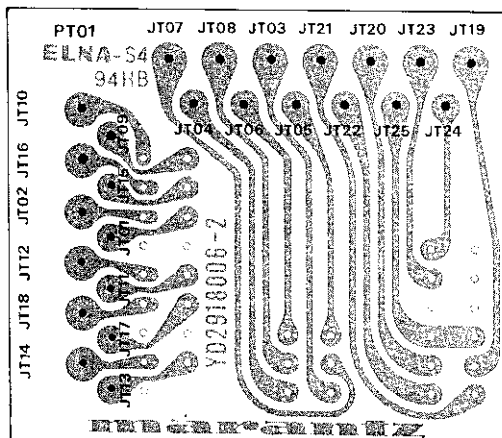
Figure 20. Tape Monitor Assembly PT01 Component Locations
