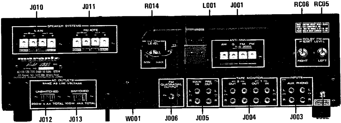
Figure 26. Rear Panel Adjustments and Component Locations
