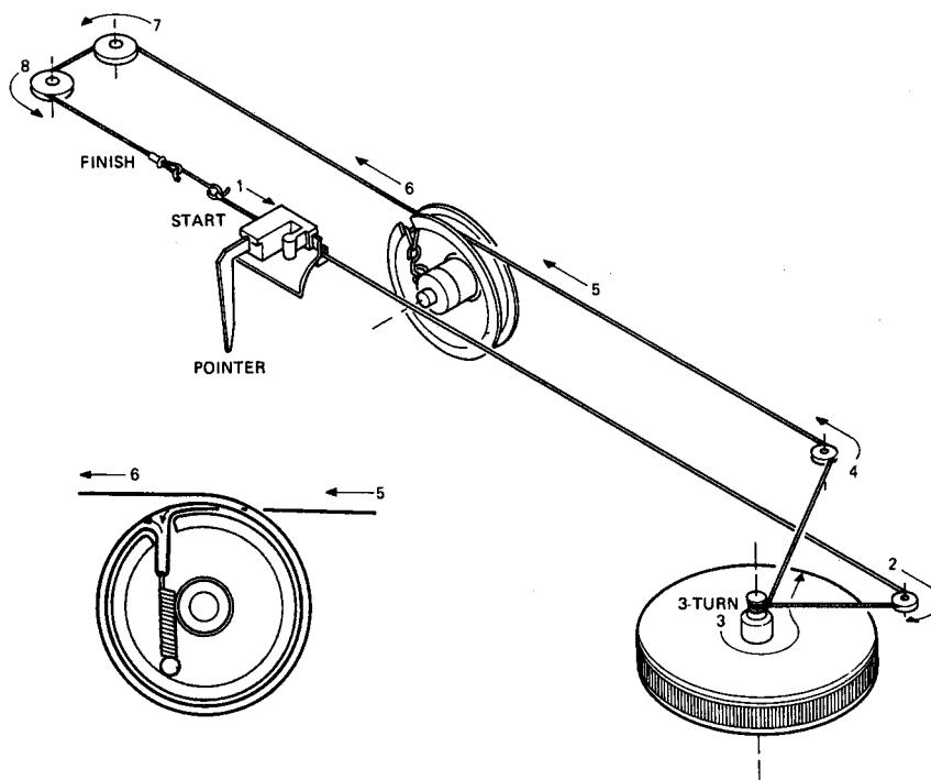
Figure 2. Dial Stringing
