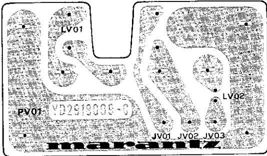
Figure 22. Antenna Terminal Assembly PV01 Component Locations
