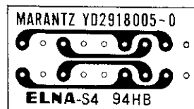
Figure 19. Dolby Tone, Tape Mon. Assembly PS01 Component Locations
