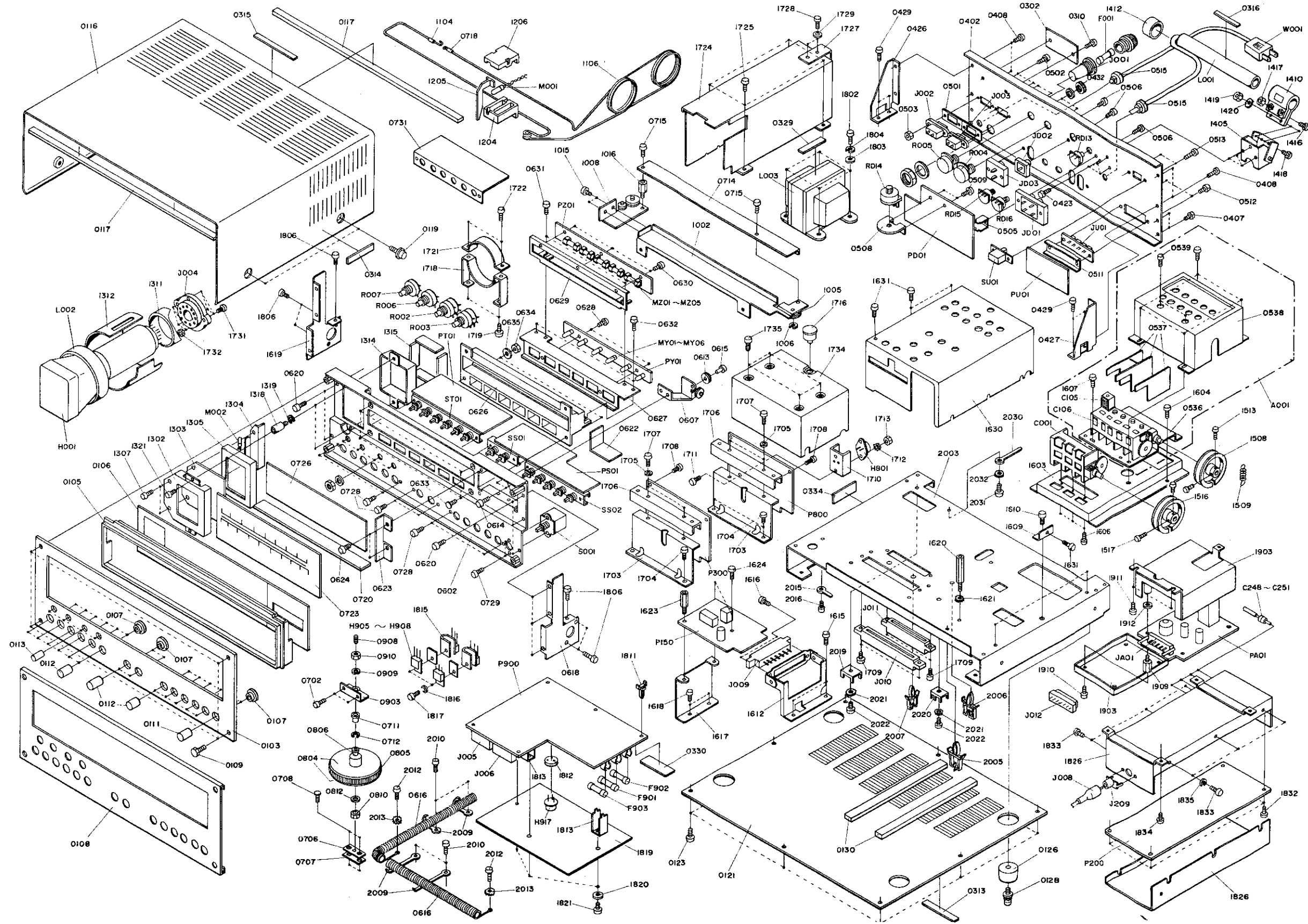
Figure 21. Exploded Mechanical Diagram
