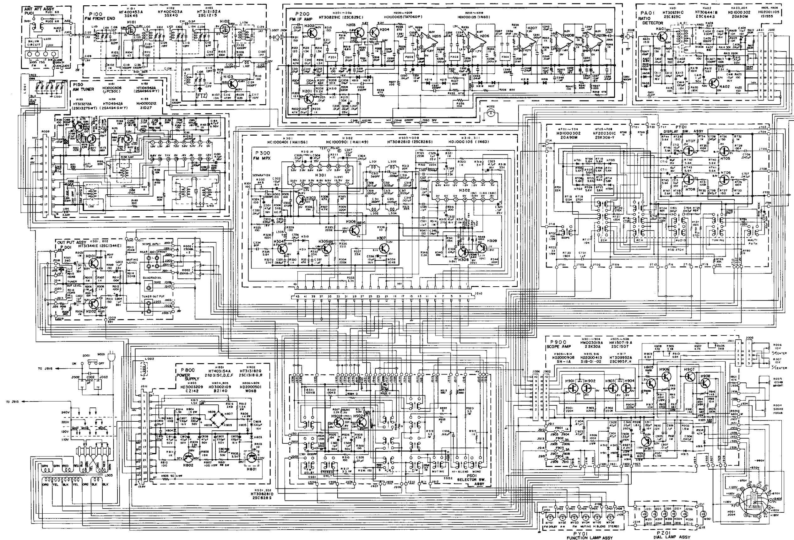
Figure 25. Schematic Diagram
