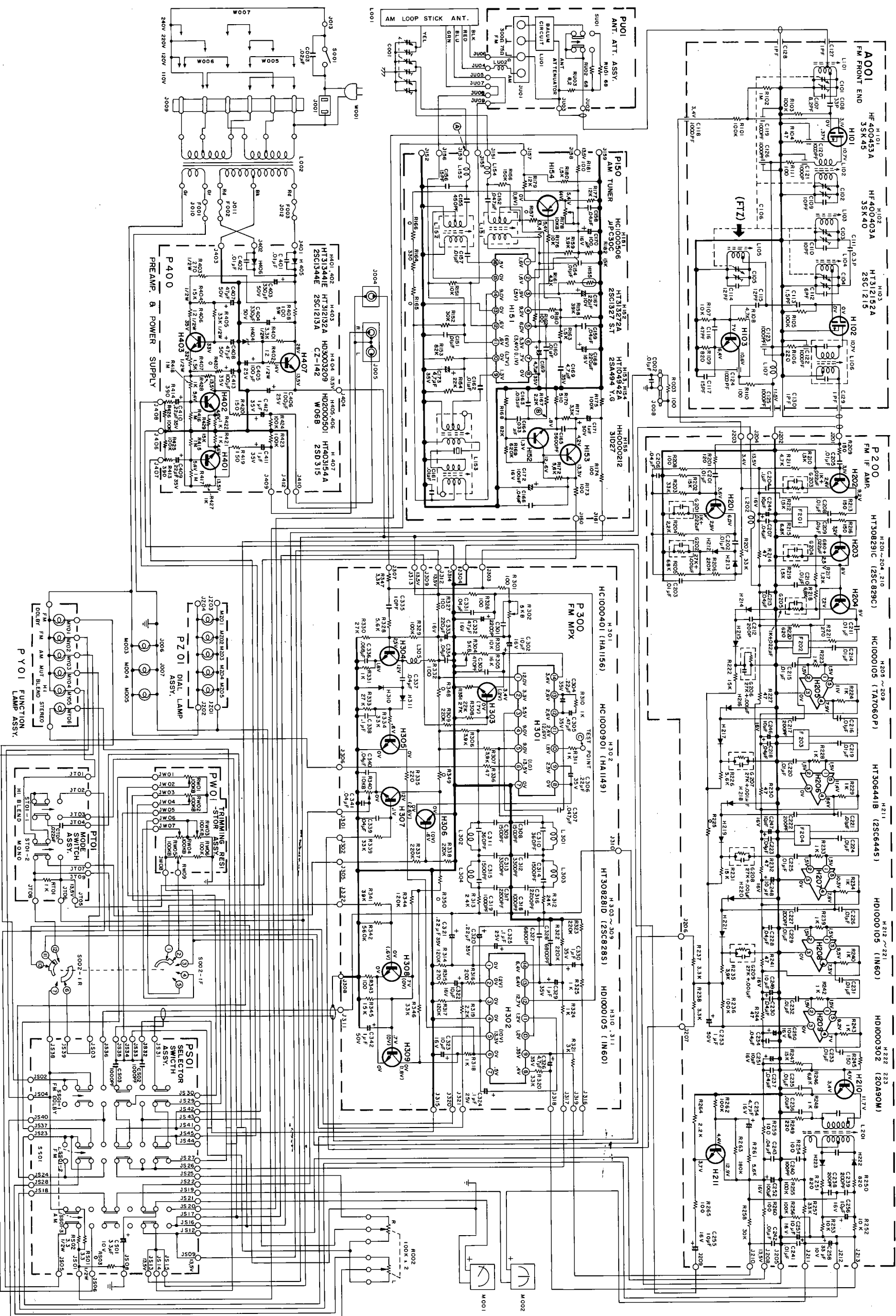
Model 125 NOTE: This schematic diagram applied to units manufactured for the European market.
