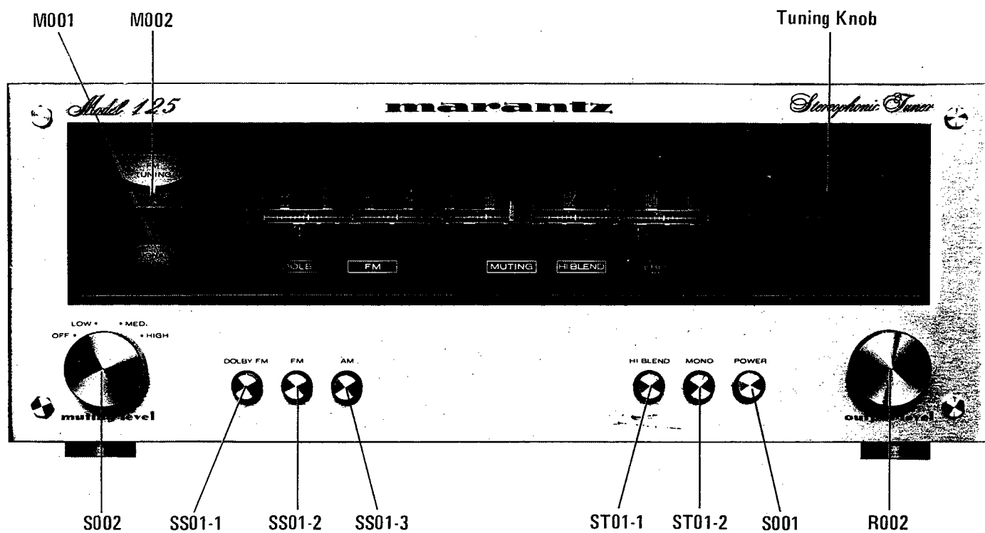
Figure 4. Front Panel Adjustment and Component Locations
