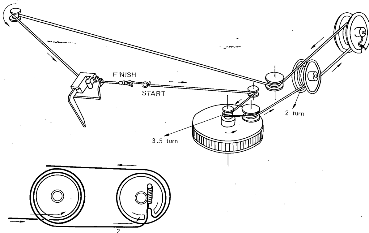
Figure 3. Dial Stringing
