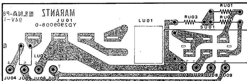
Figure 15. ANT ATT Assembly PV01 Component Locations
