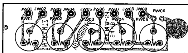
Figure 16. Trimming Resistor Assembly PW01 Component Locations
