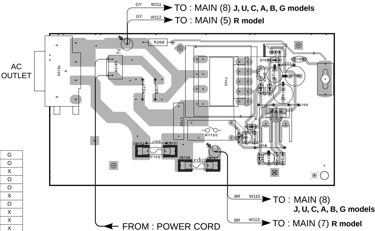
P. C. B. MAIN ( 6 )
