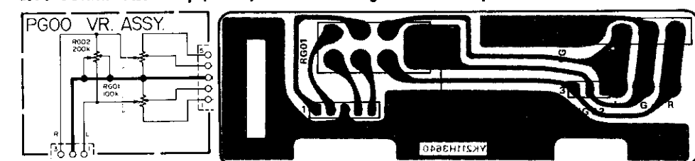
5.11 Volume Assembly (PG00) Schematic Diagram and Component Locations
