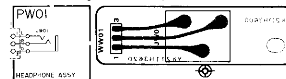
5.8 Head Phone (PW01) Schematic Diagram and Component Locations
