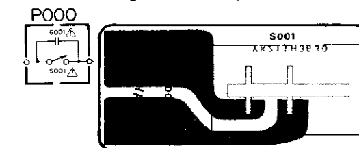
5.10 Power Switch (P000) Schematic Diagram and Component Locations
