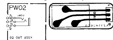
5.9 EQ Out (PW02) Schematic Diagram and Component Locations
