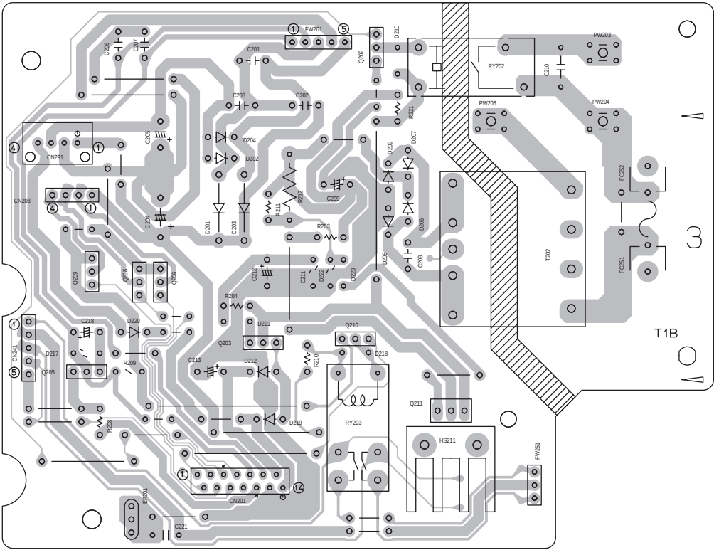
(Power / Fuse board)
