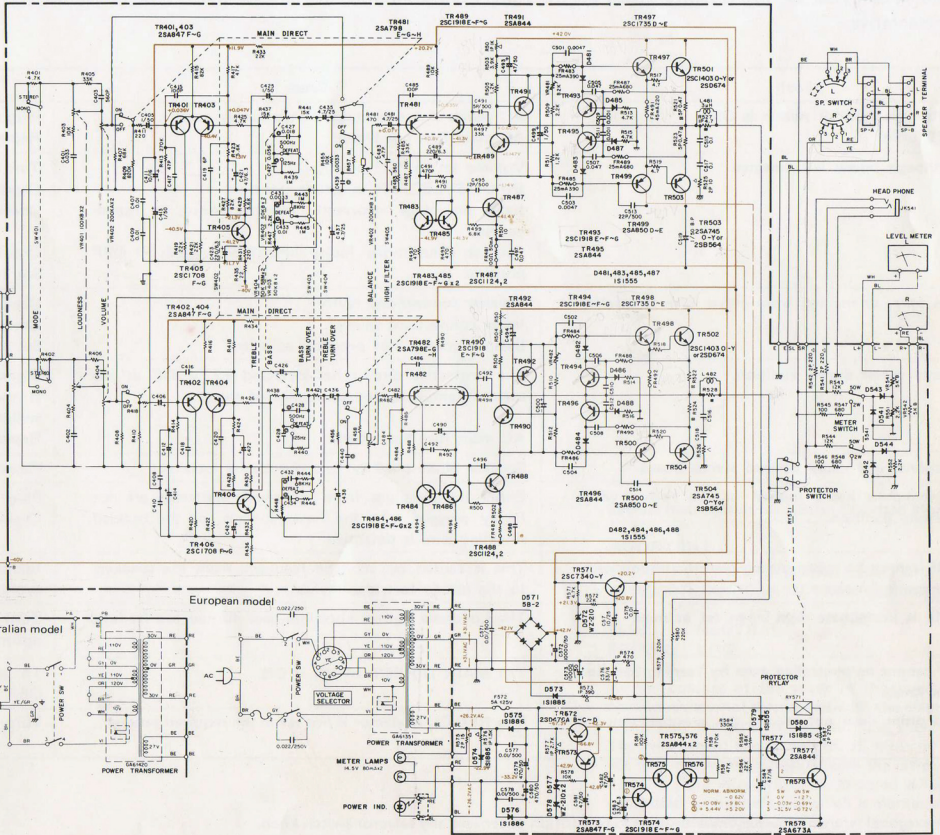
MAIN CIRCUIT BOARD (NA06940)
