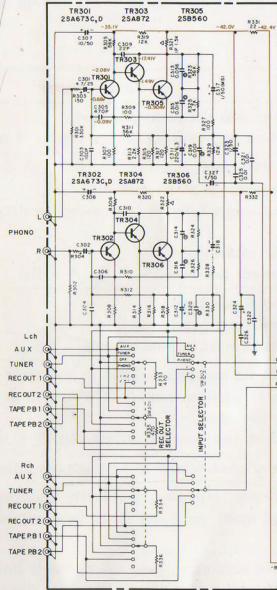
FUNCTION CIRCUIT BOARD (NA06937)
