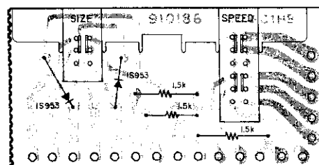
SW PCB (P-7)
