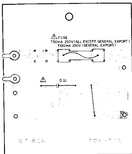
POWER PCB (P-7)
