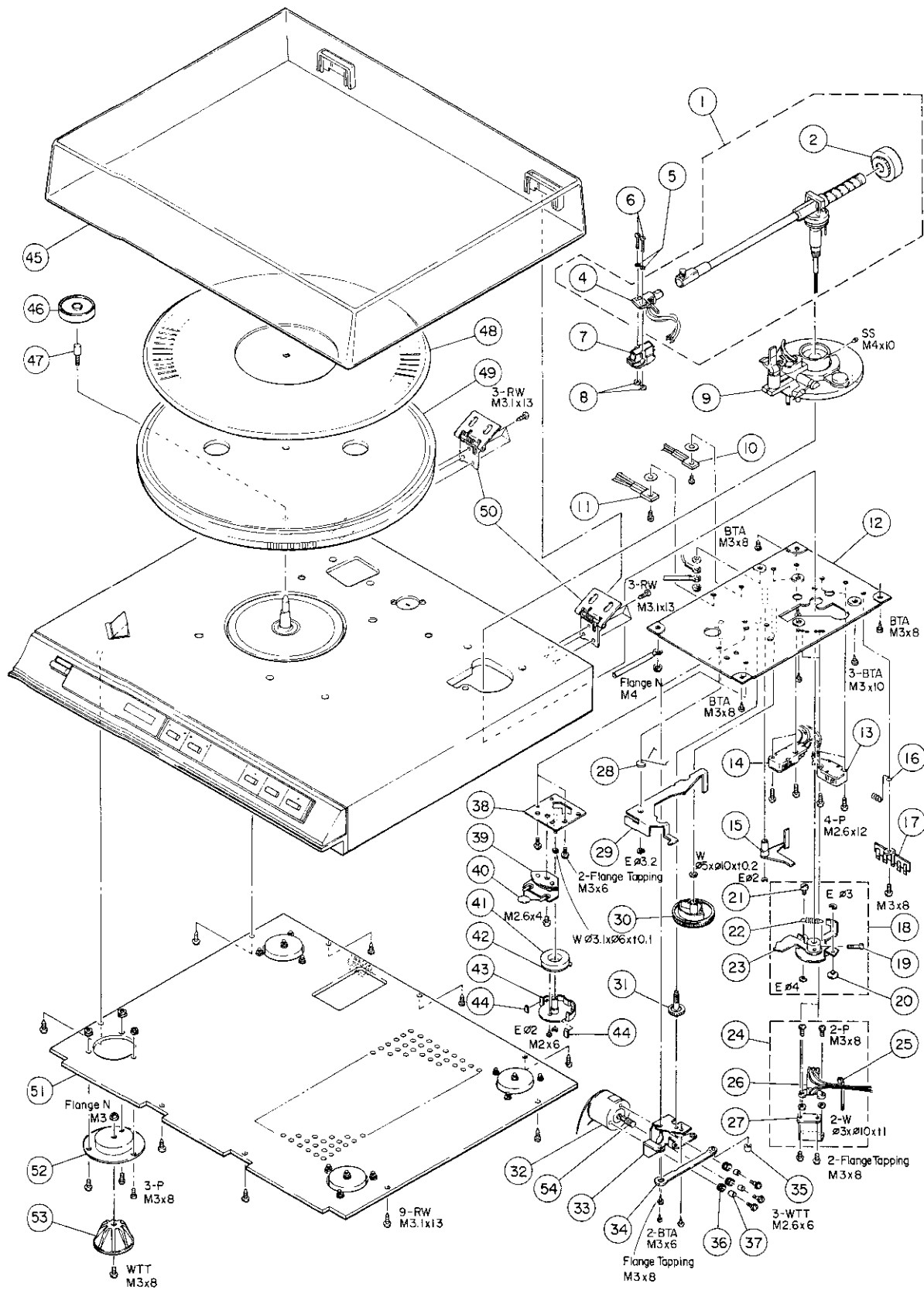
EXPLODED VIEW - 1 (P-9)
