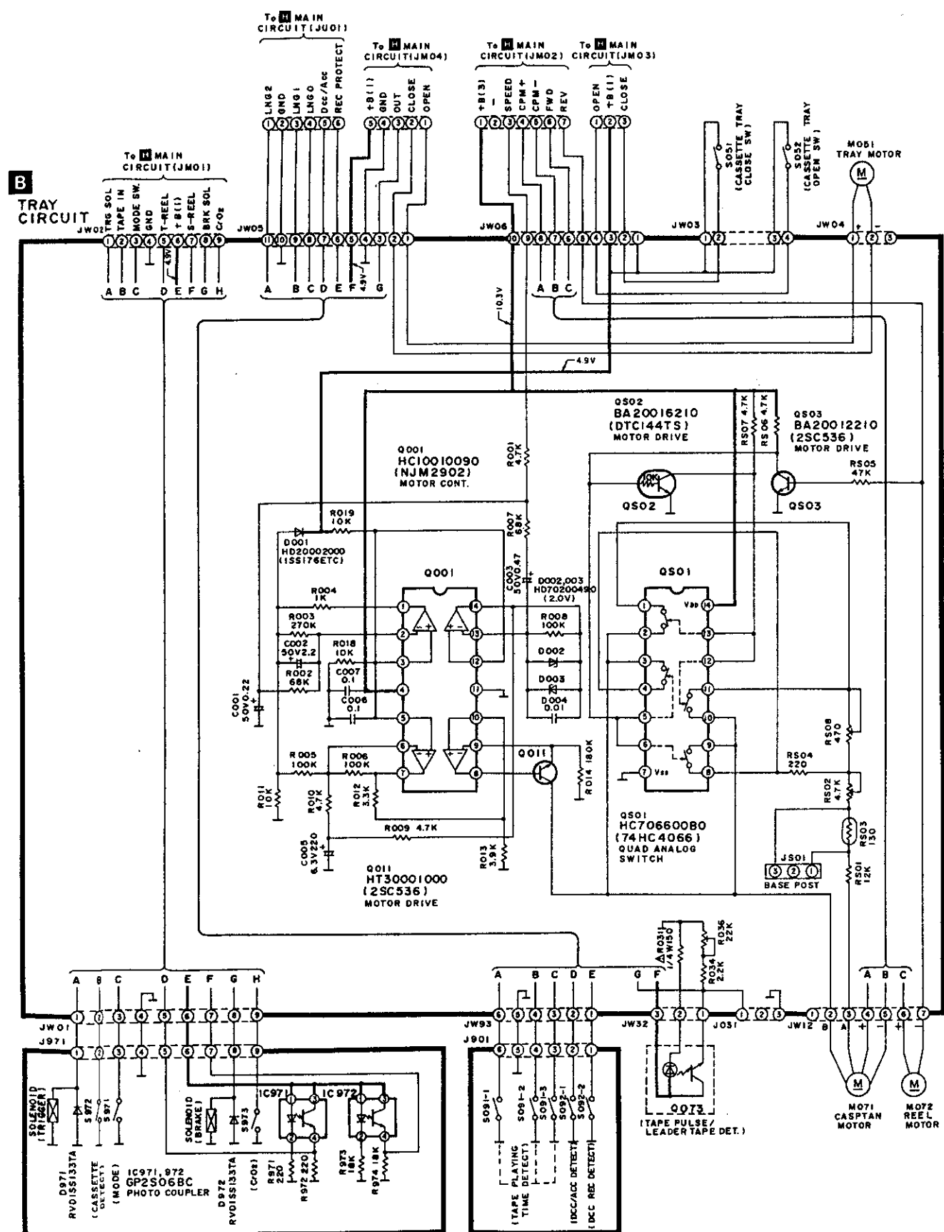
C MECHANISM CIRCUIT
