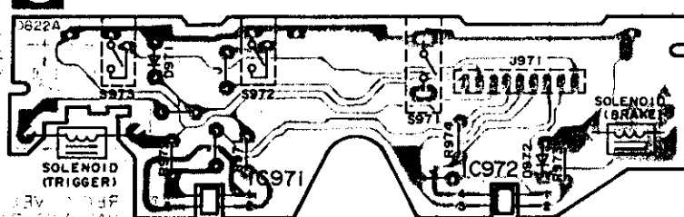
C MECHANISM P.C.B. (REP1406)
