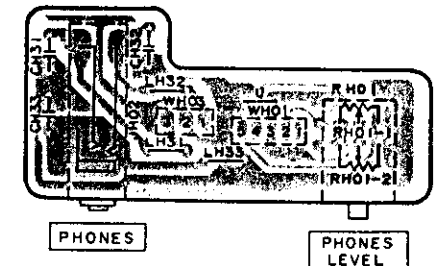
M HEADPHONES LEVEL P.C.B. (ZZ01102330)
