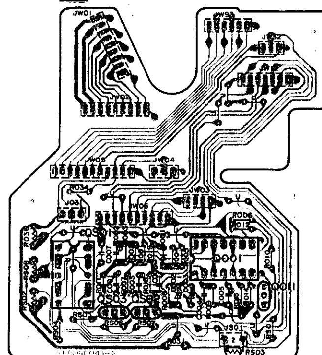
B CONNECTION P.C.B. (ZZ01100410)
