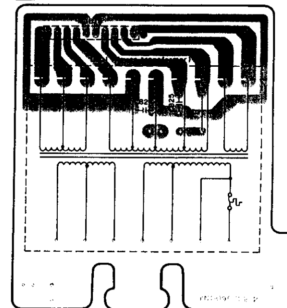
K POWER TRANSFORMER P.C.B. (ZZ01108210)
