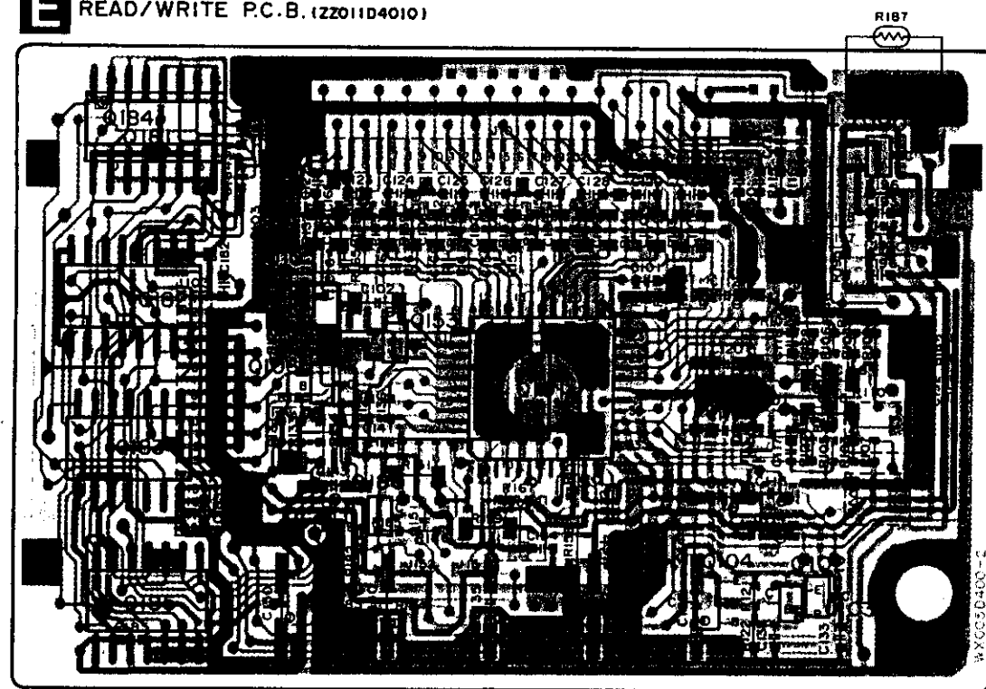
E READ/WRITE P.C.B. (ZZ01104010)
