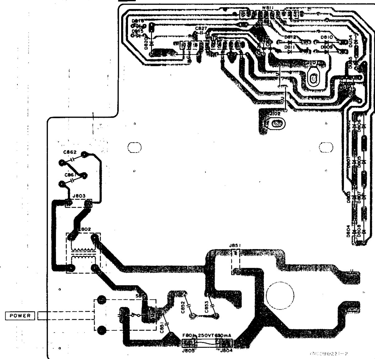
J POWER SUPPLY P.C.B. (ZZ01108210)
