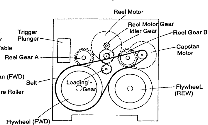
Backside View of Mechanism
