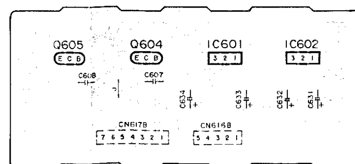
K REGULATOR P.C.B. (REPI888A-T)
