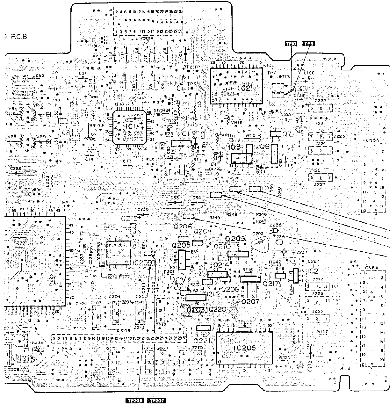
K REGULATOR P.C.B. (REPI688A-T)
