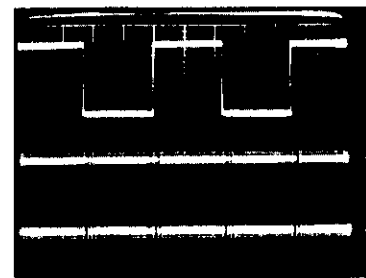
PLAY/BACK WITH MUSIC SIGNAL Y : 0.2V × 10 X : 5μs
