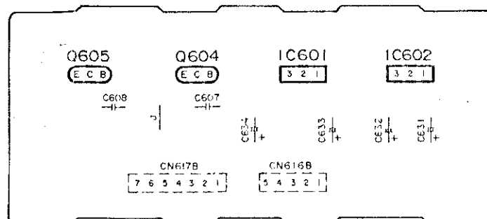
K REGULATOR P.C.B. (REPI688A-T)
