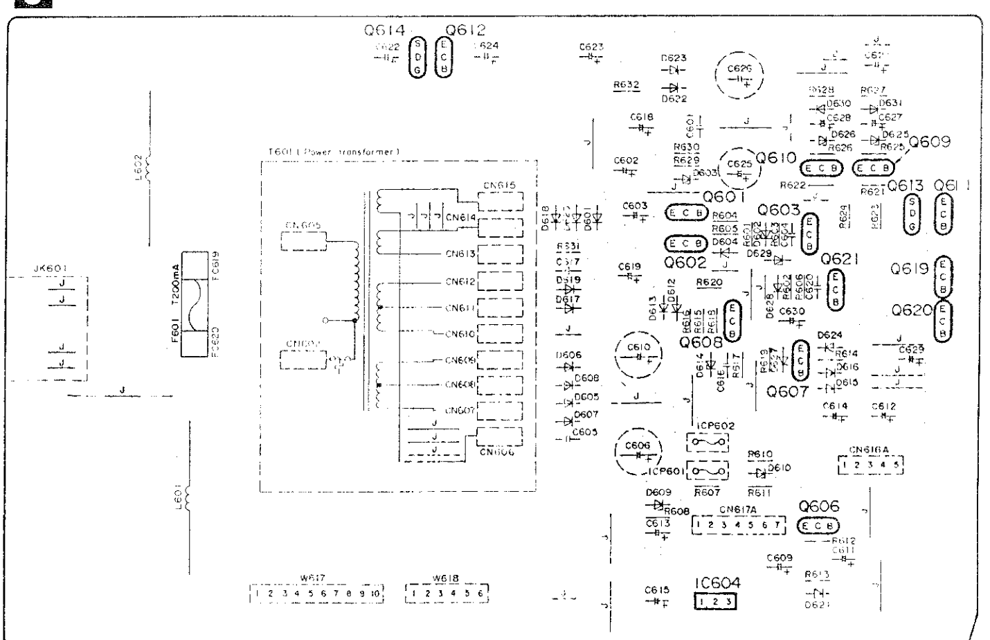
J POWER SUPPLY P.C.B. (REPI721D-P)
