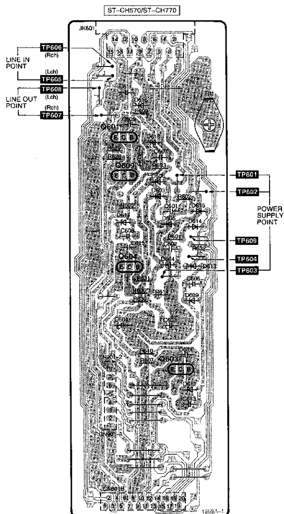
D POWER SUPPLY P.C.B. (REP2367A-P)
