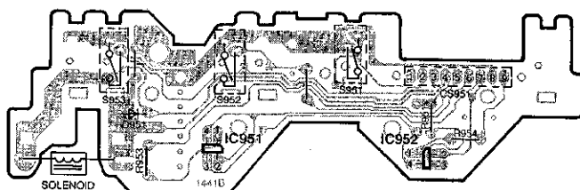
C MECHANISM P.C.B. (DECK2) (REP2131D)
