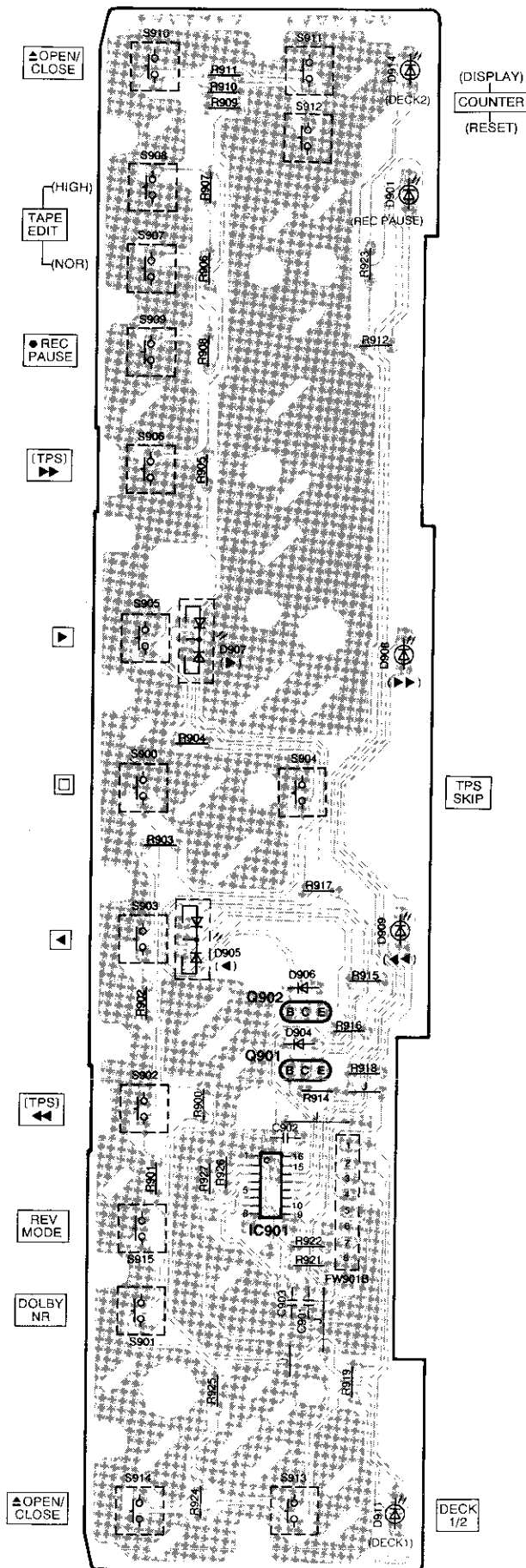
D OPERATION P.C.B. (REP2142A-M)
