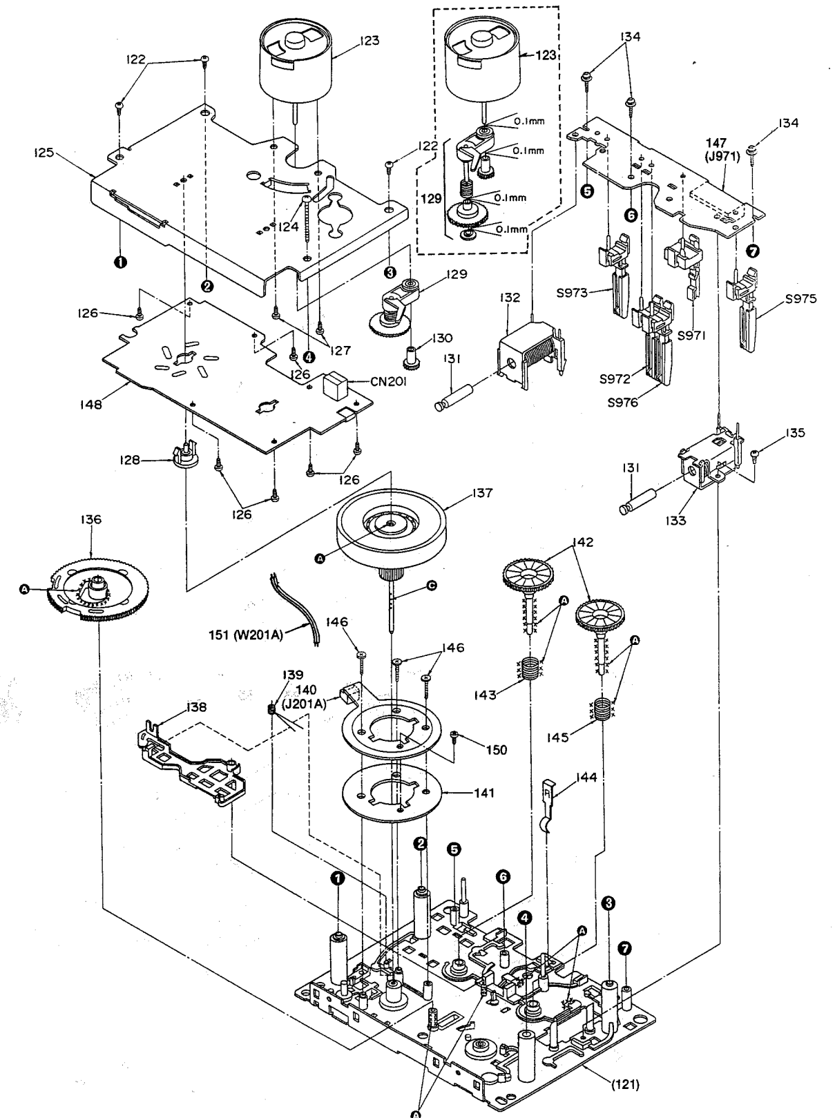
(Bottom view)
