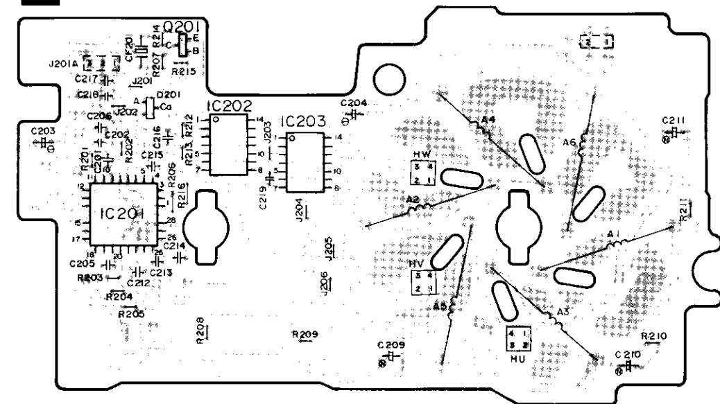
1 CAPSTAN MOTOR (D.D) P.C.B.
