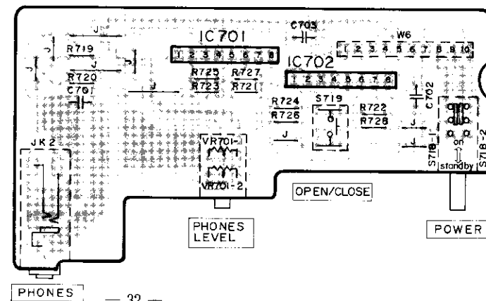
H POWER SWITCH/HEADPHONES P.C.B.
