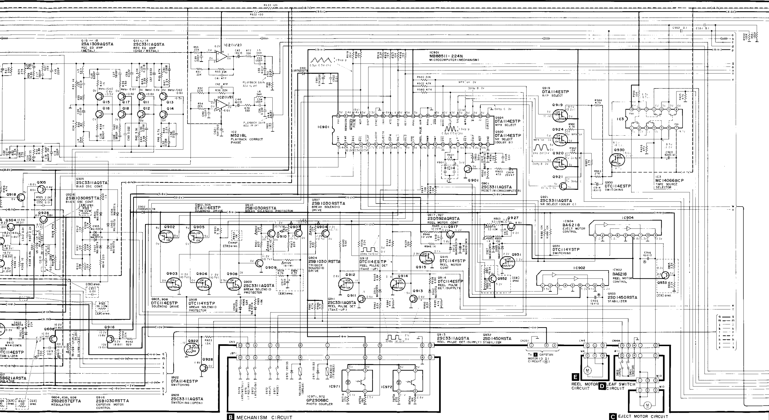
B MECHANISM CIRCUIT
