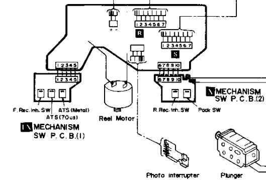
MECHANISM P.C.B.
