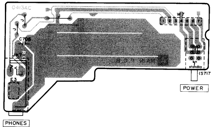
E POWER SWITCH/HEADPHONES P.C.B.
